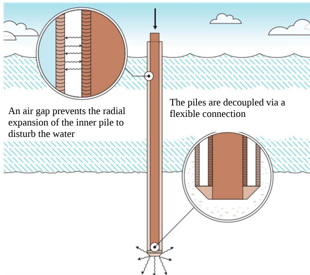
Figure 5: Schematic of the double wall pile
