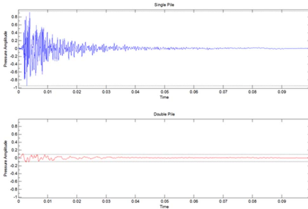
Figure 9: p(t) plots comparing a single wall pile (top) and a double wall pile (bottom)
