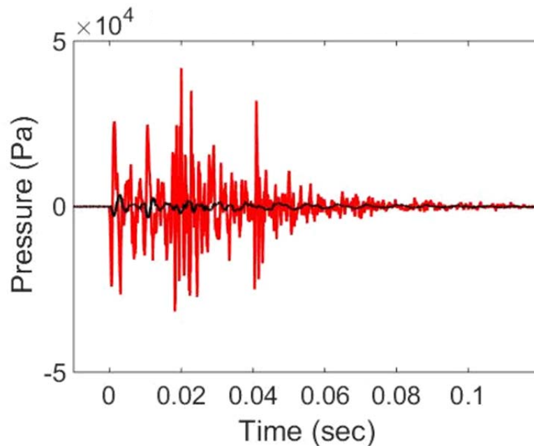
Figure 28: A typical pressure recording after a hammer strike measured at an 8-m distance from the control pile (red) and the double pile (black).
