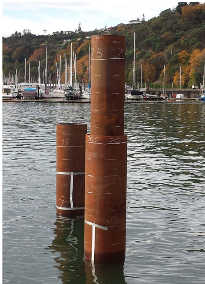
Figure 27: Control pile and double pile after driving
