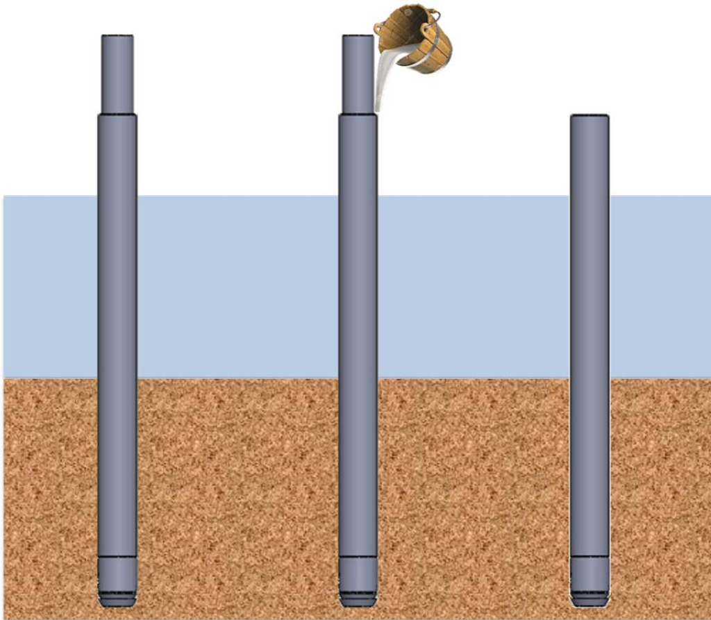
Figure 13: Double pile (left), filled double pile (center), mandrel double pile (right)
