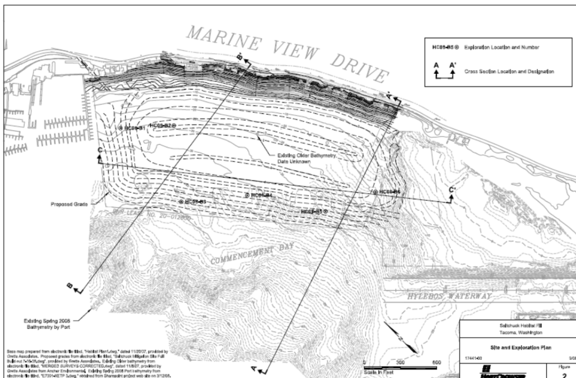
Figure 21: Bathymetry at the test site.
