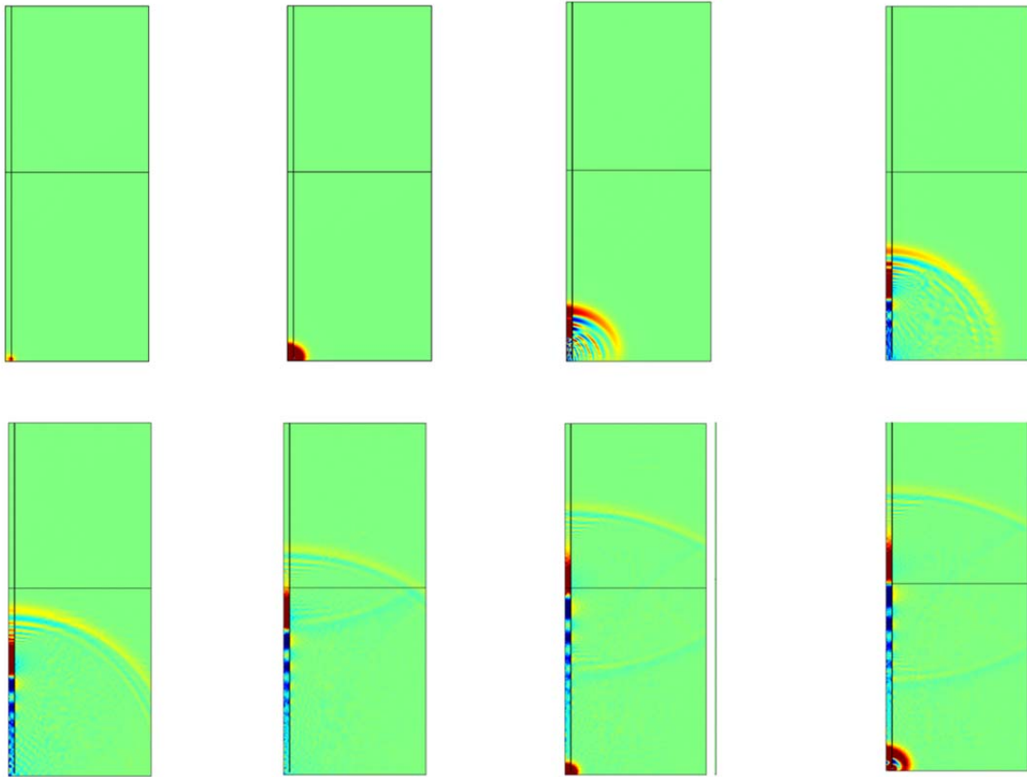
Figure 6: Initial double pile finite element modelling
