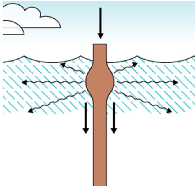
Figure 2: Illustration of the radial displacement wave after a hammer strike.
