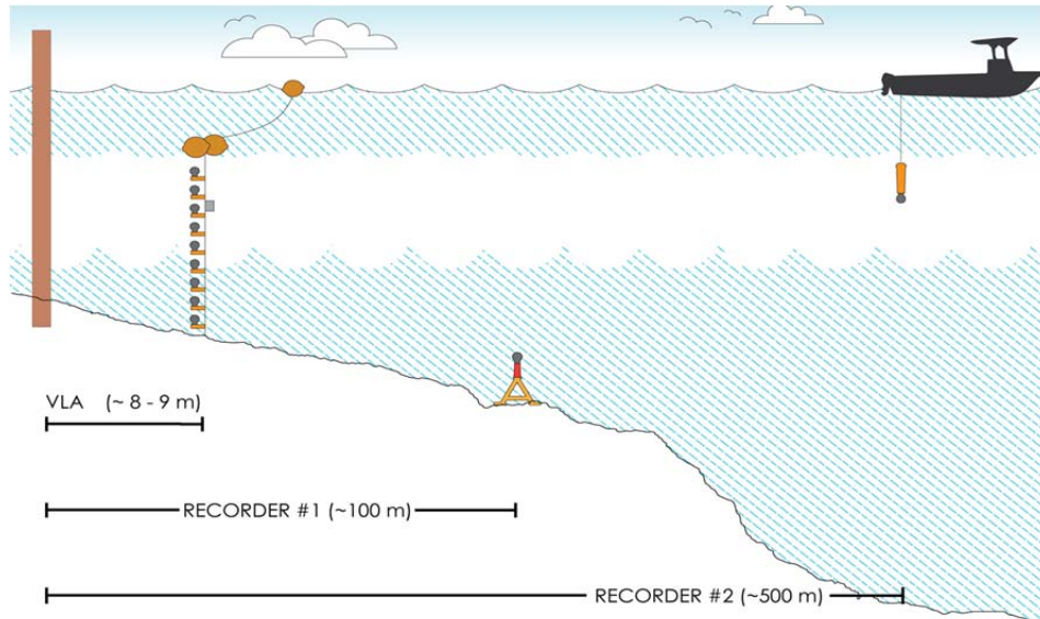
Figure 22: Locations of the hydrophones
