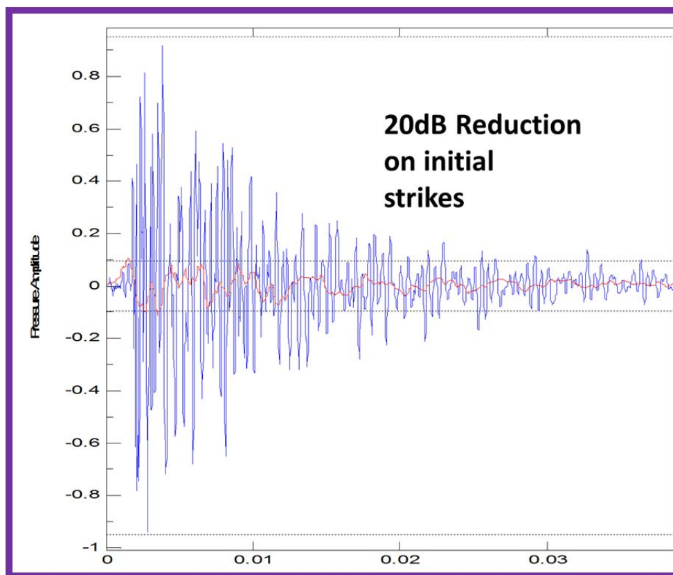
Figure 10: p(t) pile signals overlaid and magnified
