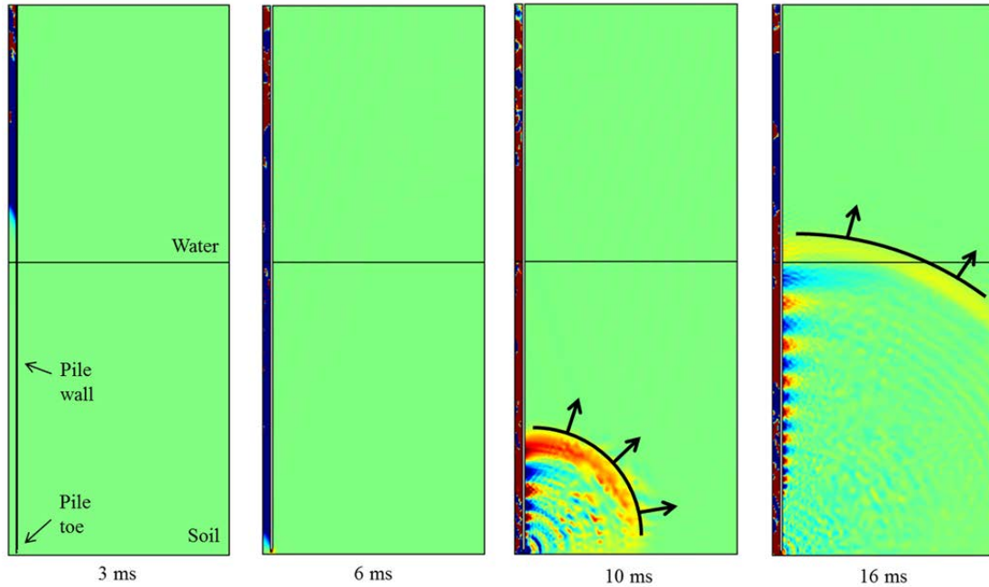
Figure 7: Finite element modelling of the 6-inch double pile
