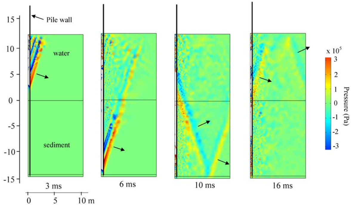
Figure 3: Acoustic pressure surface plots showing the acoustic radiation from the pile after 3, 6, 10, and 16 ms after impact by a pile hammer.
