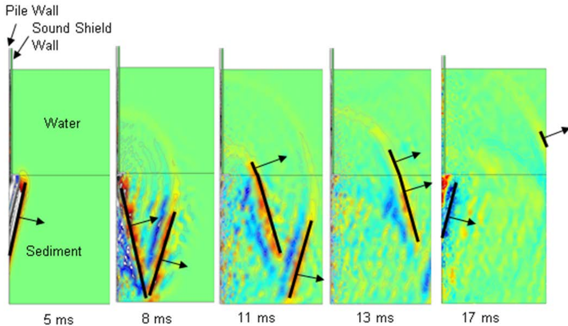
Figure 4: Acoustic pressure surface plots showing the acoustic radiation from the pile with the acoustic shield at 5, 8, 11, 13 and 17 ms after impact by a pile hammer.
