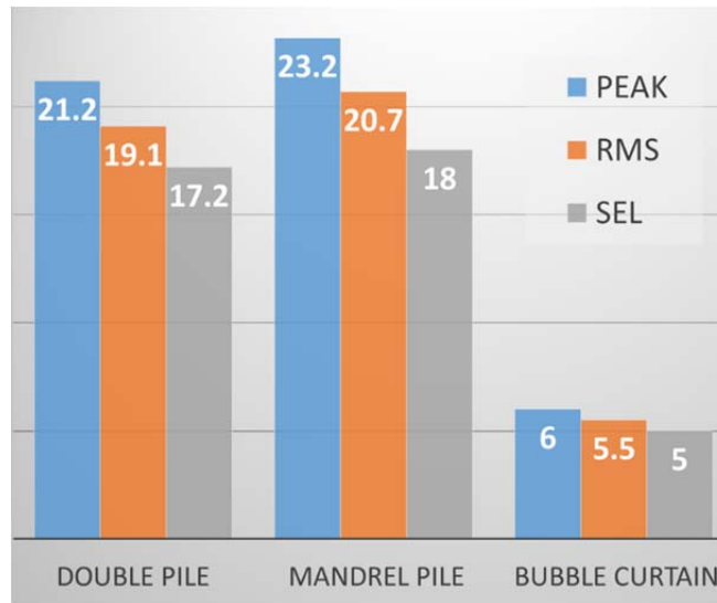
Figure 29: Summary of the results of the acoustic measurements in dB
