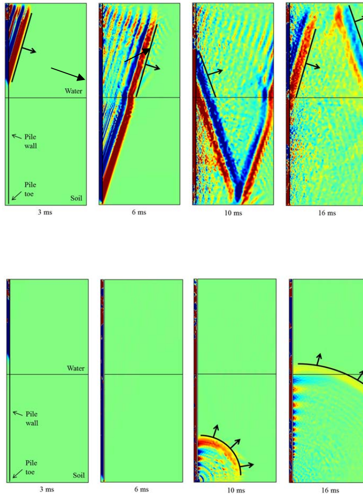
Figure 12: Acoustic pressure surface plots showing the acoustic radiation from the single pile (top) and the double pile (bottom) at 3 ms, 6 ms, 10 ms, and 16 ms after impact by a pile hammer.
