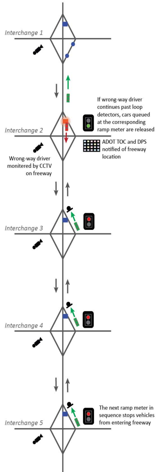
Figure 20. Suggested Plan for Pilot Deployment
