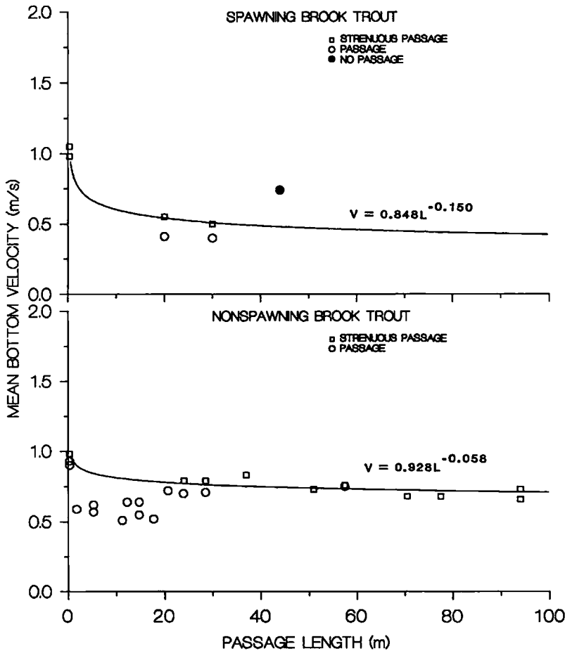
FIGURE 3.—Combinations of mean bottom water velocity ( V ) and passage length ( L ) that spawning and non-spawning brook trout did and did not pass through. The nonlinear regression lines are fits to the strenuous passage combinations indicated by the open squares. Each passage symbol indicates at least one fish successfully completed passage.
