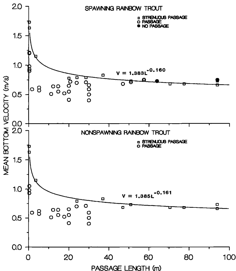
FIGURE 1.—Combinations of mean bottom water velocity ( V ) and passage length ( L ) that spawning and nonspawning rainbow trout did and did not pass through. The nonlinear regression lines are fits to the strenuous passage combinations indicated by the open squares. Each passage symbol indicates at least one fish successfully completed passage.
