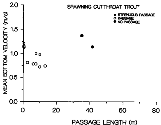
FIGURE 4.—Combinations of mean bottom water velocity and passage length that spawning cutthroat trout did and did not pass through. Each passage symbol indicates at least one fish successfully completed passage.
