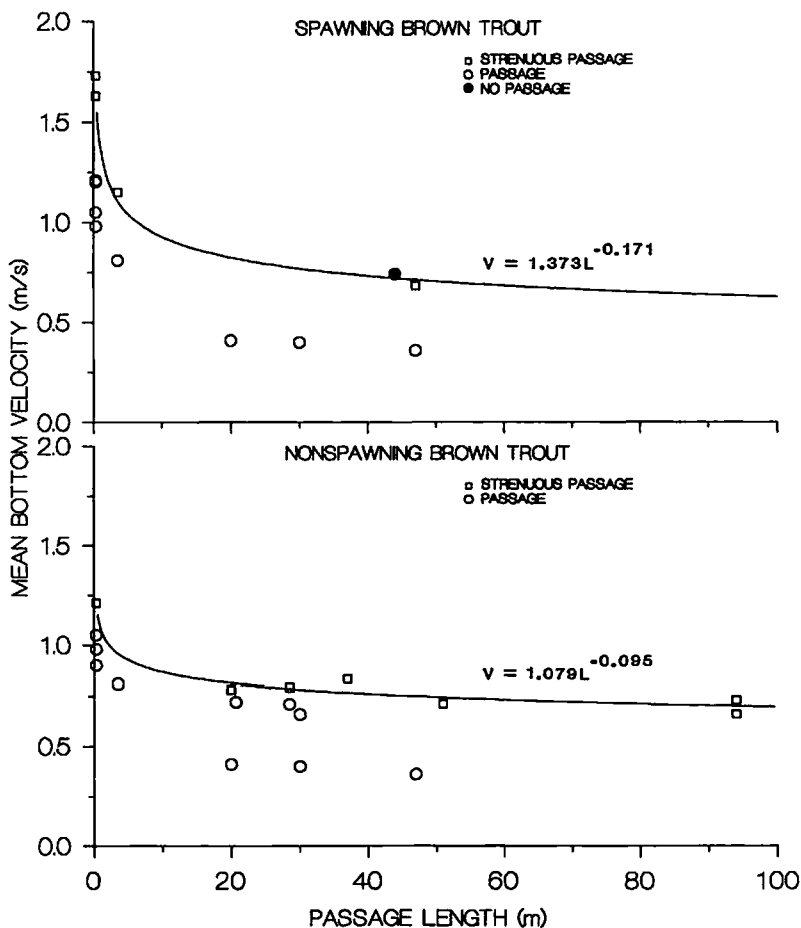
FIGURE 2.—Combinations of mean bottom water velocity ( V ) and passage length ( L ) that spawning and non-spawning brown trout did and did not pass through. The nonlinear regression lines are fits to the strenuous passage combinations indicated by the open squares. Each passage symbol indicates at least one fish successfully completed passage.
