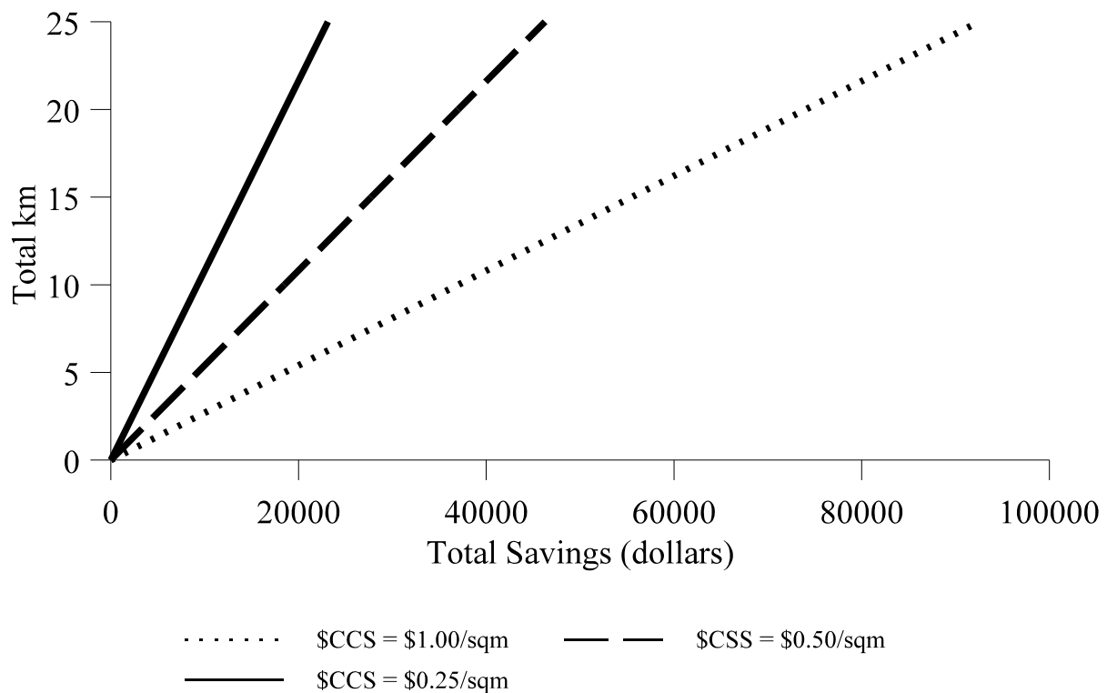
Figure 6-1. Initial construction cost savings.
