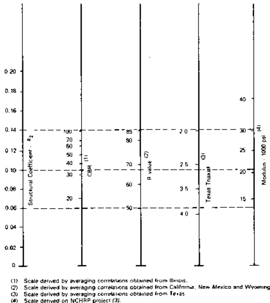
Figure E-5. Correlation between base aggregate structural layer coefficient, a_2 , and CBR, R-value, Texas-triaxial, and resilient modulus (AASHTO, 1993).
