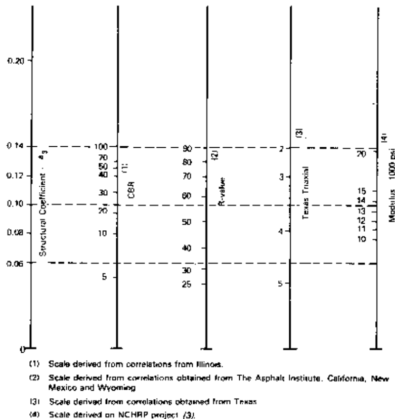
Figure E-6. Correlation between subbase aggregate structural layer coefficient, a_3 , and CBR, R-value, Texas-triaxial, and resilient modulus (AASHTO, 1993).
