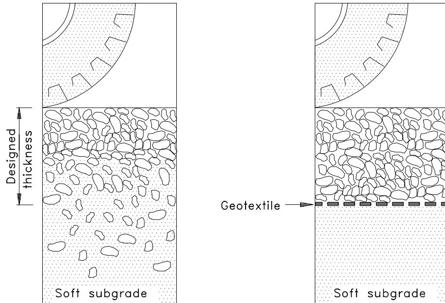
Figure A-1. Concept of geotextile separation in roadways (after Rankilior, 1981).
