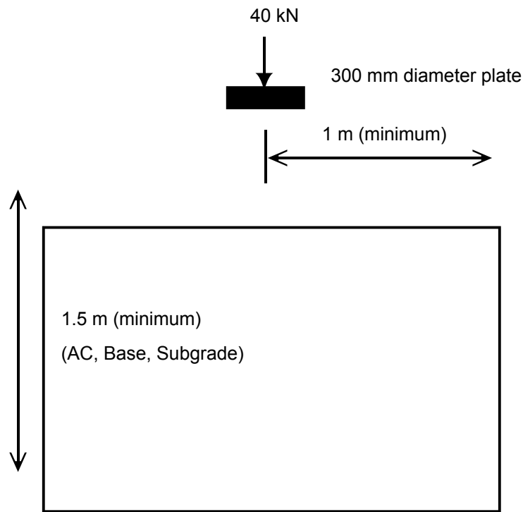
Figure E-1. Minimum box dimensions, plate load and plate dimensions for a test-box pavement test facility.
