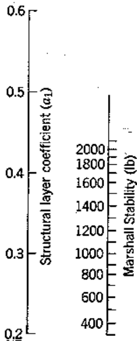
Figure E-3. Correlation between asphalt concrete structural layer coefficient, a_1 , and Marshall stability (after Van Til et al., 1972).
