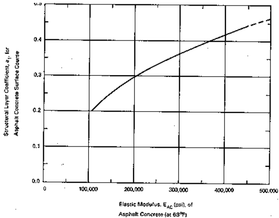
Figure E-4. Correlation between asphalt concrete structural layer coefficient, a_1 , and elastic (resilient) modulus (AASHTO, 1993).
