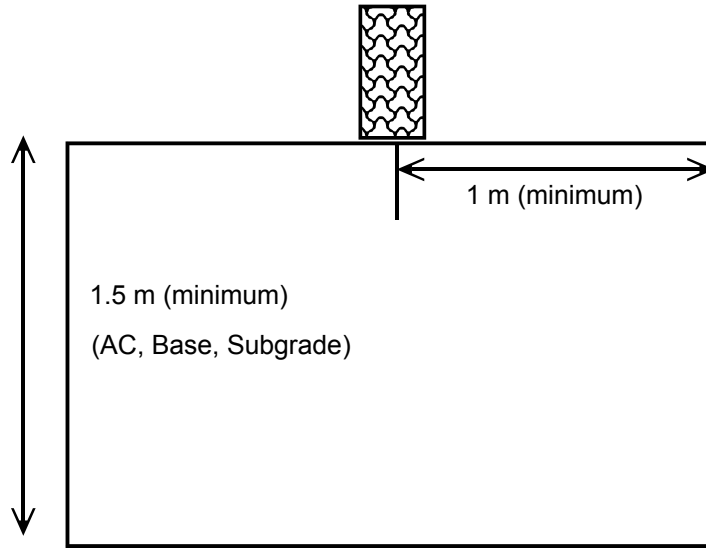
Figure E-2. Minimum dimensions for a test-track pavement test facility.
