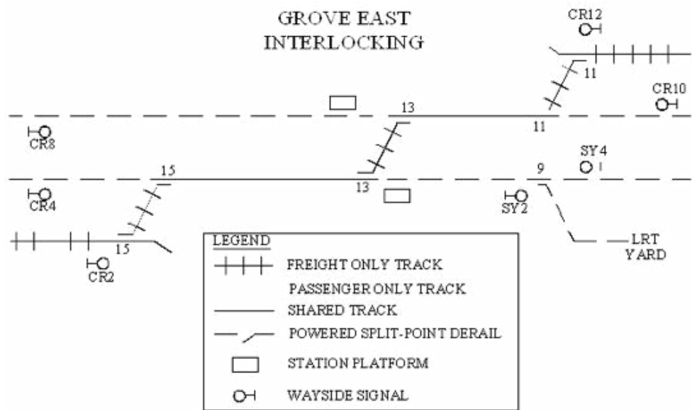
Figure B-6 SITS at Grove East interlocking
