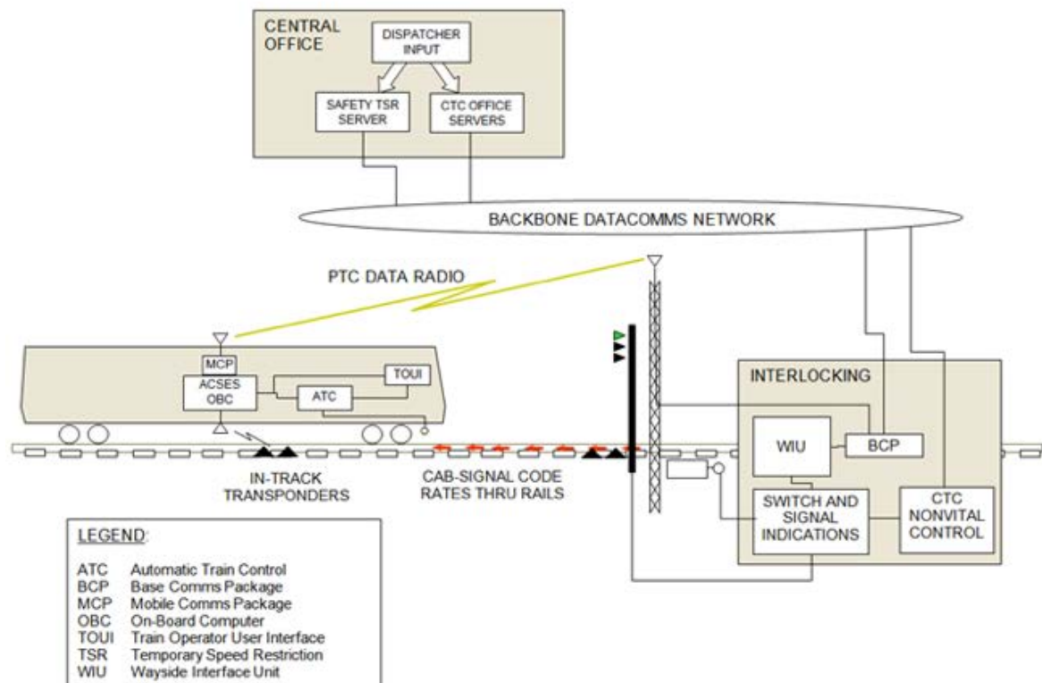
Figure 3-4 ACSES block diagram
