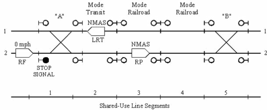
Figure D-9 RF train held to allow LRT to clear A-B at maximum speed
