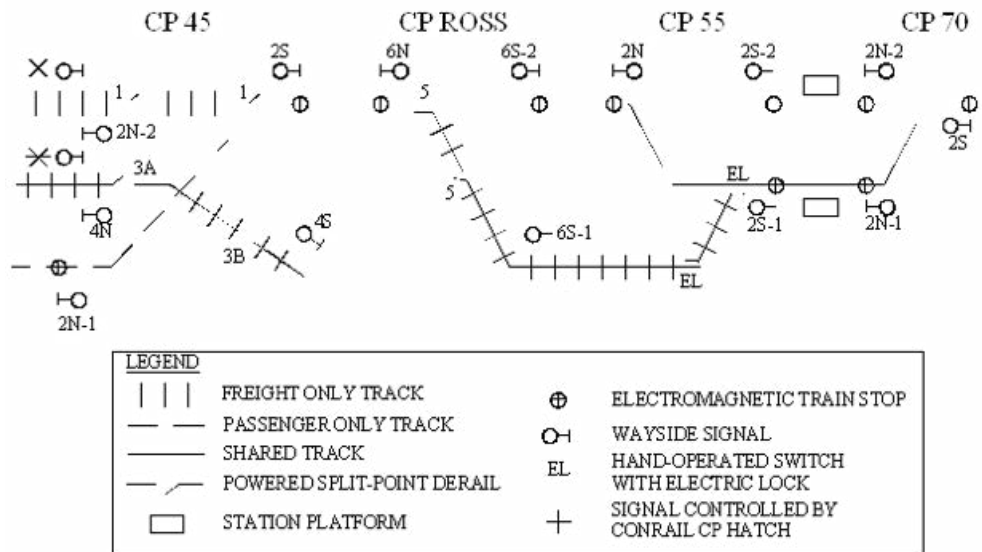
Figure B-4 ETS implementation at and between River LINE CP 45 and CP Ross interlockings
