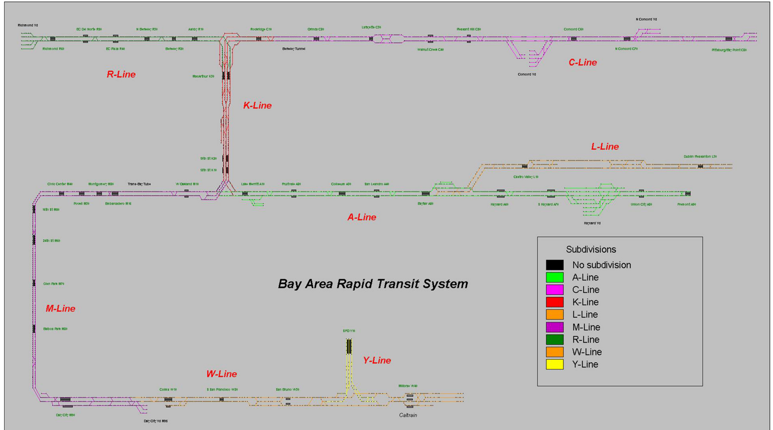
Figure 6-4 Areas of BART system for detailed capacity analysis in RTC model
