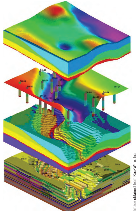
Figure 3-5. Geotechnical 3D model showing above-ground surface and geological layers.
