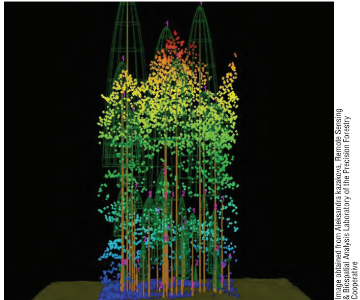
Figure 2-19. Aerial LiDAR is limited by its line of sight. When aerial LiDAR flies over a tree canopy, the user must filter out the points on the vegetation and use only those points that reached the ground surface.
