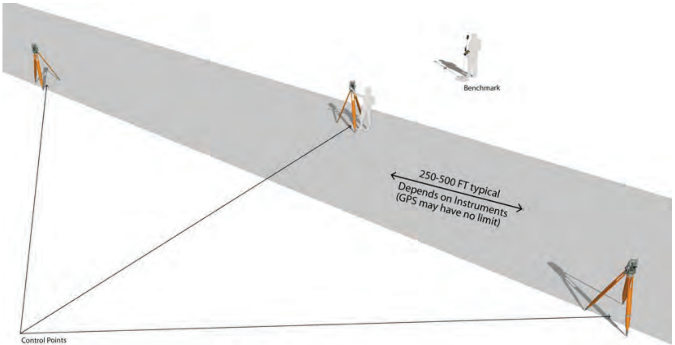
Figure 4-19. Survey control points on a typical stringless paving project.
