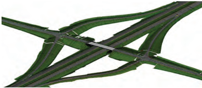
Figure 3-6. How a flyover appears to the designer on the I-35 and IA92 interchange.
