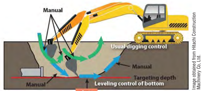
Figure 4-16. AMG excavators use the 3D engineered model for trench depths and alignment.
