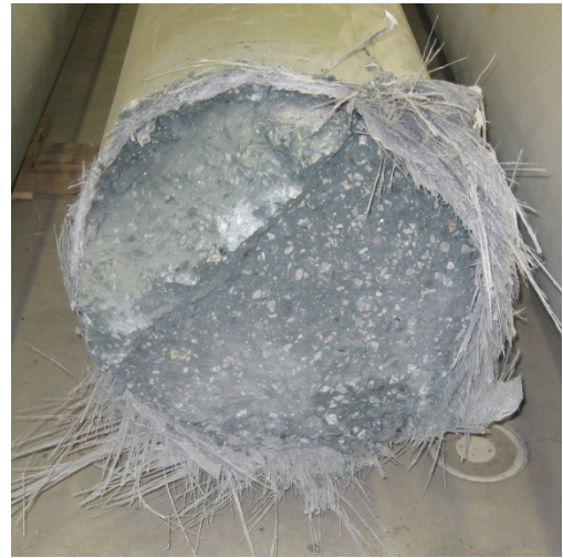
Figure 26: Cut at Failure of Pile A-4FB
