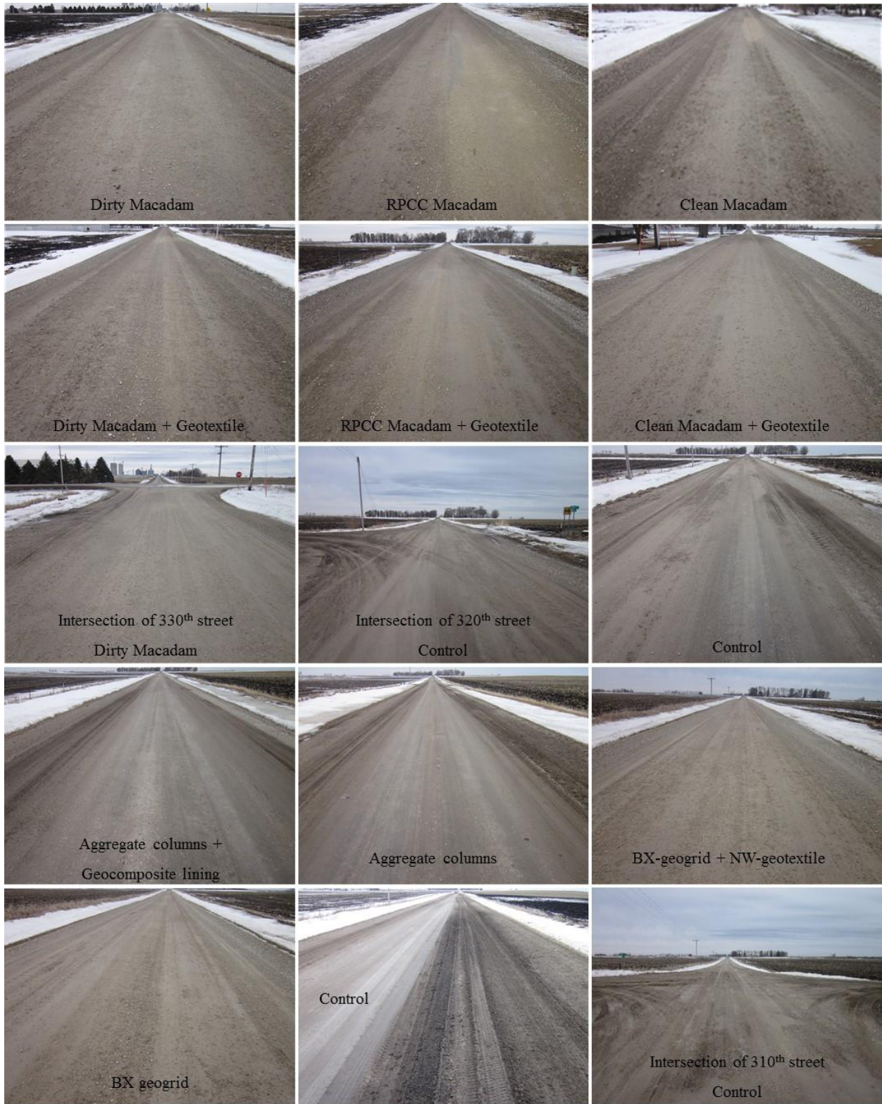
Figure 92. Survey photos of Vail Avenue demonstration sections (March 11, 2014)
