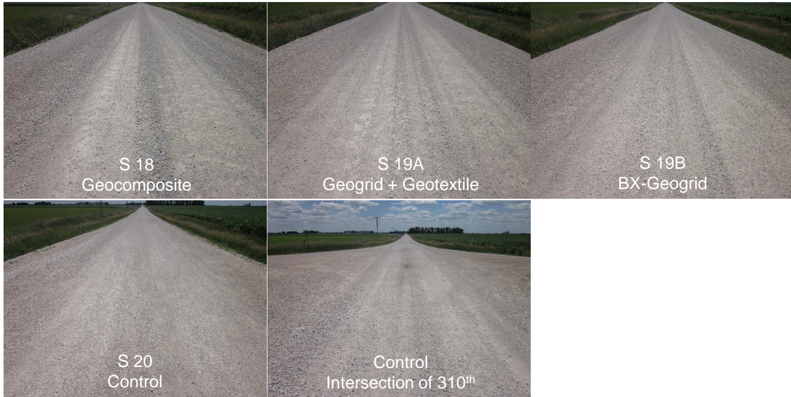
Figure 128. (continued). Survey photos of Vail Avenue demonstration sections (July 3, 2014)
