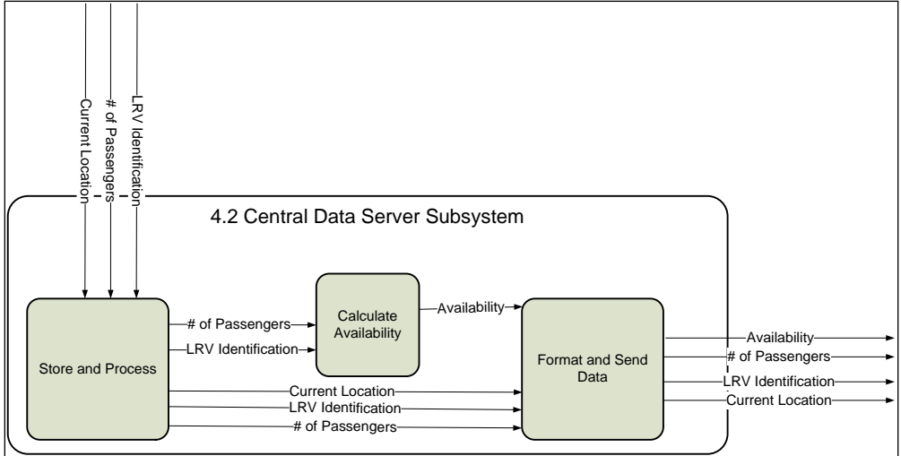
Figure B-7. Central Data Server Subsystem Data Flow Diagram (Source: DART)
