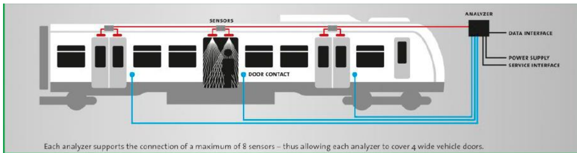
Figure A-4. APC Sensor and Analyzer Configuration (Source: Init)
