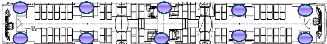
Figure E-4. Location of APC’s Equipment at Each Doorway of an APC-equipped SLRV (Source: DART)
