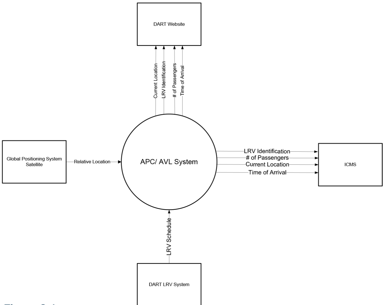
Figure 3-1 Context diagram of real-time transit vehicle data system
