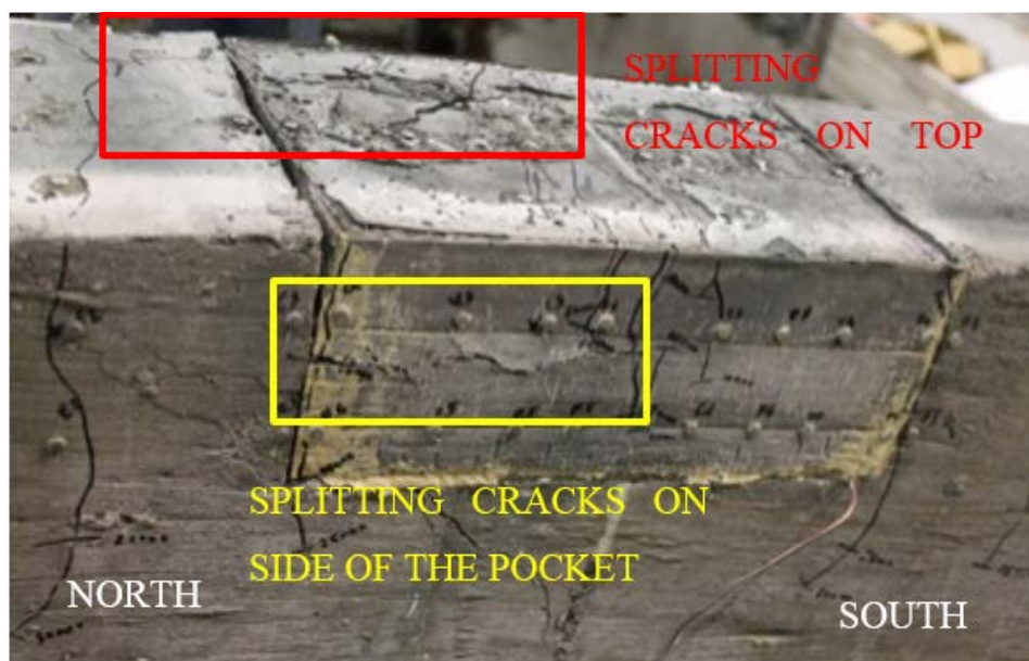
Figure 50. Side View of the UHPC Pocket in Specimen U-6-5-I-E After Failure Showing Splitting Cracks
