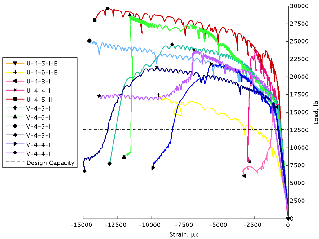
Figure 23. Load vs. Reinforcement Bar (West) Strain for Specimens with No. 4 Bars
