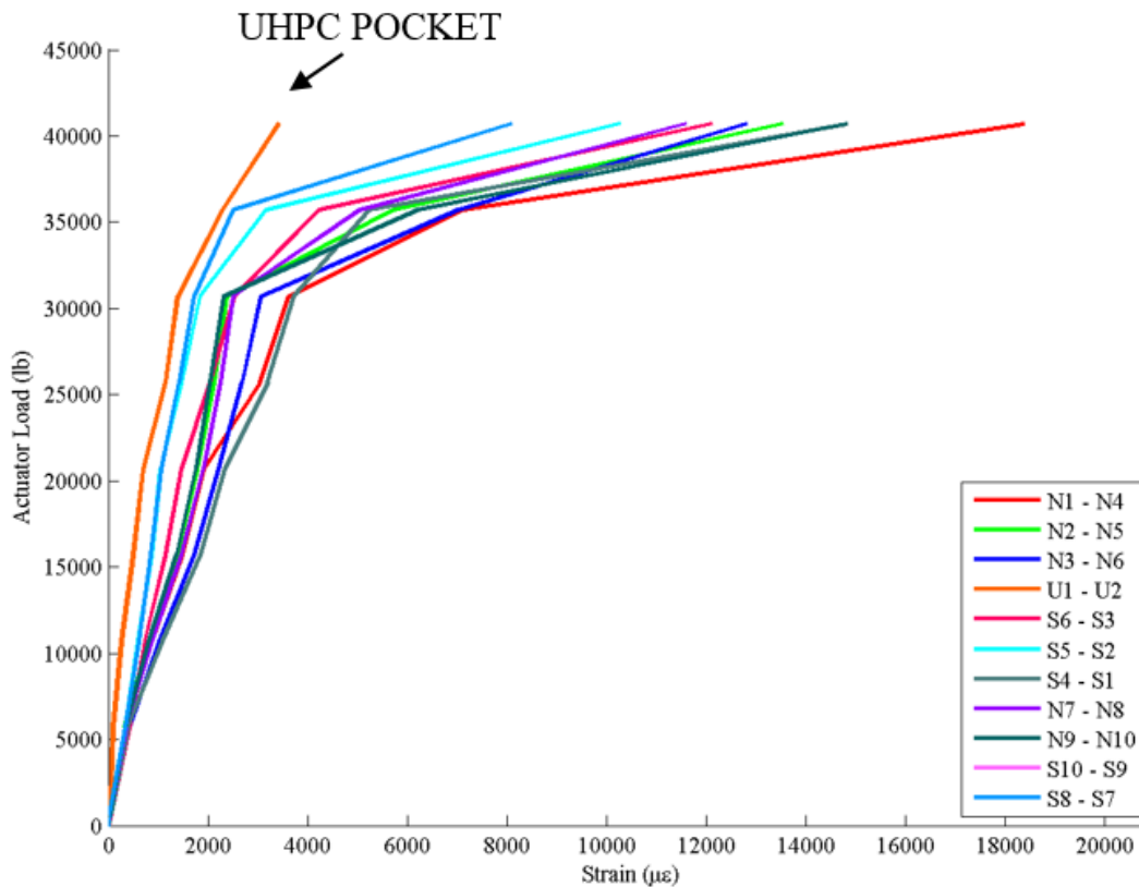
Figure 49. Strain Variation Observed at the Top of the UHPC Pocket in U-6-8-I
