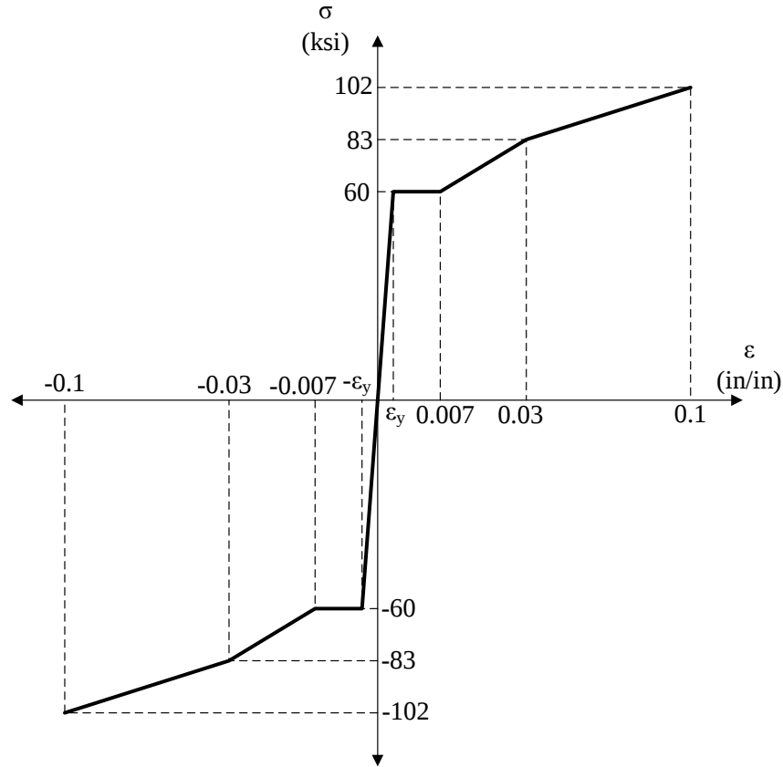
Figure 54. Stress-Strain Relationship for Reinforcing Steel
