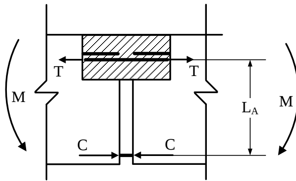
Figure 5. Beam Mechanics: Tension Equals Compression for Equilibrium
