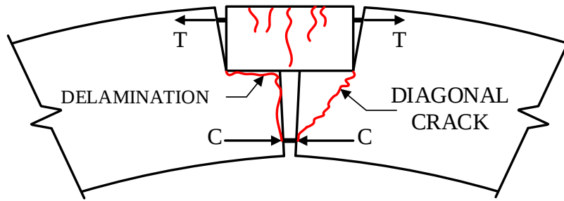
Figure 25. Schematic Representation of Cracks in the Precast Element Under the UHPC Pocket
