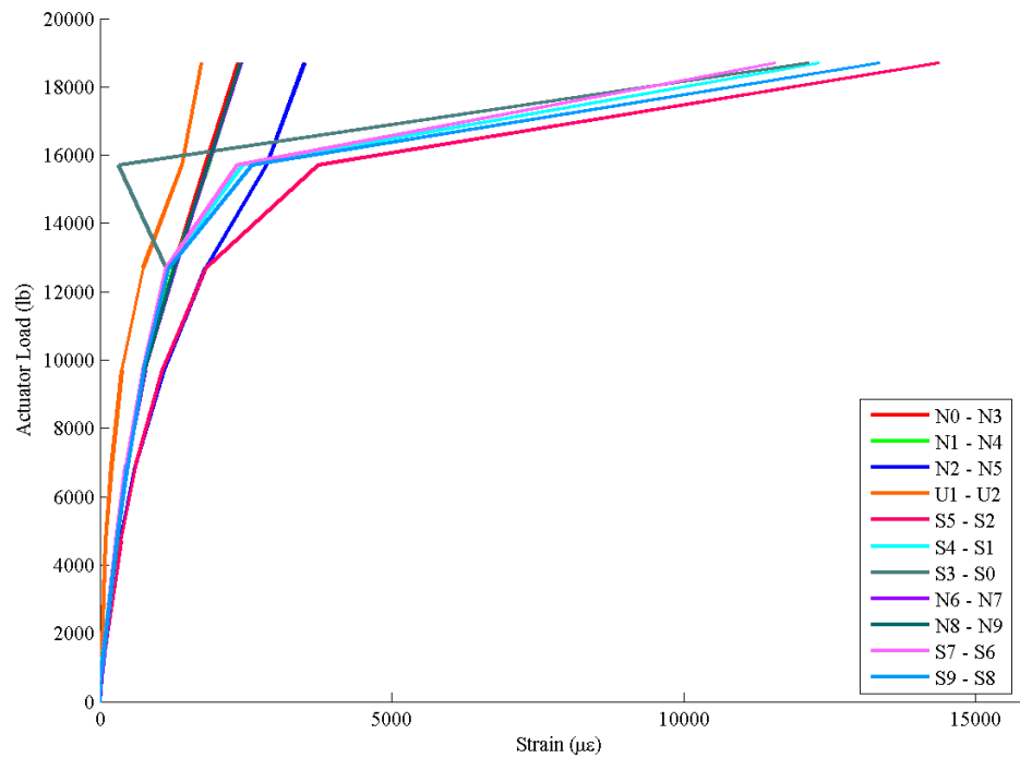
Figure 63. Strain Variation Observed at the Top of the UHPC Pocket in U-4-6-I-E
