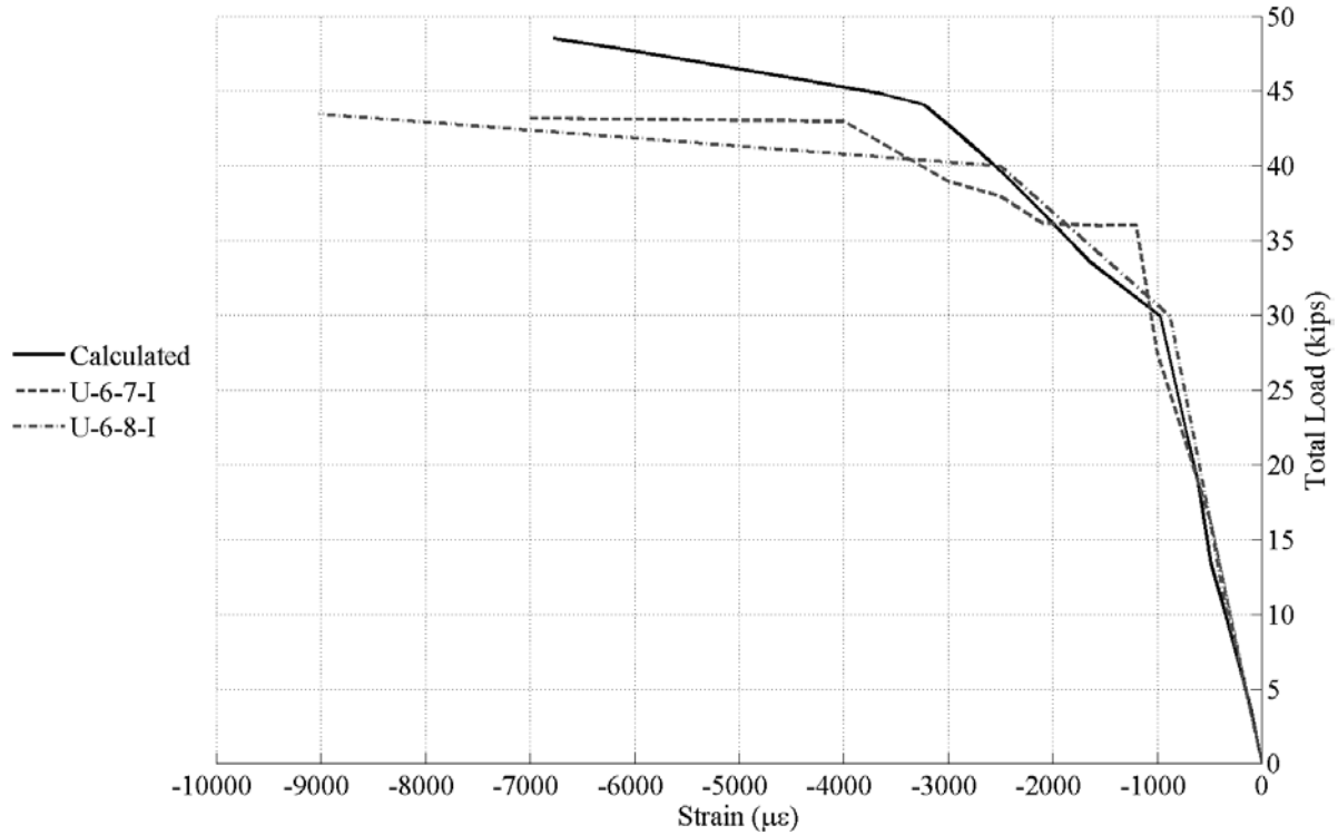
Figure 59. Load vs. Strain at Bottom of Compression Reinforcement for Specimens with Two No. 6 Bars at Top and Two No. 8 Plus One No. 7 at Bottom of Beam
