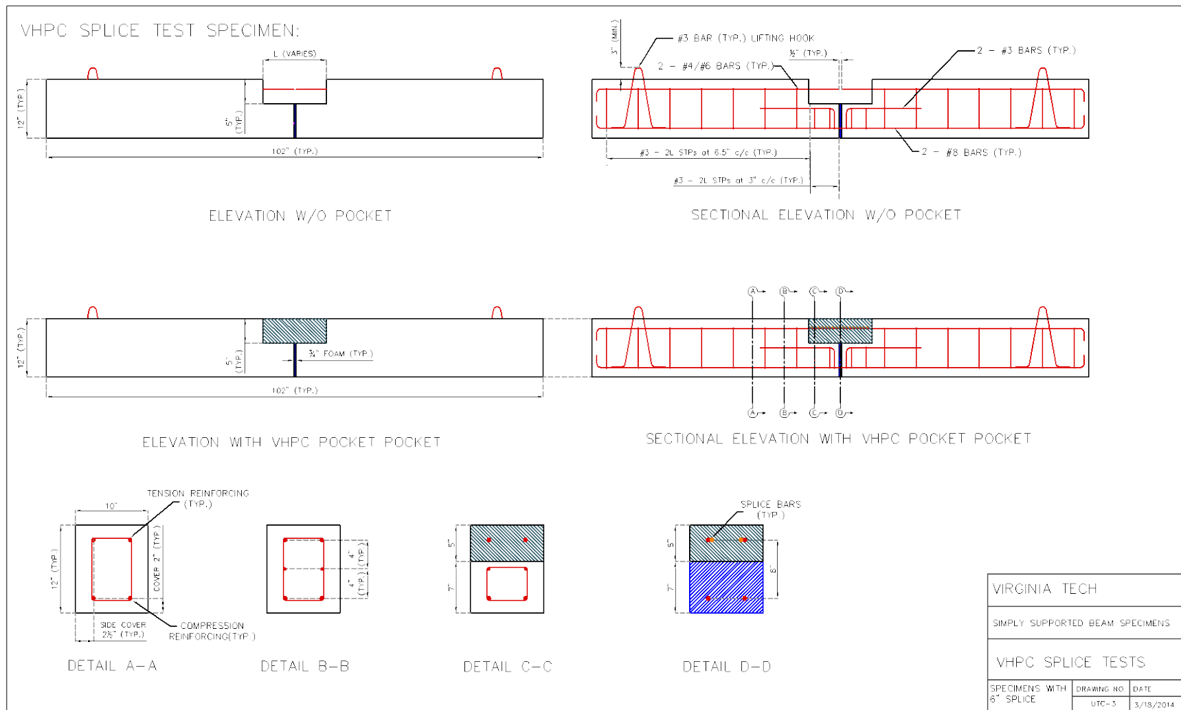
Figure 4. Typical Details of VHPC Test Specimens
