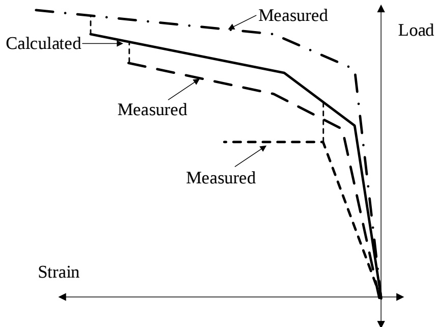
Figure 61. Method for Selecting Strain in Compression Bars at Ultimate
