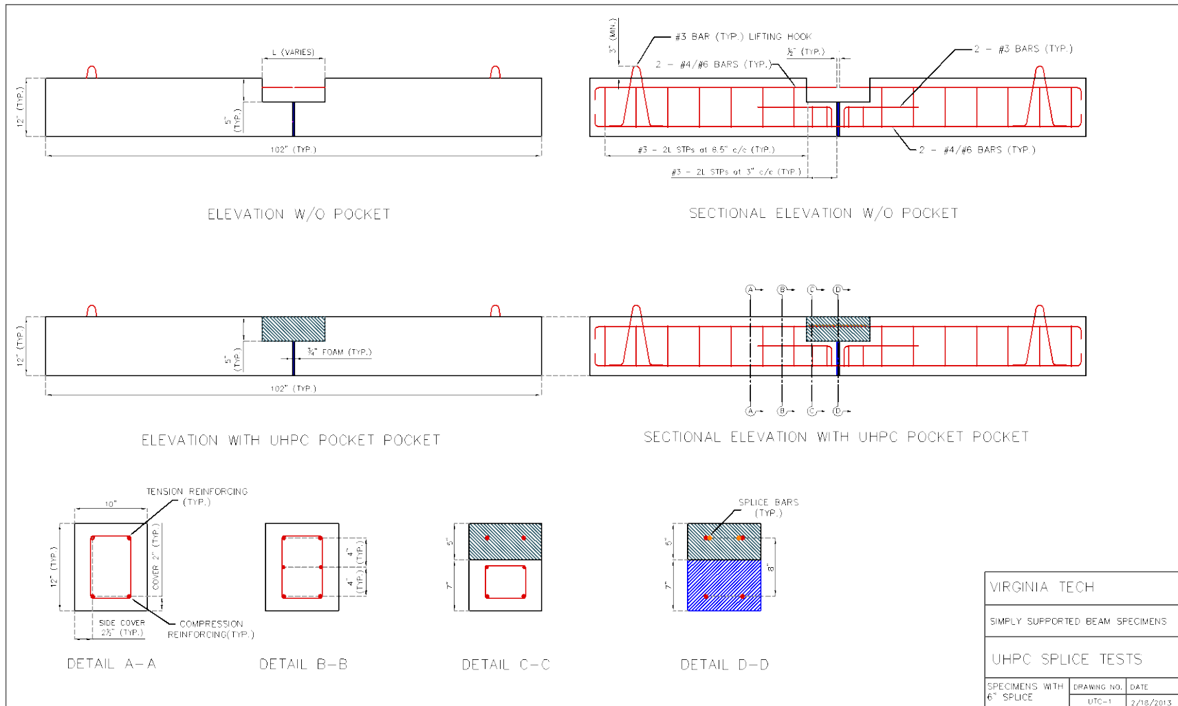
Figure 2. Typical Details of Initial Test Specimens
