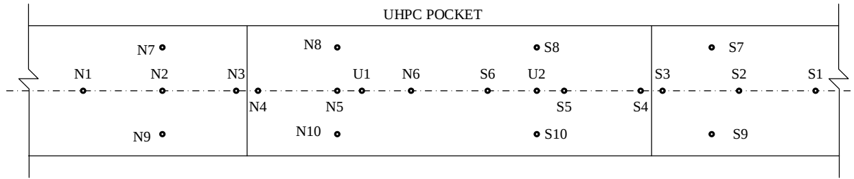
Figure 28. Locations and Designations of Locating Discs for DEMEC Gauge
