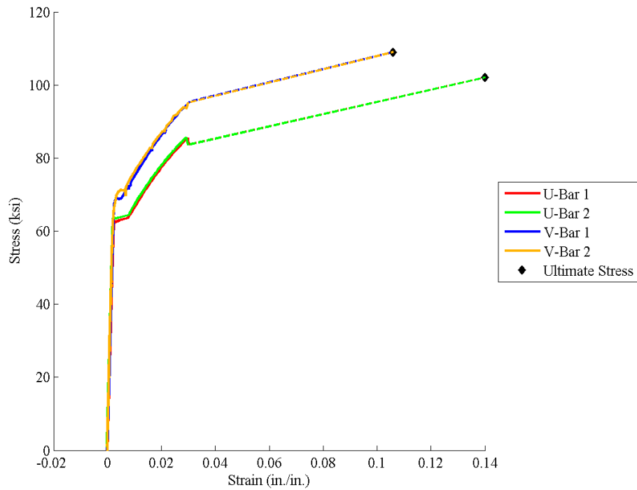
Figure 8. Stress vs. Strain Plot for No. 4 Bars
