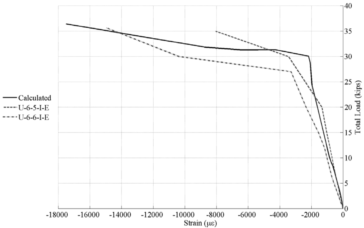
Figure 58. Load vs. Strain at Bottom of Compression Reinforcement for Specimens with Two No. 6 Bars at Top and Bottom of Beam
