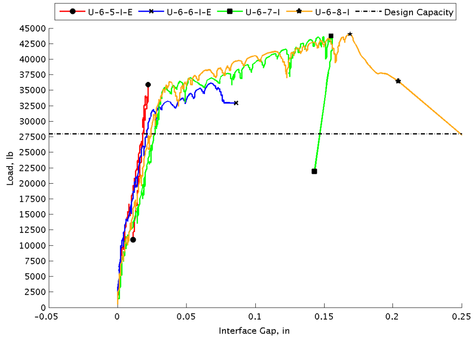
Figure 48. Load vs. South Interface Displacement for All Specimens with No. 6 Bars
