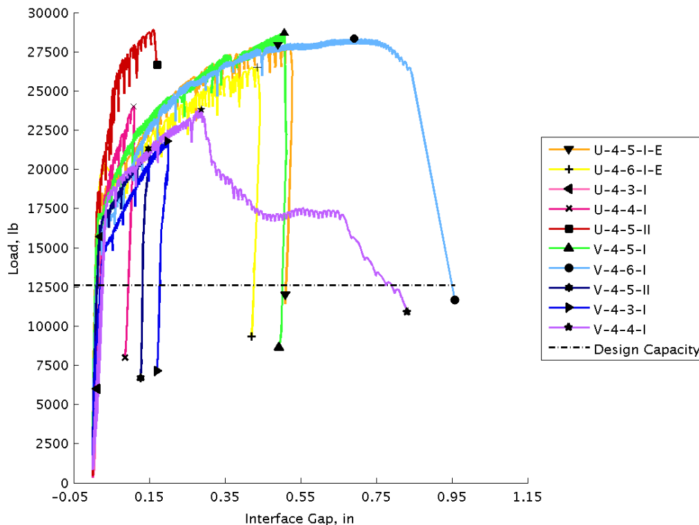
Figure 26. Load vs. North Interface Displacement for Specimens with No. 4 Bars
