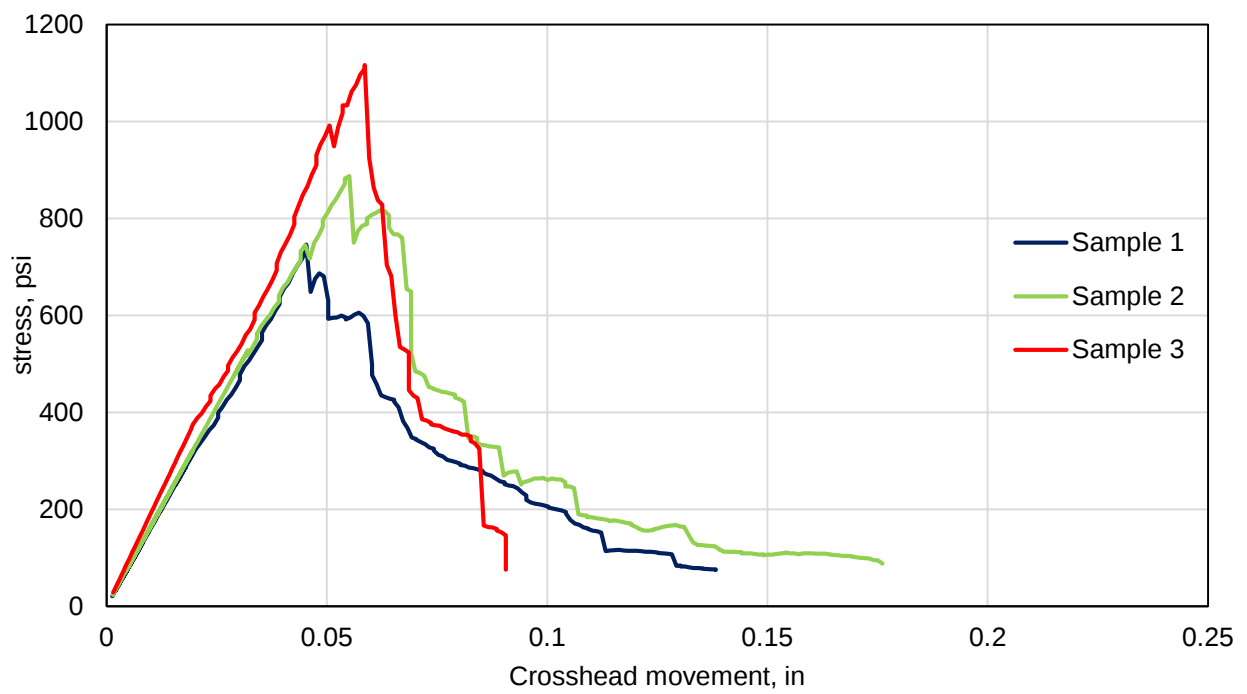
Figure 14. UHPC Dog Bone Test
