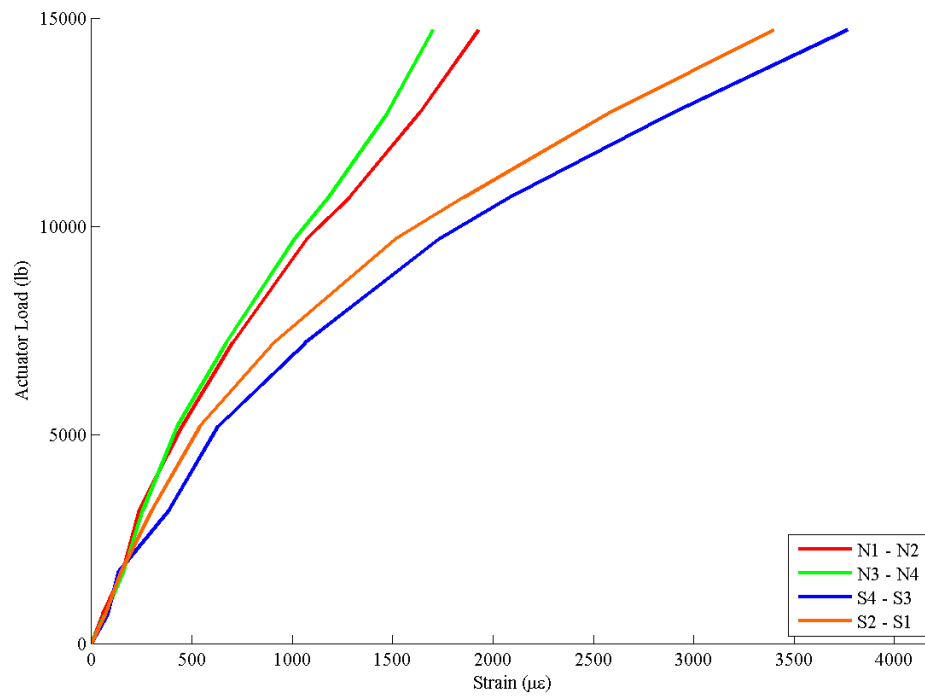
Figure 66. Strain Variation Observed at the Top of the UHPC Pocket in U-4-6-I-E
