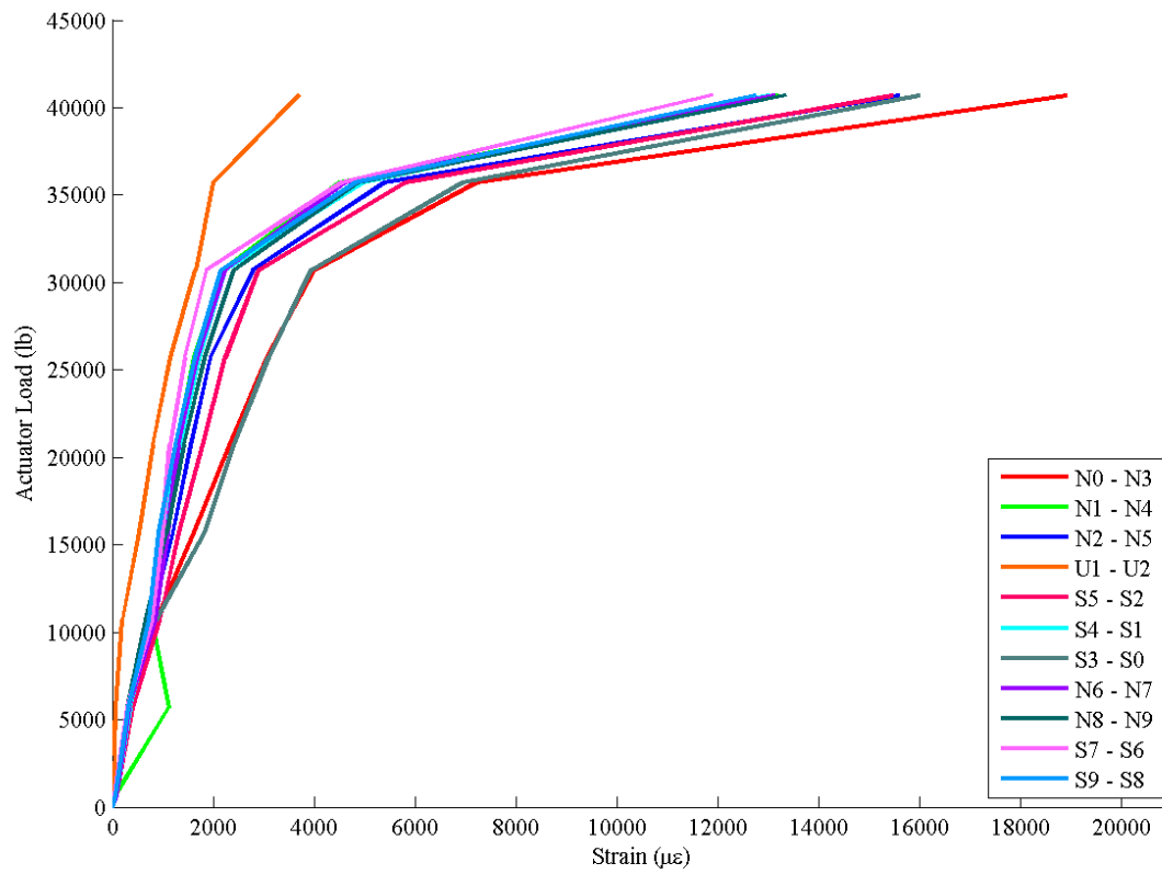
Figure 68. Strain Variation Observed at the Top of the UHPC Pocket in U-6-7-I
