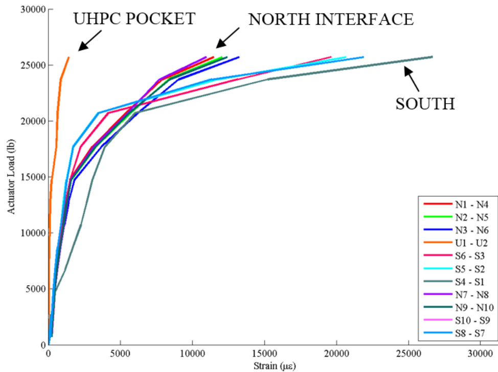
Figure 29. DEMEC Strain Measurements at the Top of the Beam for Specimen U-4-5-I-E
