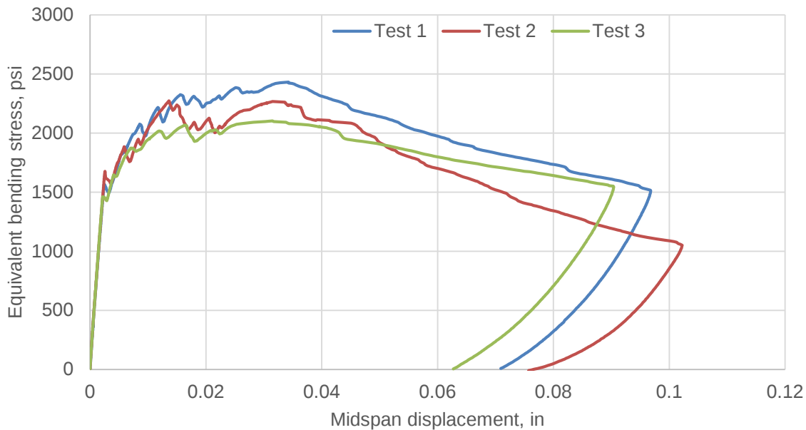
Figure 12. Flexural Beam Test Results for VHPC at 7 Days
