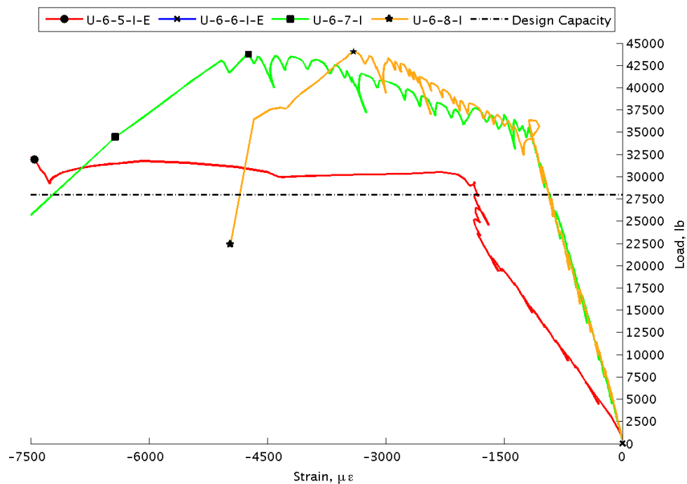
Figure 45. Load vs. Reinforcement Strain (East) for All Specimens with No. 6 Bars
