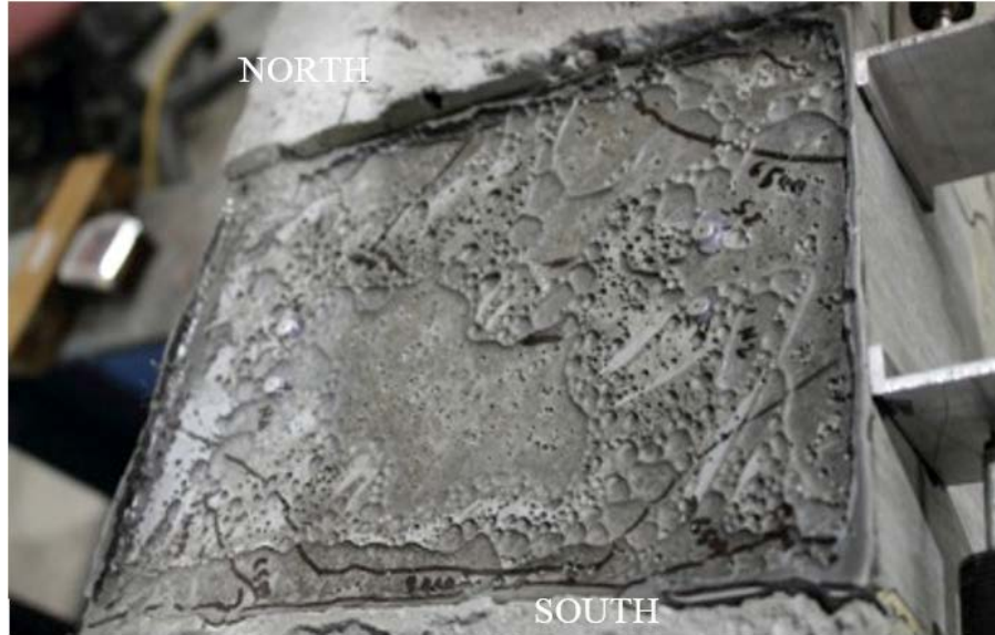
Figure 32. UHPC Pocket in Specimen U-4-3-I Showing Cracks Near the Interfaces and the Corners
