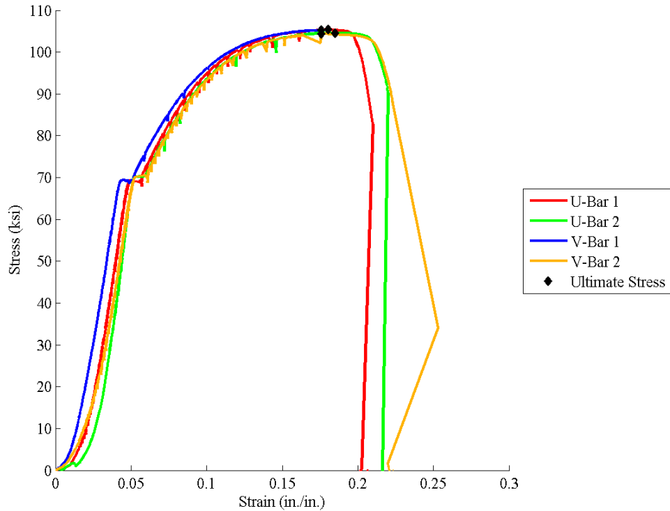
Figure 11. Stress vs. Strain Plot for No. 8 Bars
