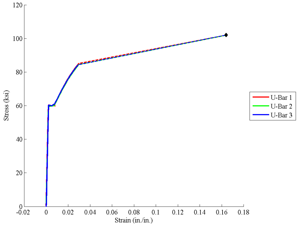
Figure 9. Stress vs. Strain Plot for No. 6 Bars
