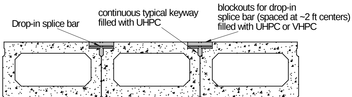
Figure 1. Adjacent Box Beam Connection with Drop-In Splice Bar
