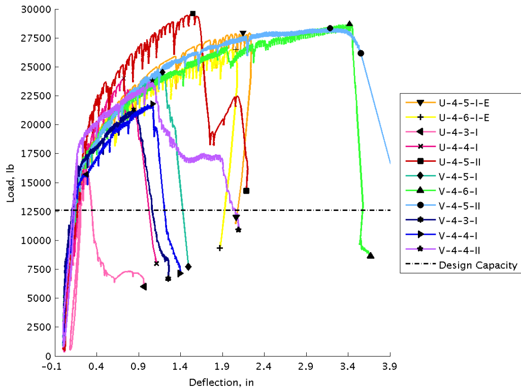
Figure 20. Load vs. North End Deflection for Specimens with No. 4 Bars
