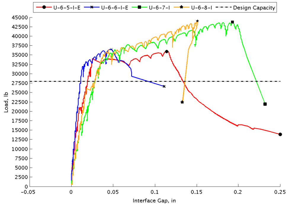
Figure 47. Load vs. North Interface Displacement for All Specimens with No. 6 Bars
