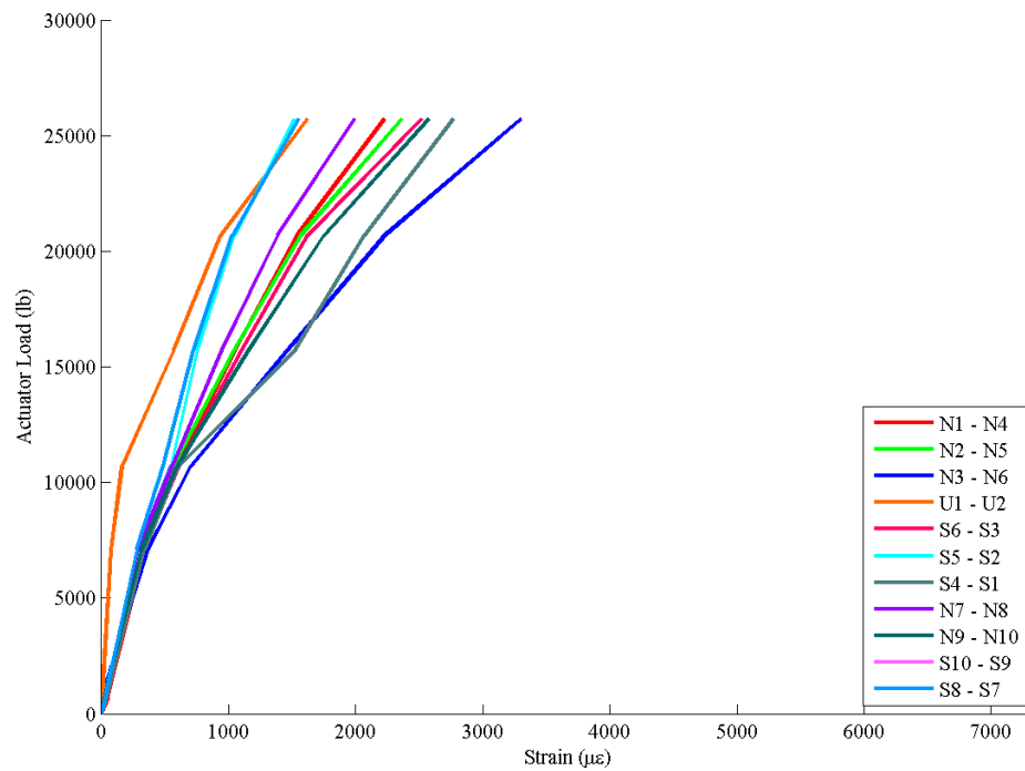
Figure 65. Strain Variation Observed at the Top of the UHPC Pocket in U-4-4-I
