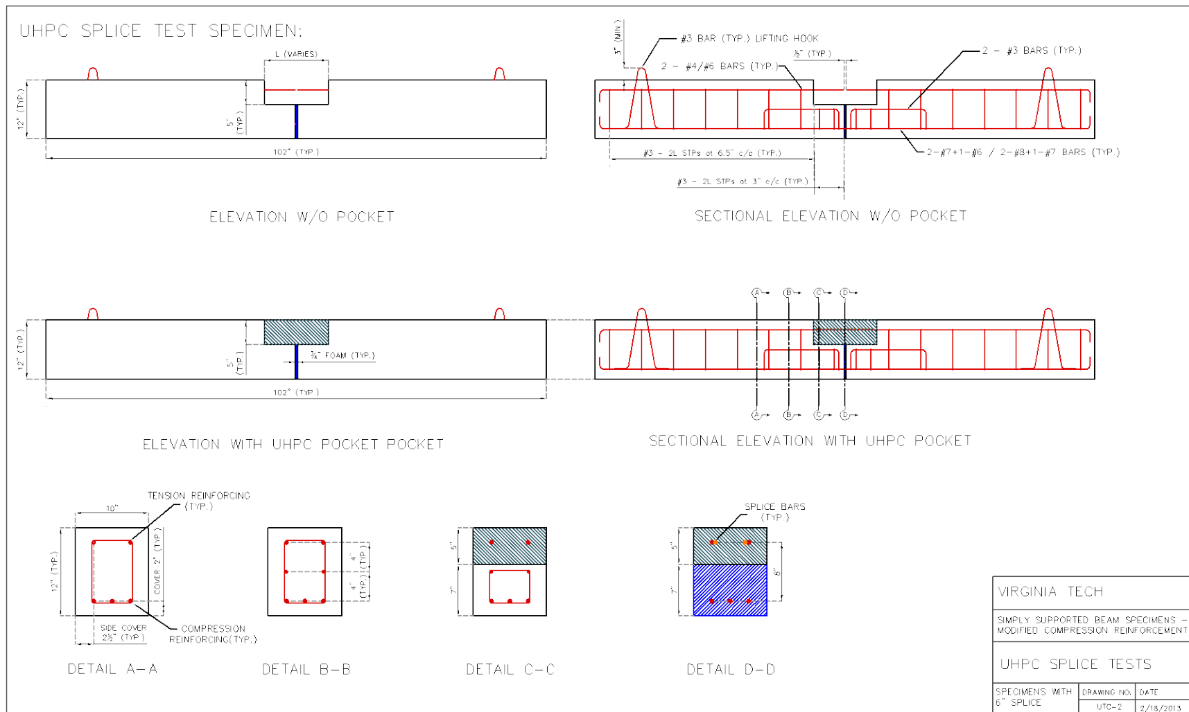
Figure 3. Typical Details of Modified Test Specimens
