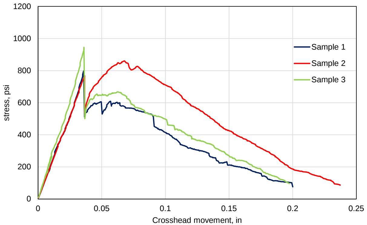
Figure 15. UHPC Dog Bone Test
