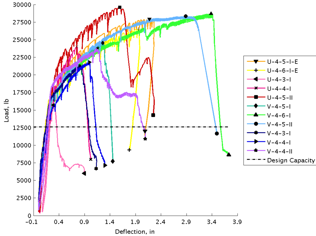
Figure 19. Load vs. South End Deflection for All Specimens with No. 4 Bars
