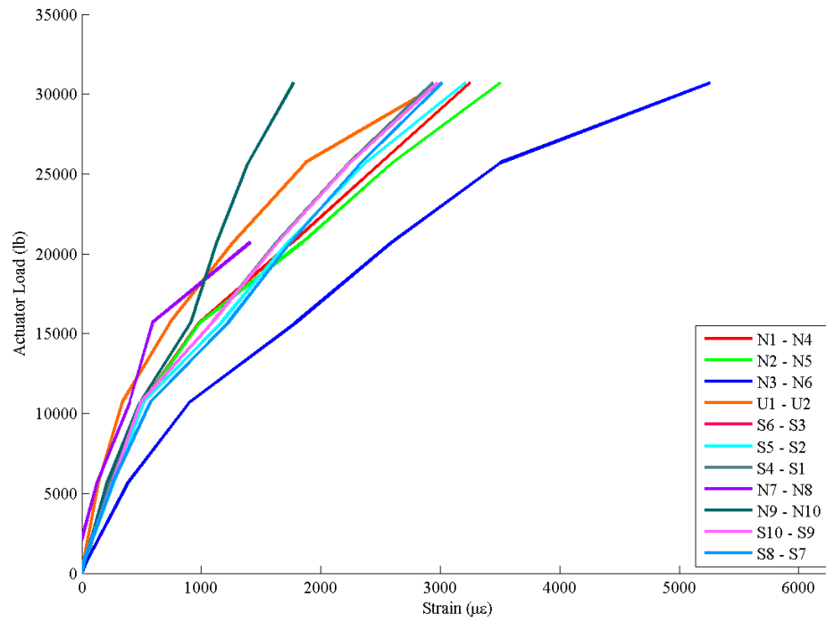
Figure 64. Strain Variation Observed at the Top of the UHPC Pocket in U-4-3-I
