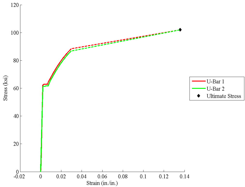
Figure 10. Stress vs. Strain Plot for No. 7 Bars
