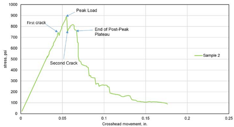
Figure 16. Cracking Behavior of VHPC Dog Bone Sample 2
