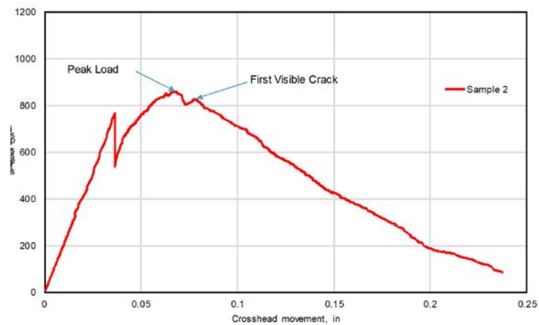
Figure 17. UHPC Cracking Behavior
