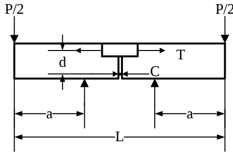
Figure 24. Force in Compressive Reinforcement from Externally Applied Loads
