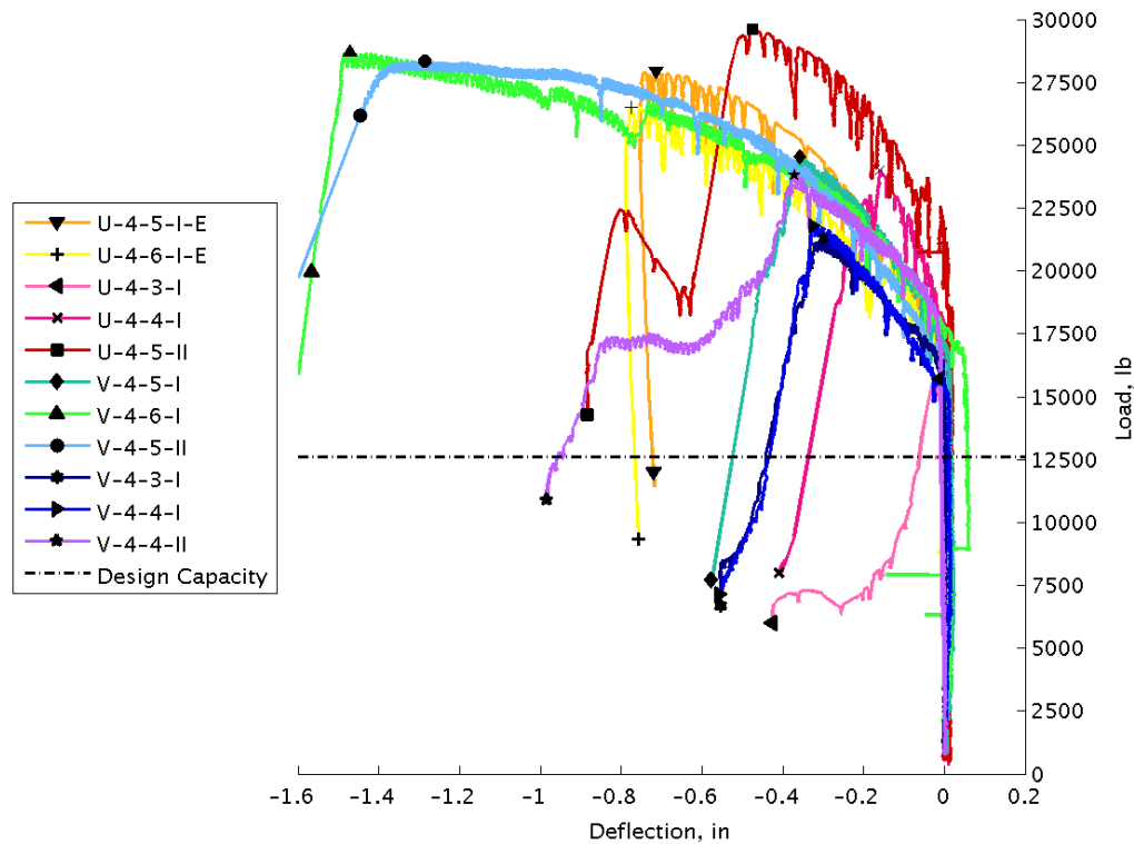
Figure 21. Load vs. Midspan Deflection for Specimens with No. 4 Bars
