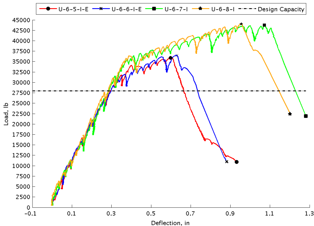
Figure 42. Load vs. South Deflection for All Specimens with No. 6 Bars
