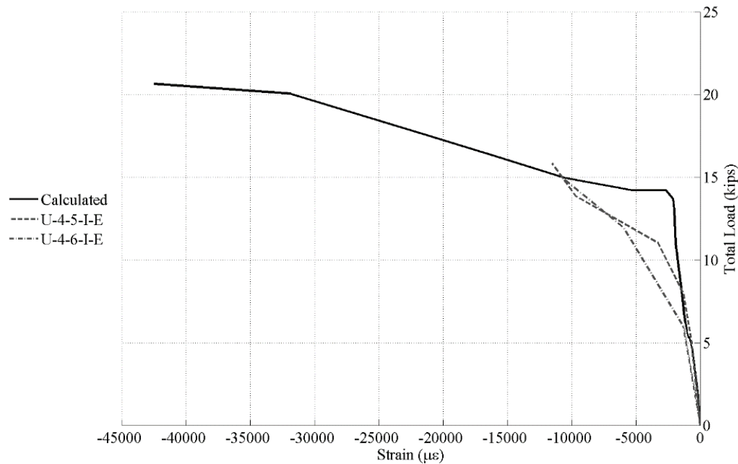
Figure 56. Load vs. Strain at Bottom of Compression Reinforcement for Specimens with Two No. 4 Bars at Top and Bottom of Beam
