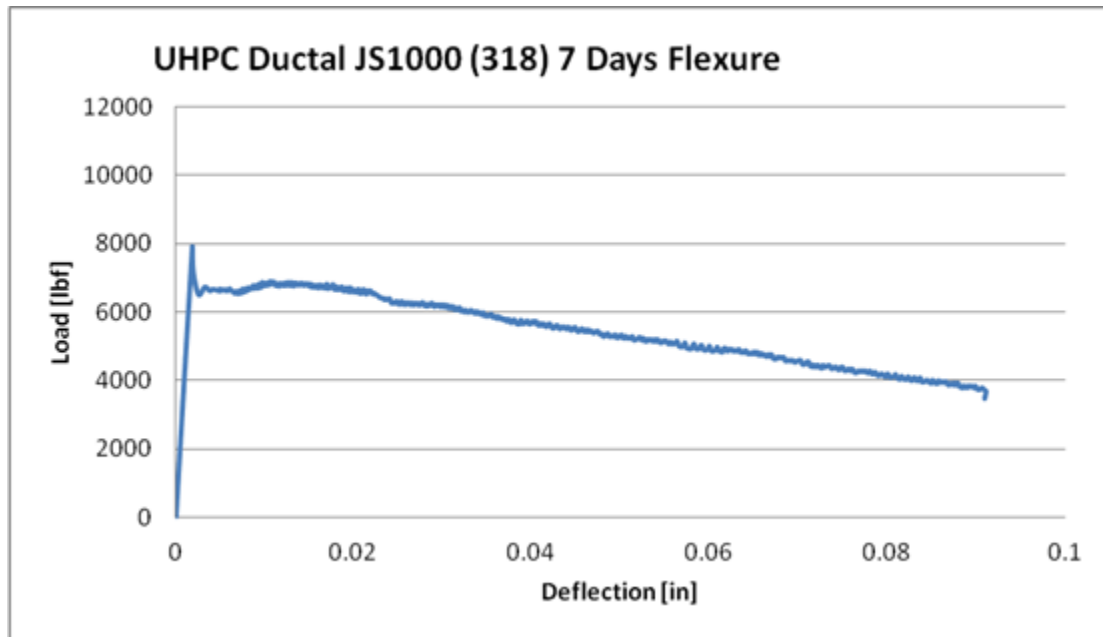
Figure 13. Typical 7 Day Flexural Beam Test Results for Untreated UHPC
