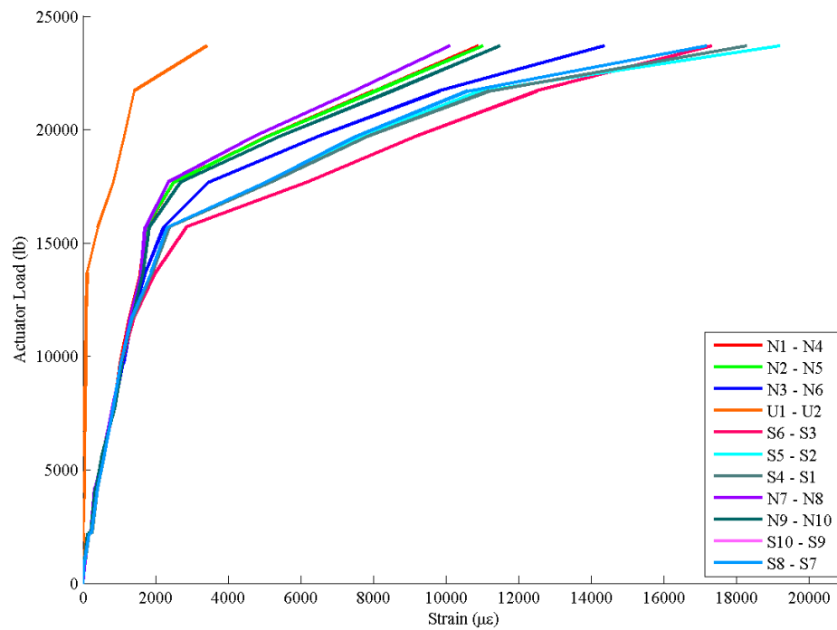
Figure 67. Strain Variation Observed at the Top of the UHPC Pocket in U-6-5-I-E
