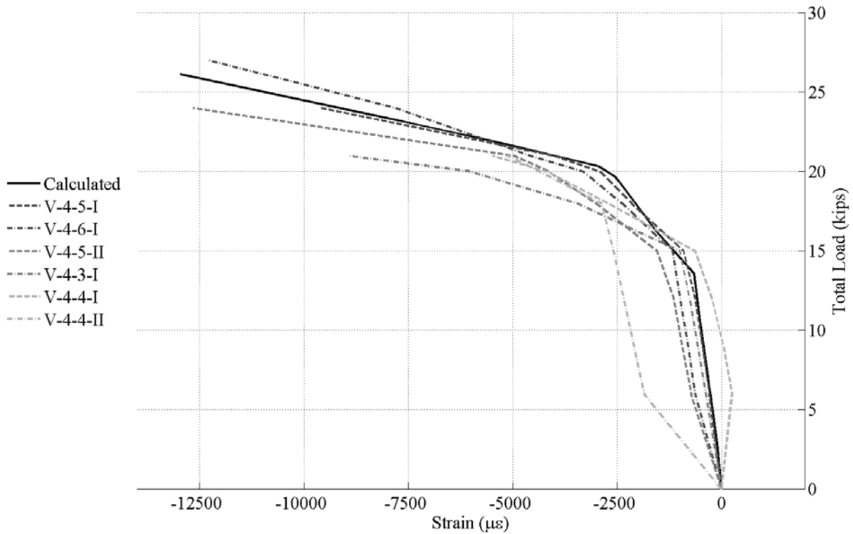
Figure 60. Load vs. Strain at Bottom of Compression Reinforcement for Specimens with Two No. 4 Bars at Top and Two No. 8 at Bottom of Beam with VHPC
