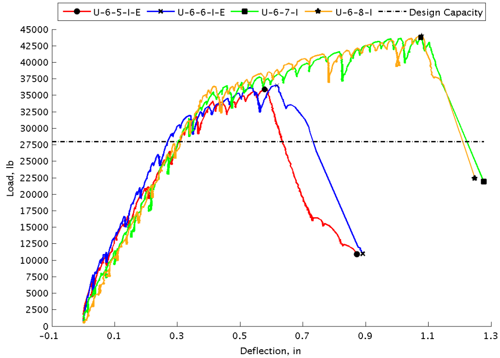
Figure 43. Load vs. North Deflection for All Specimens with No. 6 Bars
