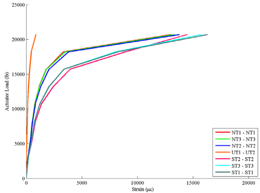
Figure 62. Strain Variation Observed at the Top of the UHPC Pocket in U-4-5-I-E
