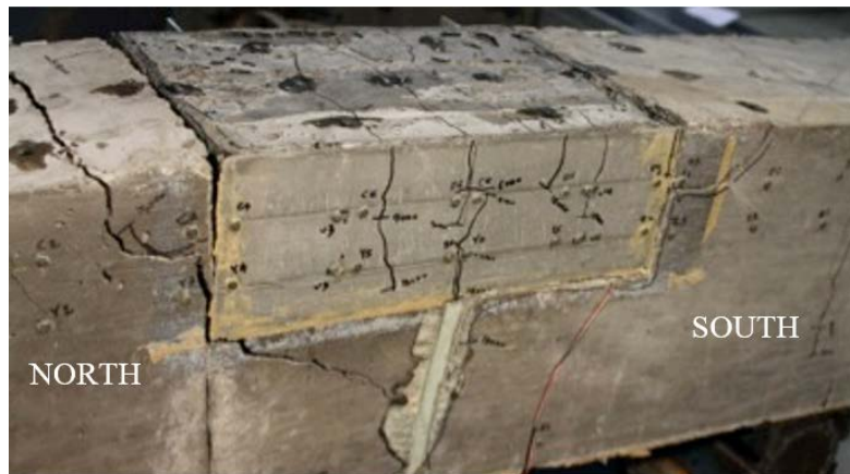
Figure 31. UHPC Pocket in Specimen U-4-6-I-E at End of Load Application Showing Flexural Cracks
