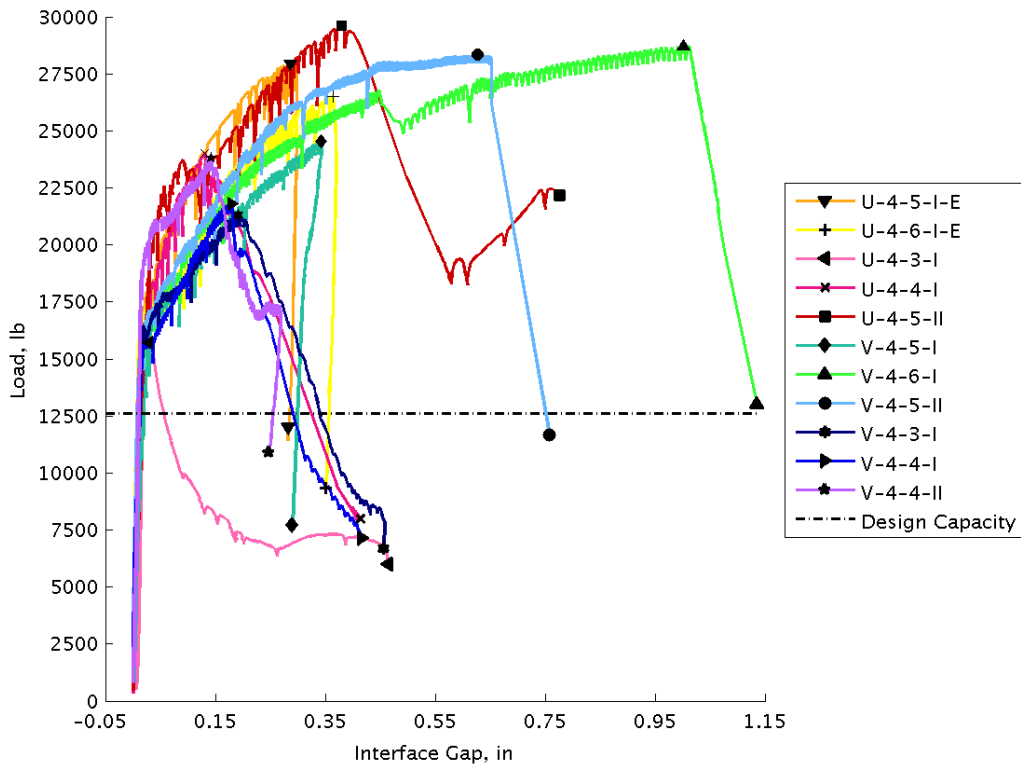
Figure 27. Load vs. South Interface Displacement for Specimens with No.4 Bars
