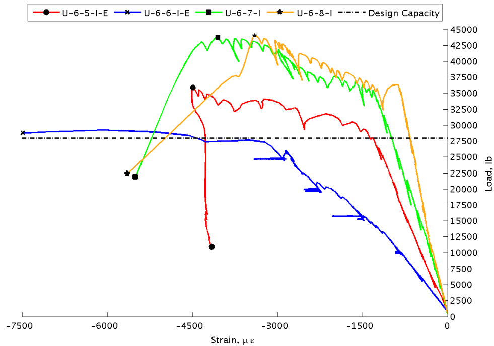
Figure 46. Load vs. Reinforcement Strain (West) for All Specimens with No. 6 Bars
