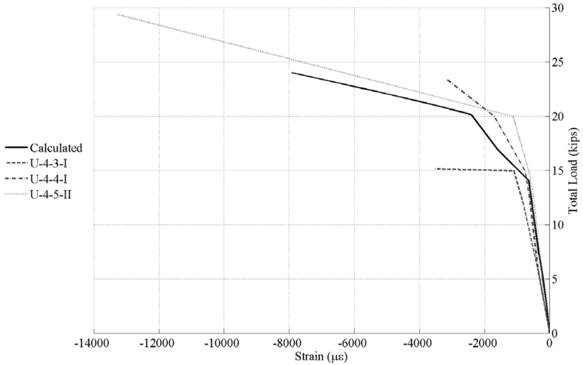
Figure 57. Load vs. Strain at Bottom of Compression Reinforcement for Specimens with Two No. 4 Bars at Top and Two No. 7 Plus One No. 6 at Bottom of Beam
