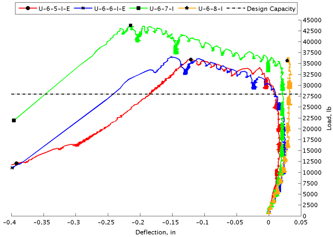
Figure 44. Load vs. Midspan Deflection for All Specimens with No. 6 Bars
