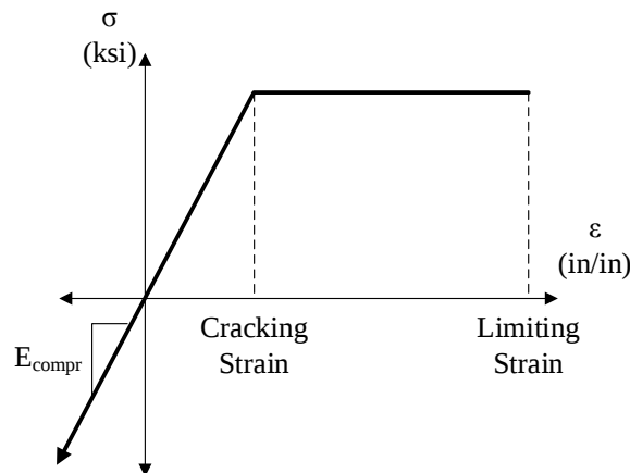
Figure 55. Constitutive Model for UHPC and VHPC
