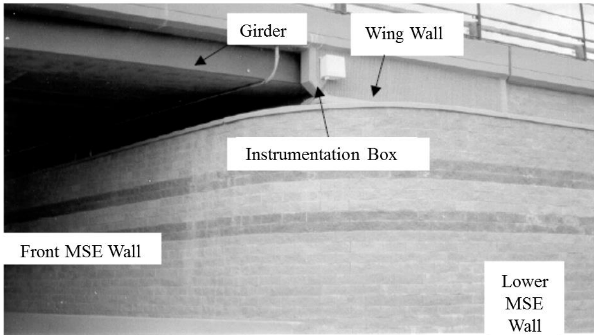
Figure 11 View of the south-east side of the completed Founders/Meadows Bridge (Abu-Hejleh et al. 2000)
