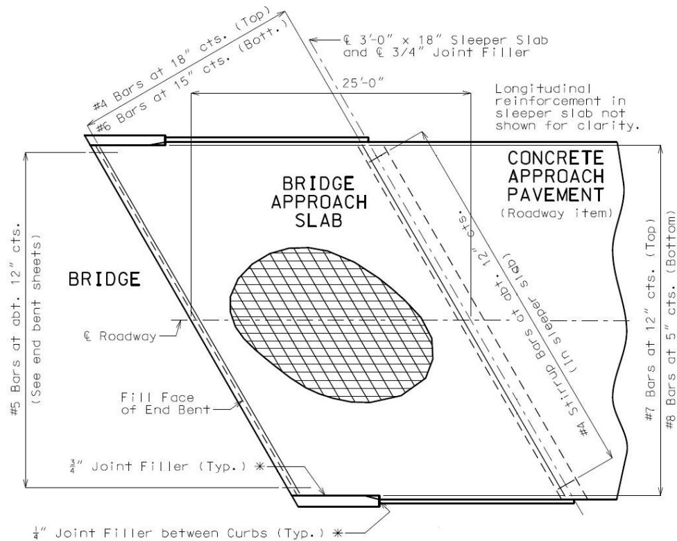
Figure 25 Plan view of the approach slab system used in Missouri (MODOT, 2014)
