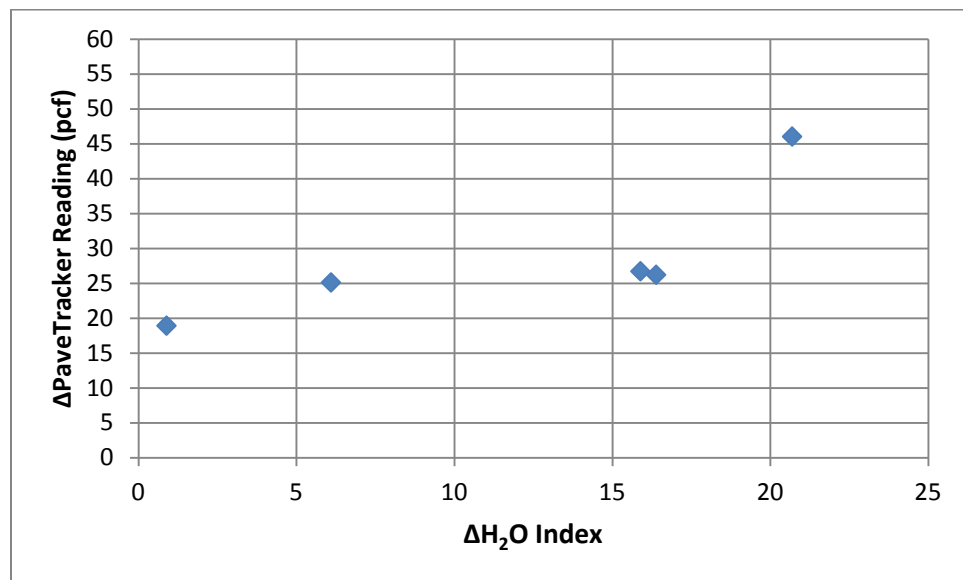
Figure 31. PT Old Laboratory Density Change with Moisture Content for Slab 2 (2012)
