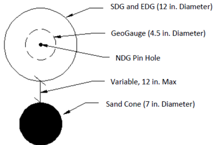
Figure 16. Unbound Field Testing Pattern
