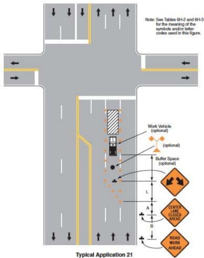
Exhibit 2: Typical Through Lane Closure at Signalized Intersections
