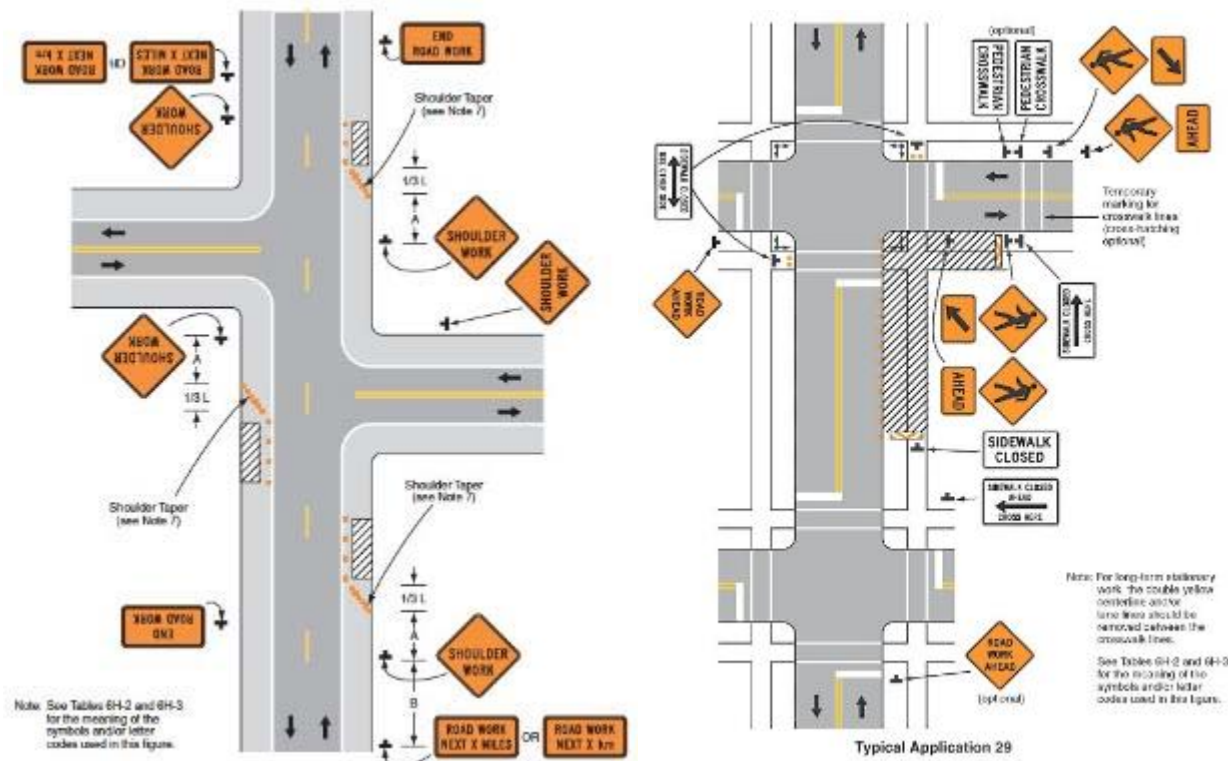
Exhibit 1: Typical Shoulder (Left), and Sidewalk or Crosswalk (Right) Closure
