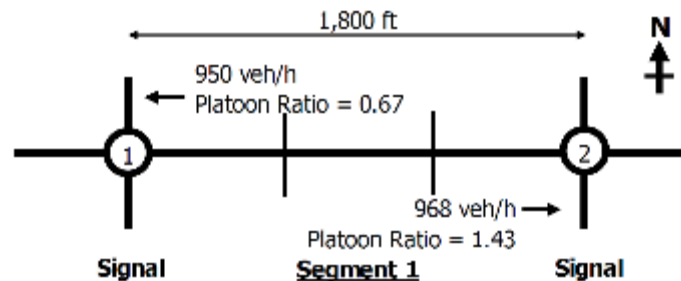
Exhibit 9 Example of an Urban Street (Source: HCM2010, Exhibit 30-13)
