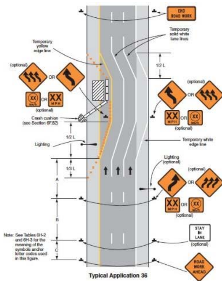
Exhibit 4: Typical Lane Shift Work Zones
