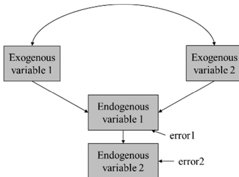
Exhibit 49: Path Diagram
