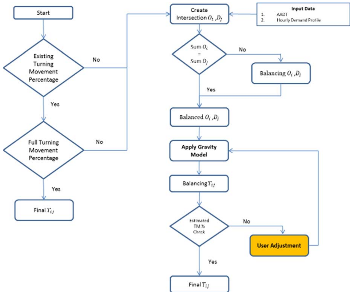
Exhibit 64: Gravity Model Estimation Process
