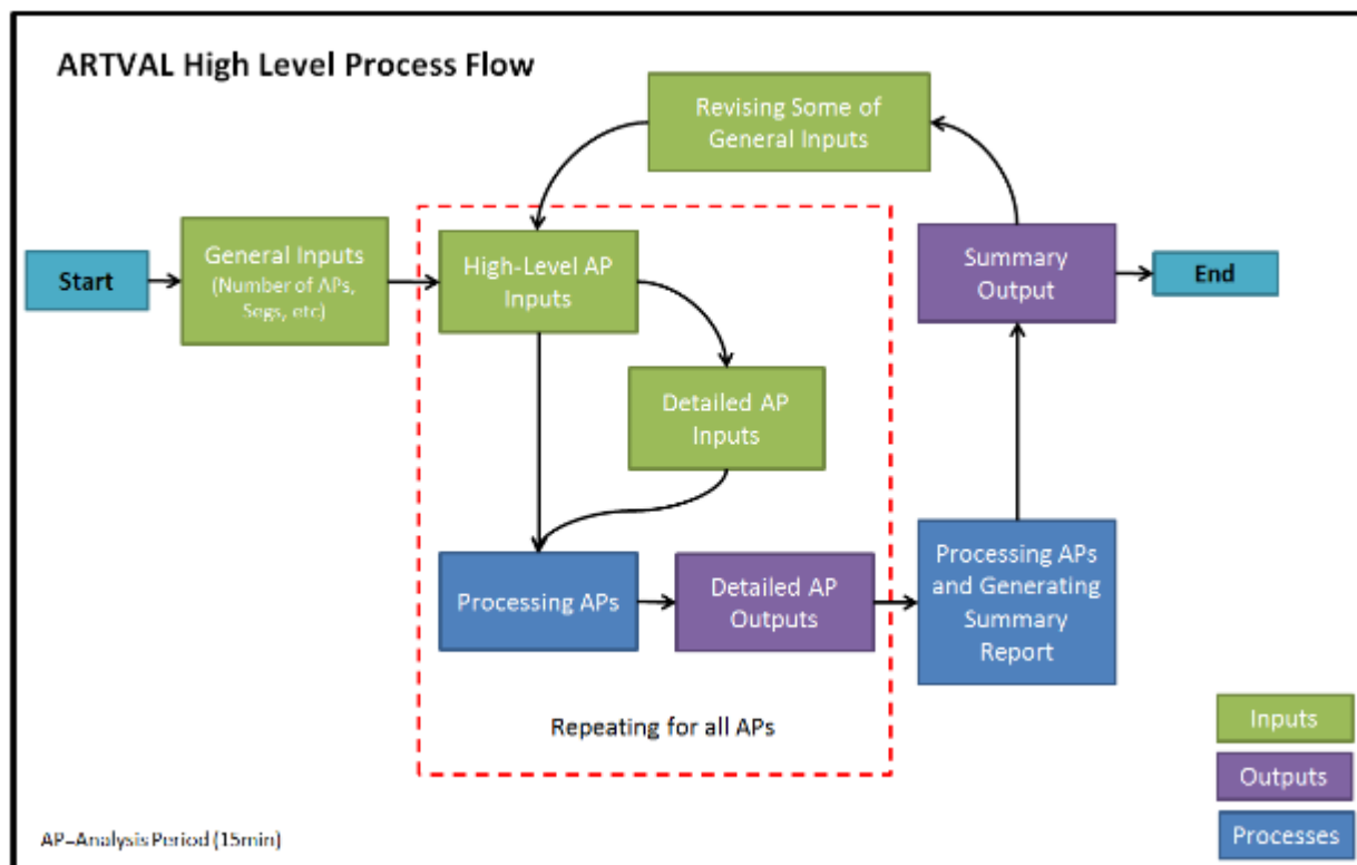
Exhibit 19: ARTVAL high-level process flow
