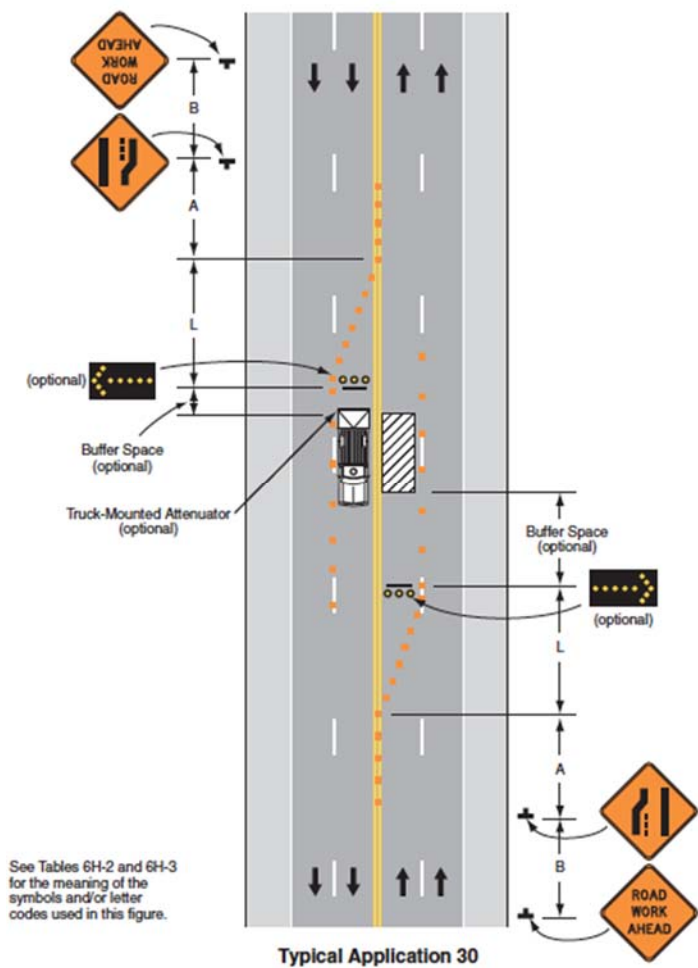
Exhibit 3: Typical Inside Lane Closure at Mid-segment Work Zones
