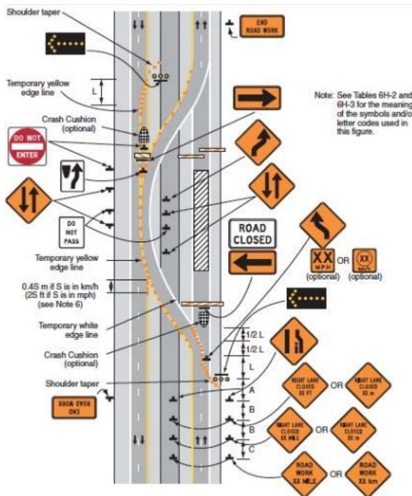
Exhibit 5: Typical Median Crossover Work Zones
