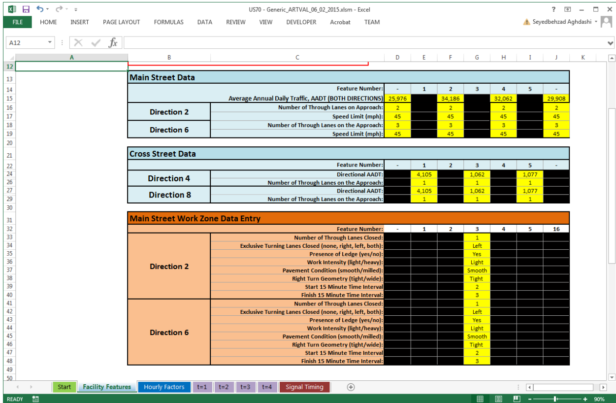
Figure 5 – Demand and Work Zone Data Entry in Facility Features Worksheet
