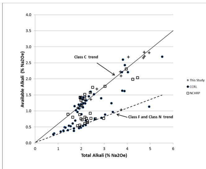
Relationship between total alkali and available alkali for fly ash
