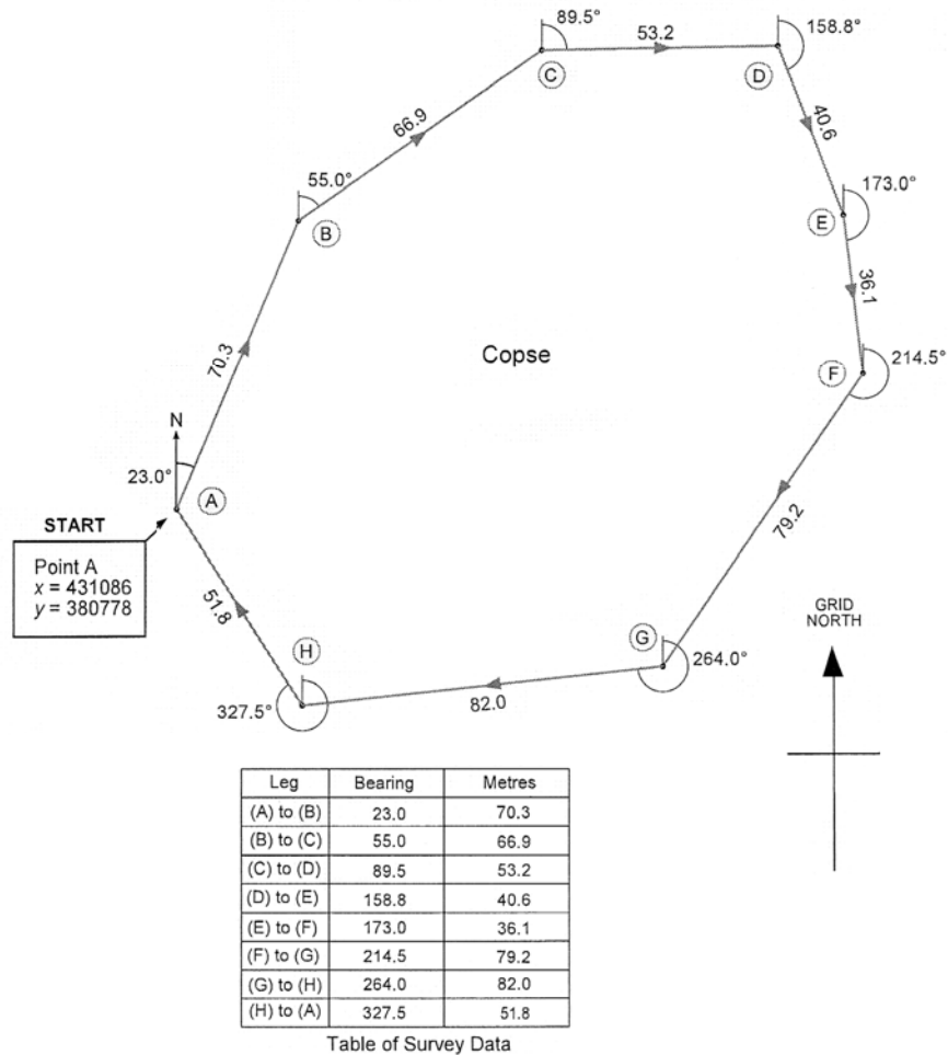
Figure 2.3 Closed Traverse Survey [TCPD 2012].
