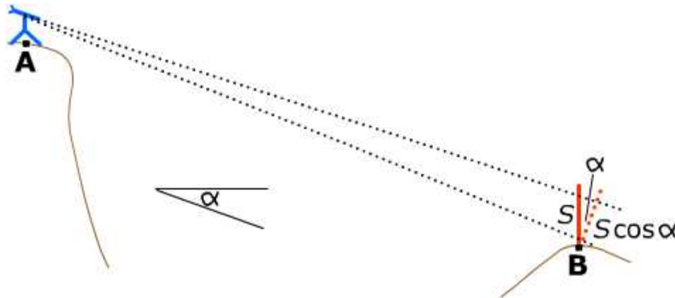
Figure 2.4 Geometry of Tacheometric Surveying. [American Mathematical Society]
