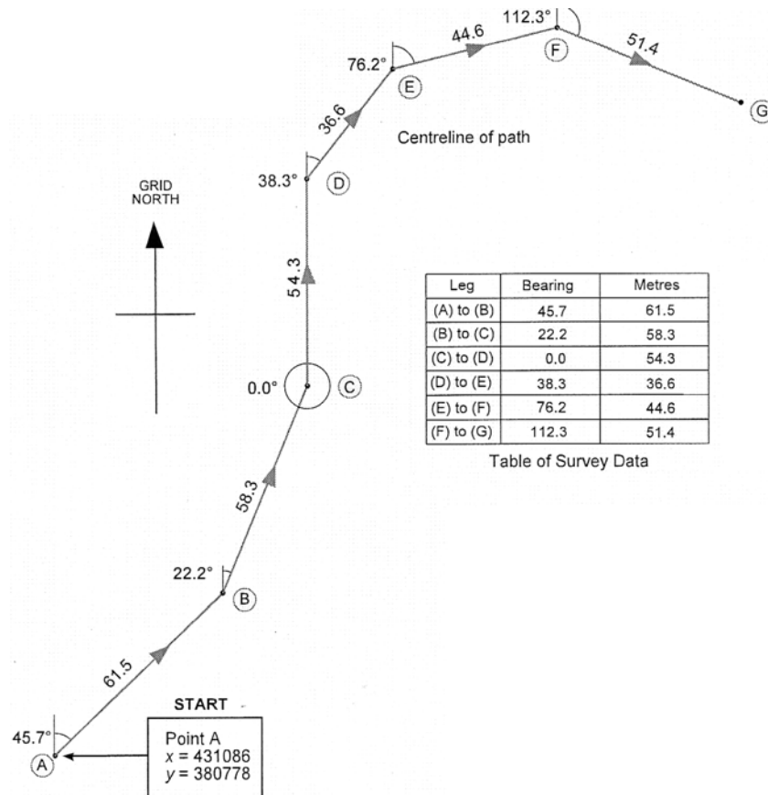
Figure 2.2 Open Traverse Survey [TCPD 2012]
