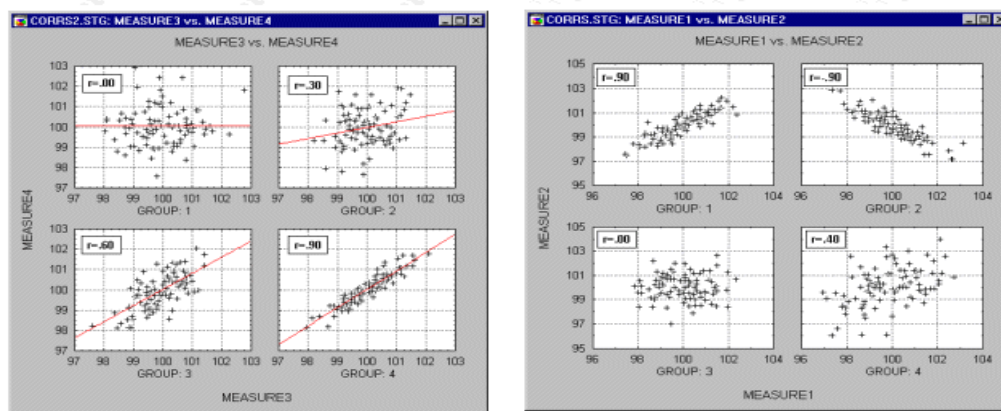
Figure 4.1 Sample data with corresponding r values.
