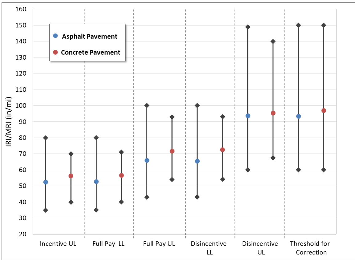
Figure 5 Comparison of specification thresholds for asphalt and concrete pavement for IRI/MRI
