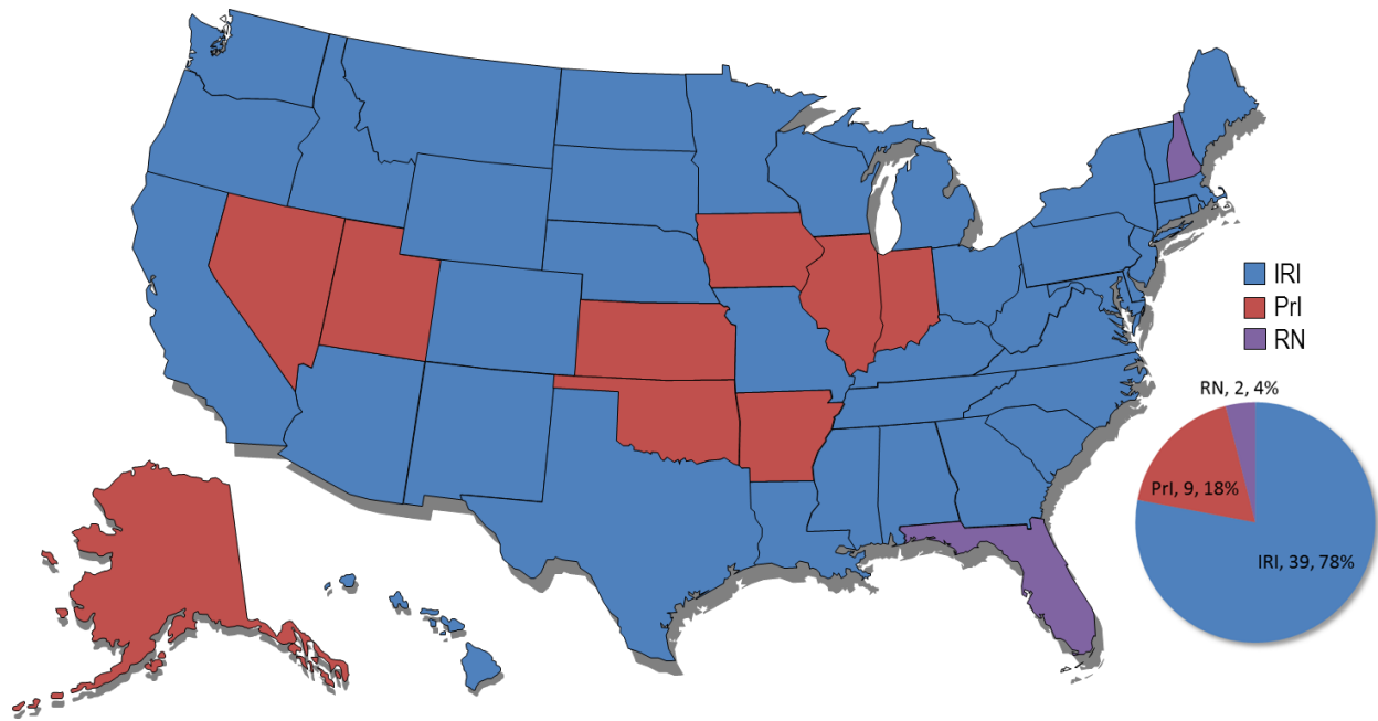
Figure 1 Smoothness specifications for asphalt pavements by state
