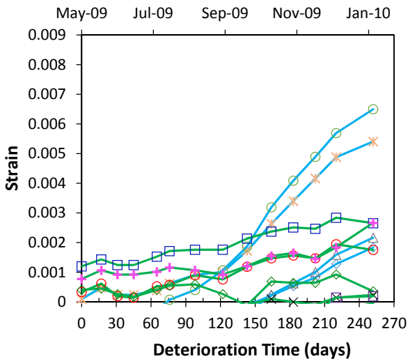
(c) Vertical DEMEC Strains in Joint
