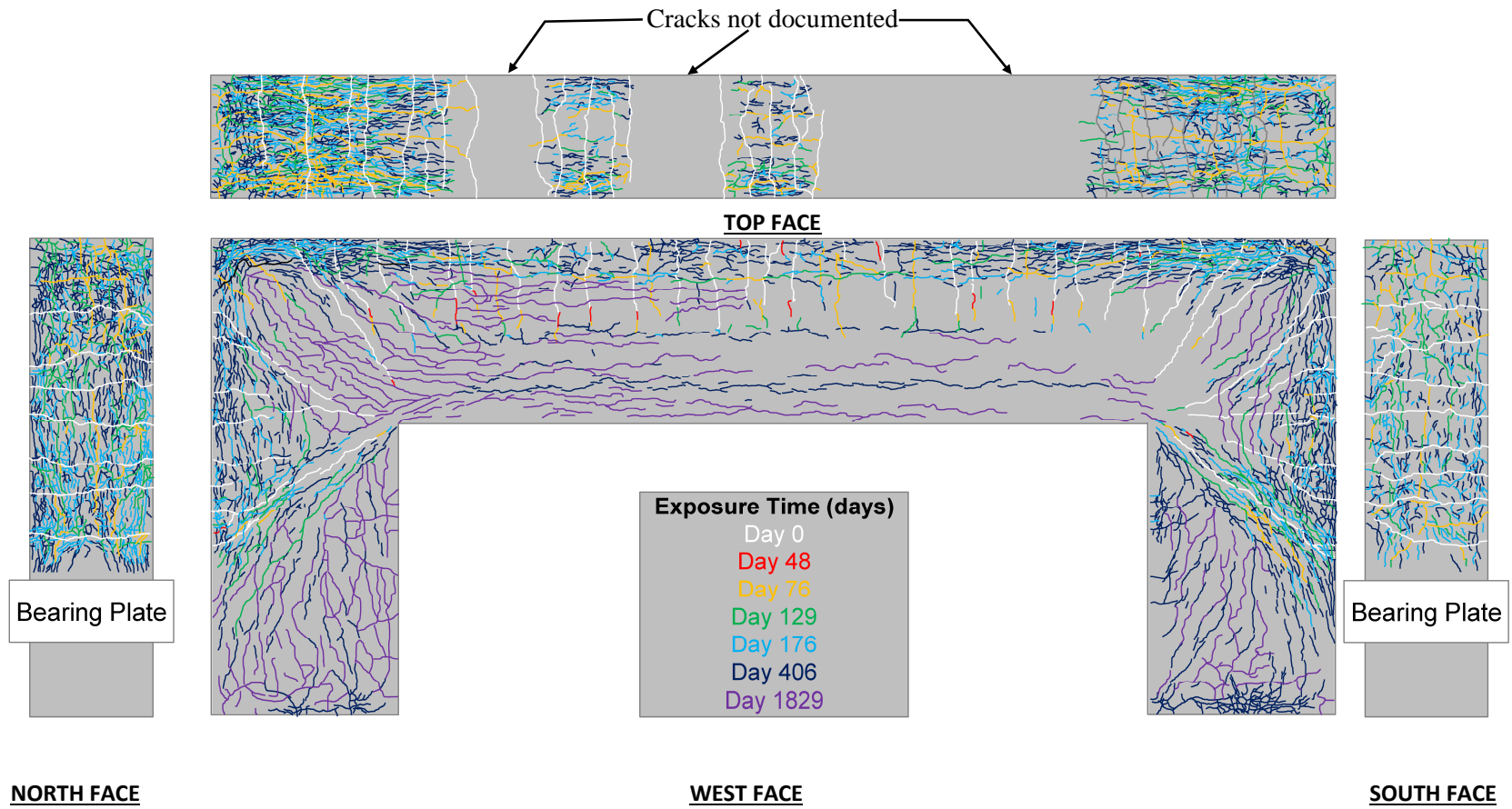
Figure 4-2: Crack Pattern over Time in Specimen 3.
