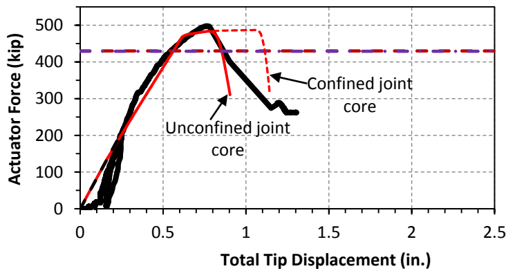
Figure 7-7: Comparison of Experimental and C-STM Results for C-Beam Specimens Subjected to ASR/DEF Deterioration.
