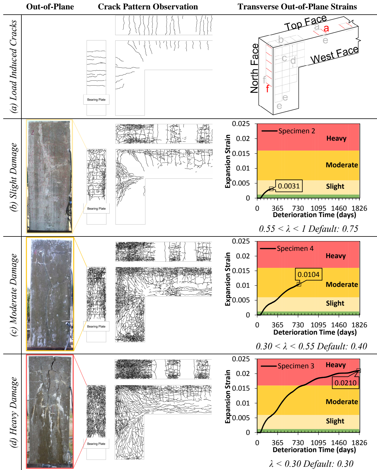
Figure 7-2: Deteriorated Specimen Appearance, and the Modeled Transverse Strains in the C-Beam Out-of-Plane Direction.
