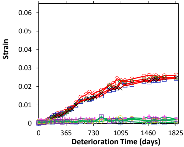
(c) DEMEC Strains in Member
