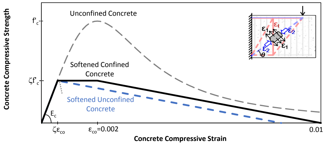
(b) Compression Softened Concrete Model
