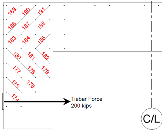
(a) DEMEC Layout Transverse to Diagonal Strut in Beam and Joint Region
