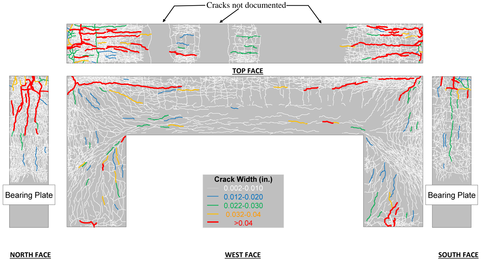
Figure 4-3: Final Crack Widths on Specimen 3.
