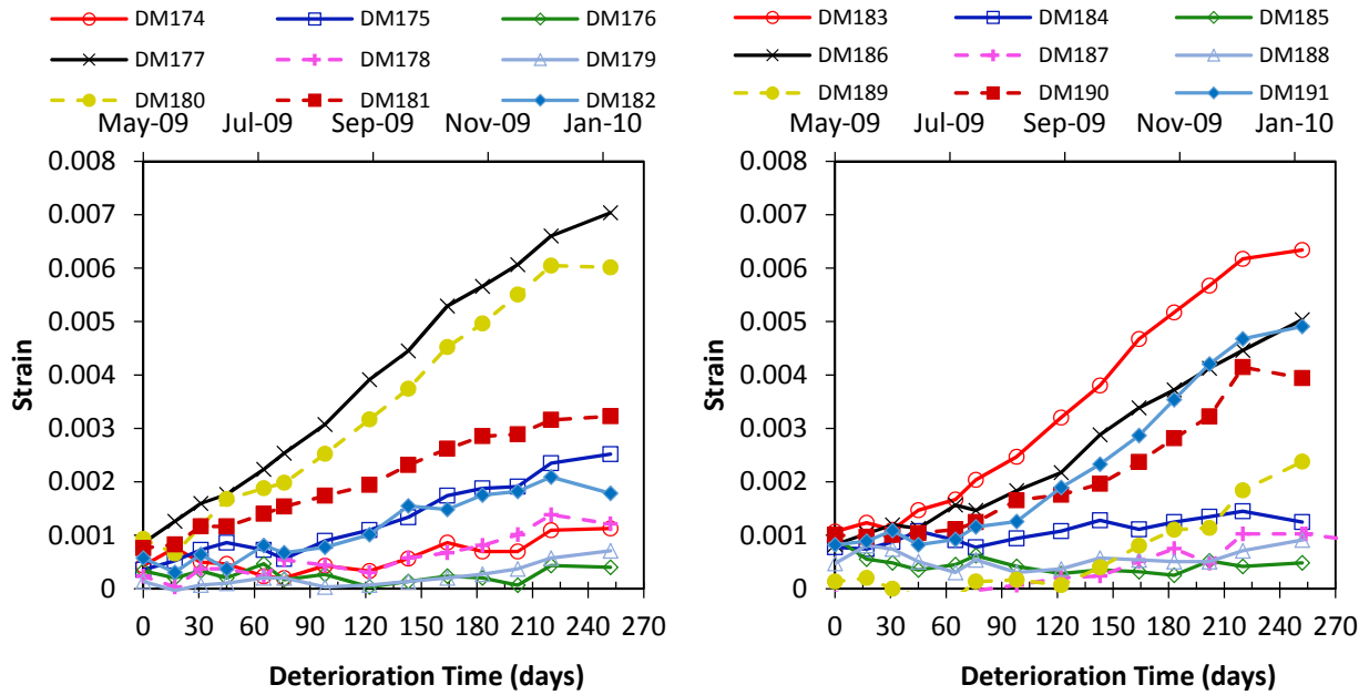
(b) Strains Transverse to Main Diagonal Strut in Beam
