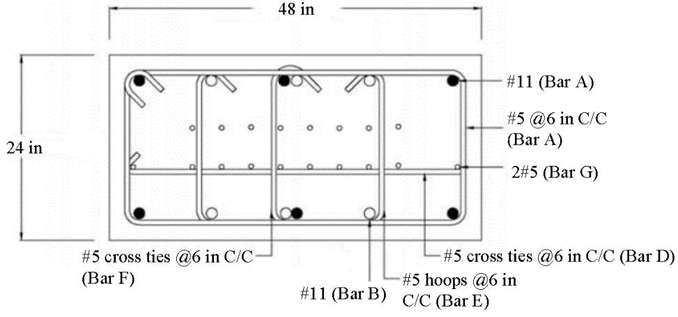
(c) Section B—B: End Region
