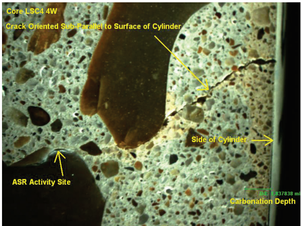
Image illustrating carbonation depth on side of cylinder (1.84 mm)
