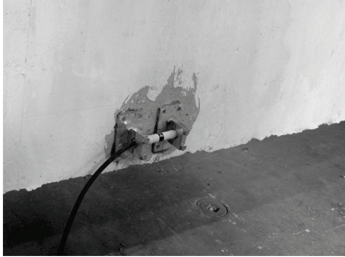
Figure 4-11. KM Gage Installation prior to Testing.
