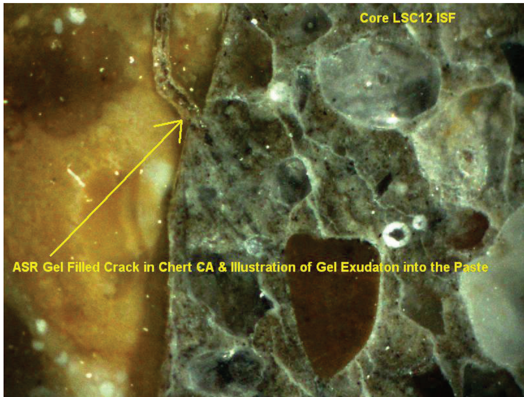
Optical image illustrating ASR activity
