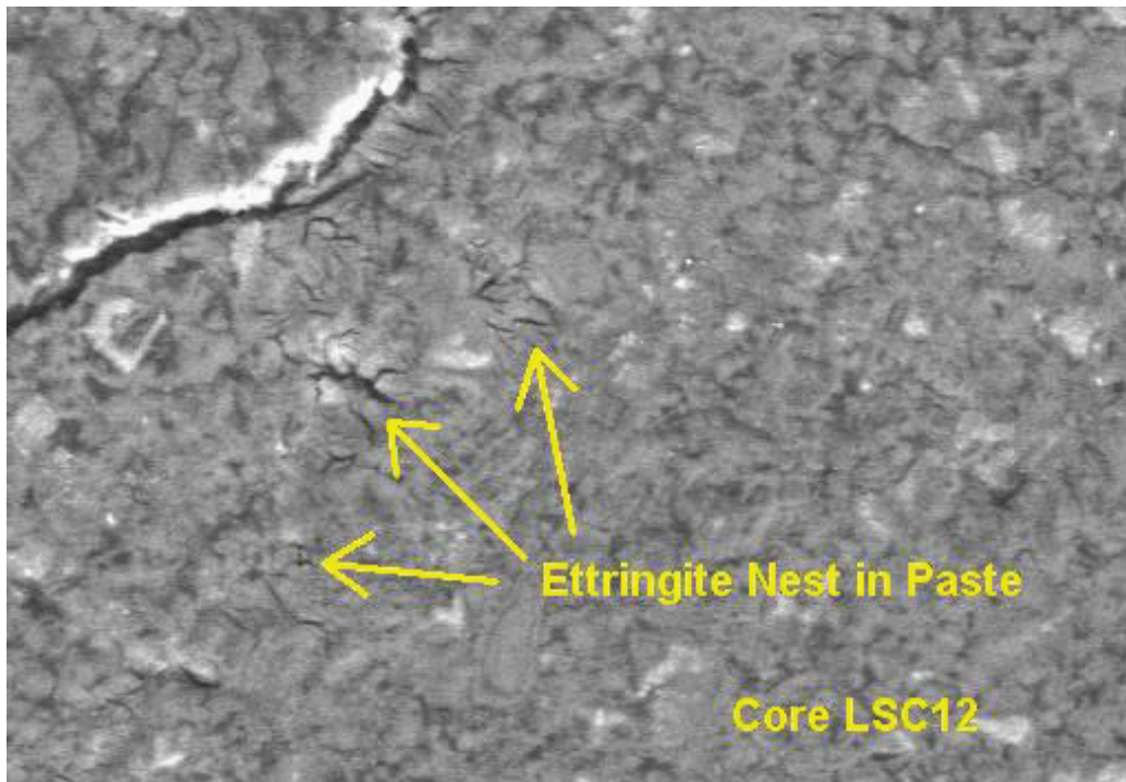
BSE image illustrating ettringite nest in the paste of core LSC12 ISF
