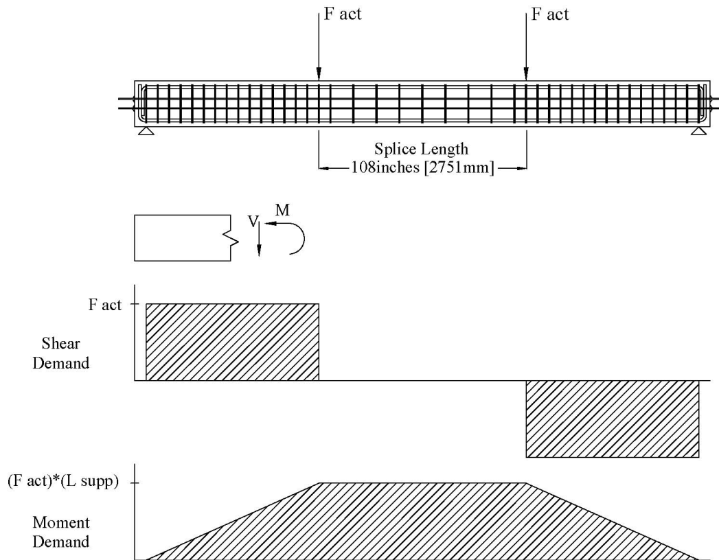
Figure 4-4. Four-Point Load Test Setup and Demand Loading.
