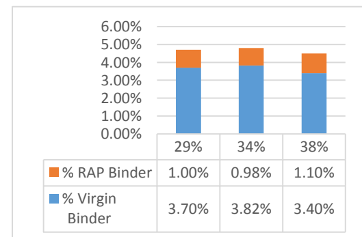
(f) Optimum Asphalt Content
