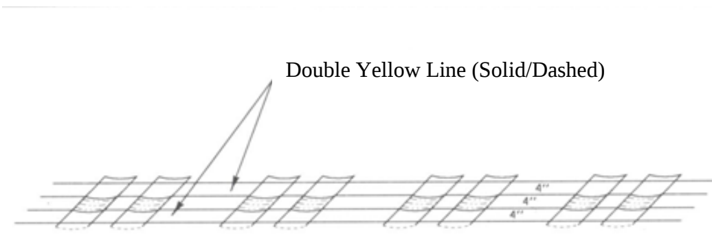
Figure 3: Rumble stripe design.
