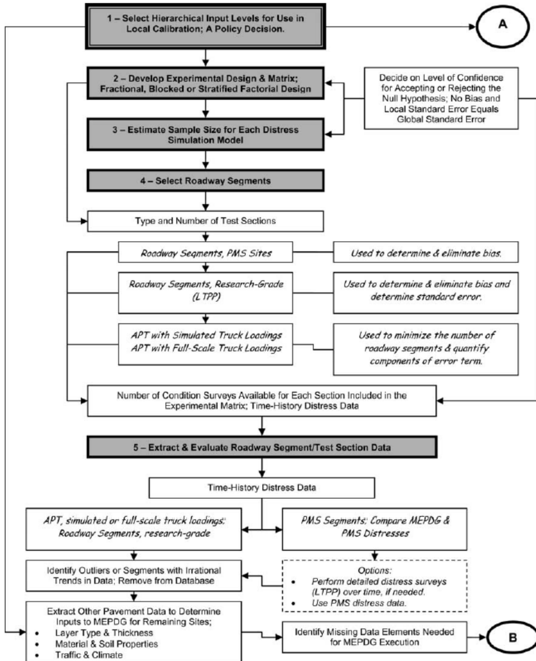
Figure 3.1 Local Calibration Process, Part 1 (NCHRP 2009)
