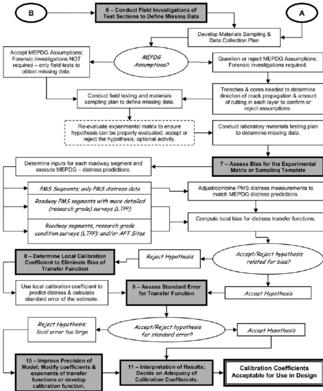
Figure 3.2 Local Calibration Process, Part 2 (NCHRP 2009)
