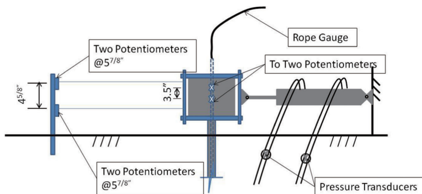
Figure E-1.1 Bridge displacement monitoring locations with potentiometers.
