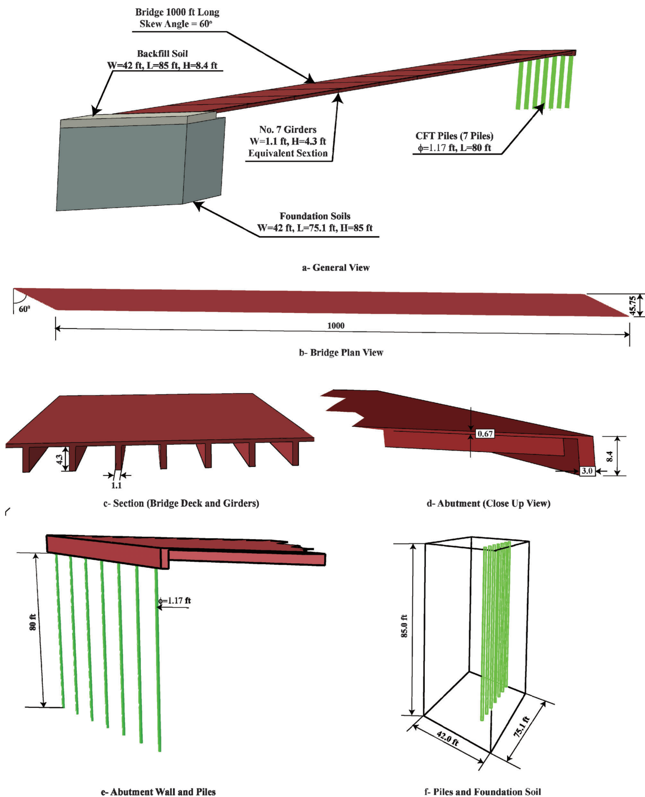
Figure F.4 Numerical model dimensions.
