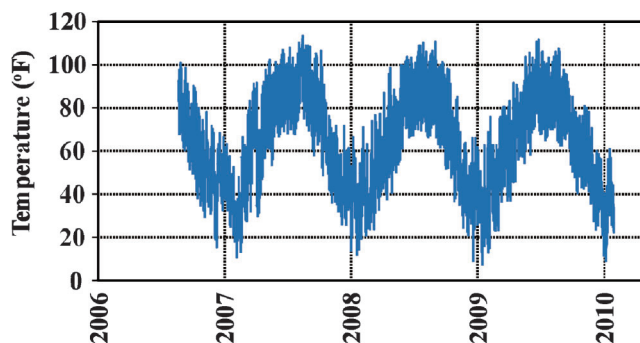
Figure E.21 Recorded temperature at US 231 bridge's deck (Frosch & Lovell, 2011).
