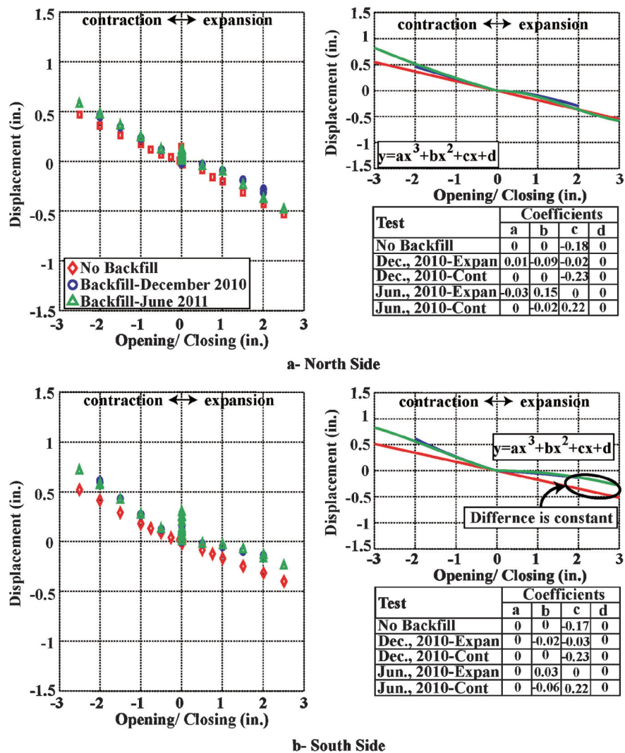
Figure B.47 Bridge deck rigid body transverse movement.
