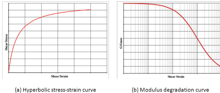
Figure D.1 Schematic of a modified hyperbolic stress-strain relationship and associated modulus degradation curve.
