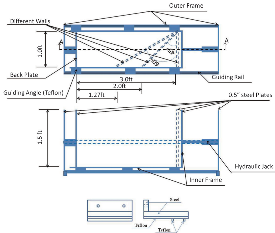
Angle Detail
