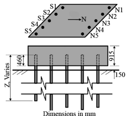
Figure B.3 Piles configuration and depth. (After Frosch and Lovell, 2011.)
