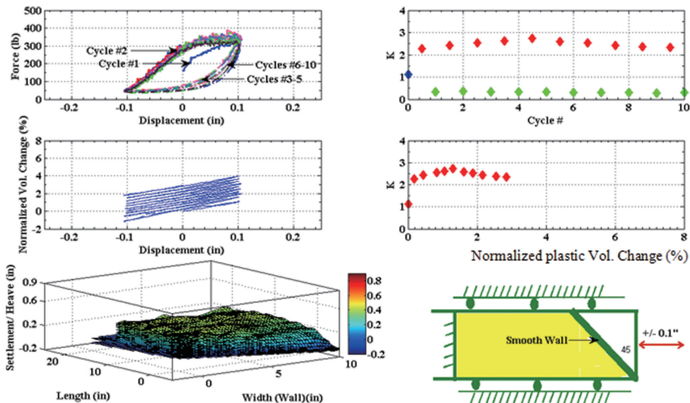
Figure C-1.8 Summary plot for Test #8.
