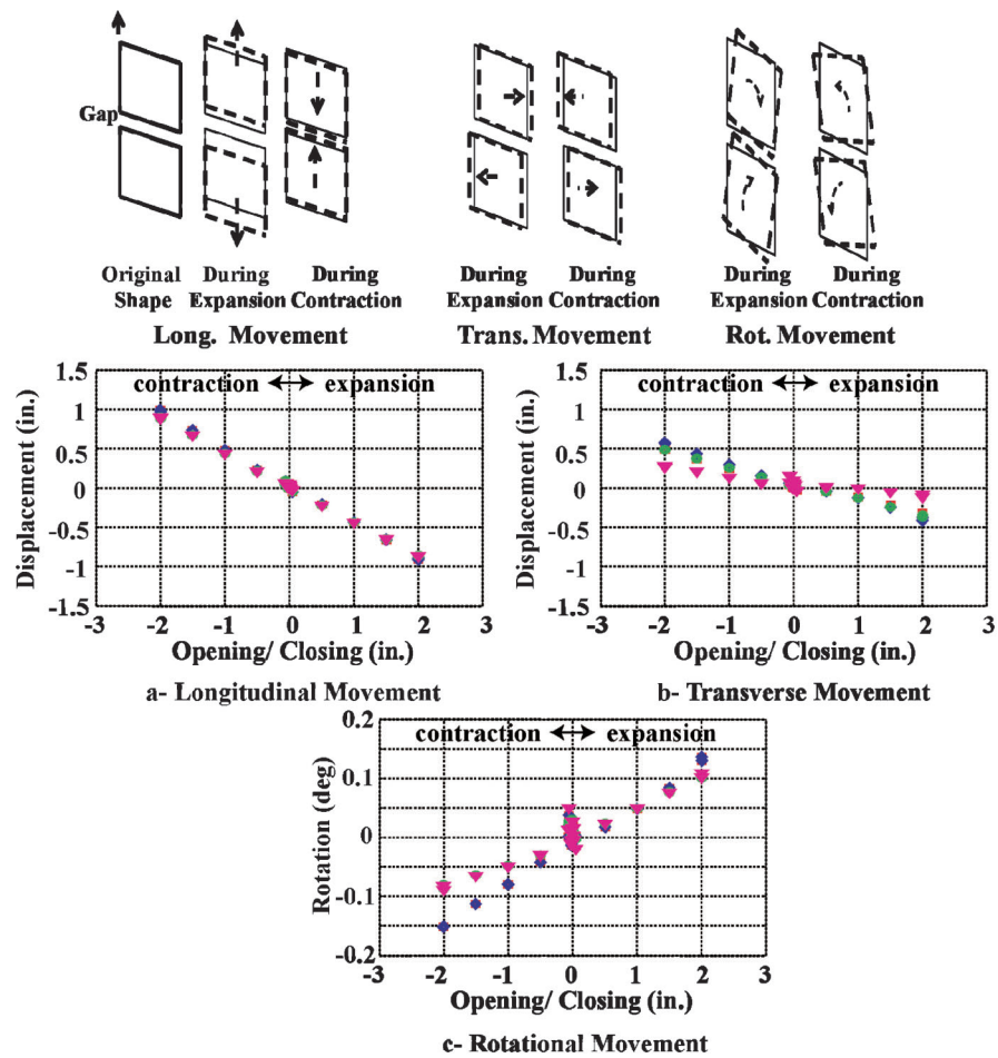
Figure B.22 North side rigid body movement.
