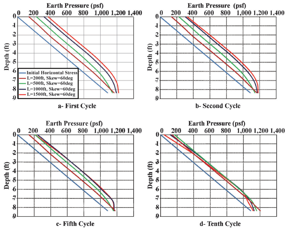
Figure F.16 Effect of bridge length—soil pressure along a vertical section at the center of the abutment.
