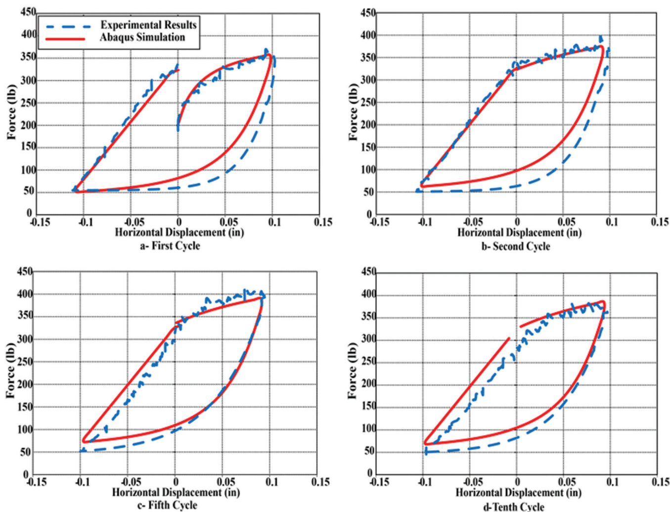
Figure E.5 Force versus displacement comparison—zero degree (0°), smooth wall case (Test 2).
