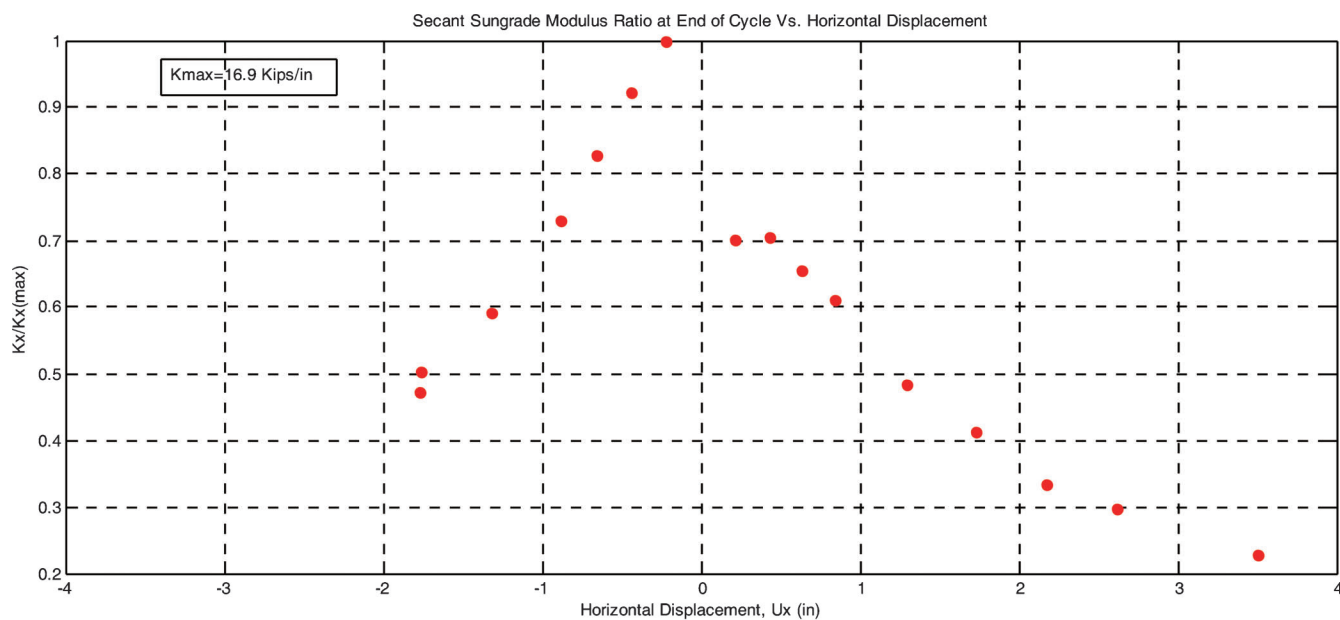
Figure E-1.7 Secant modulus as a function of displacement.
