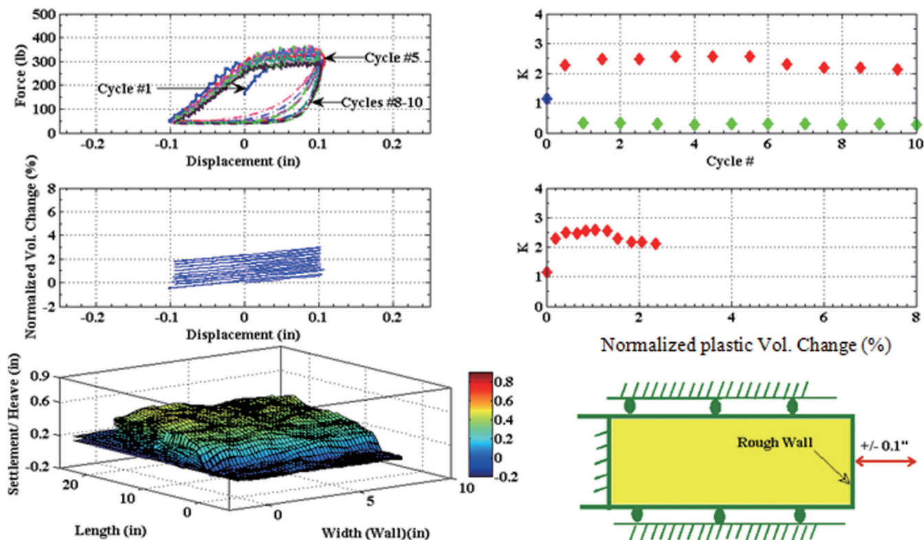
Figure C-1.9 Summary plot for Test #9.
