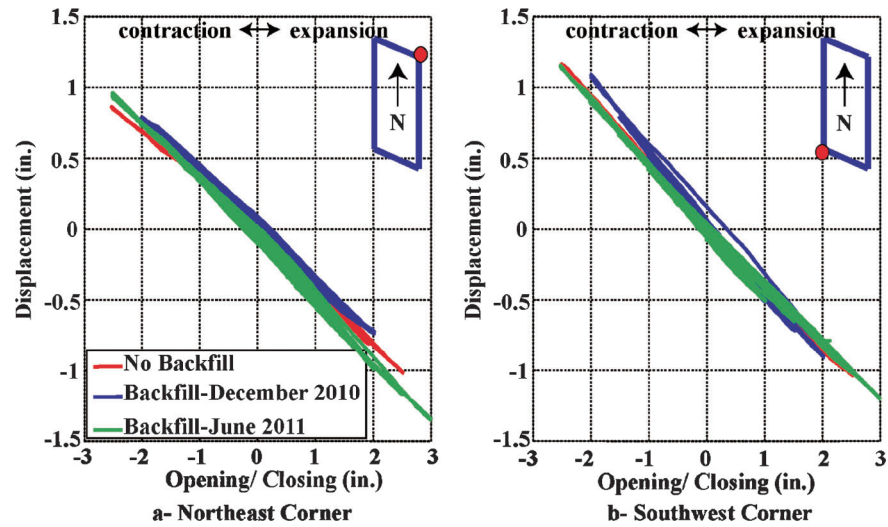
Figure B.44 Obtuse corners hysteresis of longitudinal displacements.
