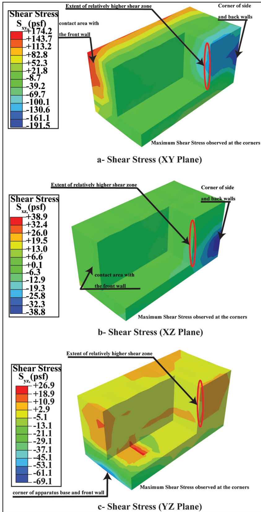
Figure C.5 Shear stress (in psf) distribution in the sand specimen.
