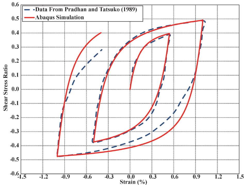
Figure E.2 Comparison of the stress-strain relationship—laboratory cyclic direct simple shear.
