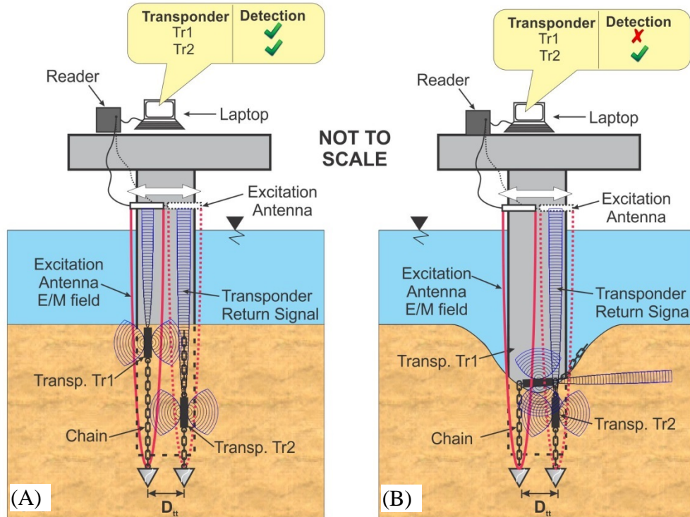
Figure 5. Application of the RFID technology for measuring scour via the transponder orientation: (A) prior to the occurrence of scour, and (B) after the occurrence of scour.
