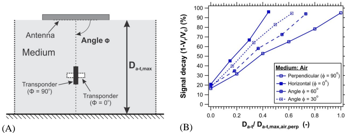
Figure 7. (A) Inclination angle, \phi , between the transponder antenna axis and the excitation antenna plane, (B) Dependence of the transponder signal strength decay on \phi .
