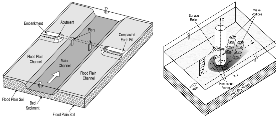
Figure 1. Flow through a bridge site produces complex interactions between the flowing water, bed sediment, and bridge pier causing hydraulic erosion and scour. These sketches illustrate some of these flow complexities around an abutment or pier.
