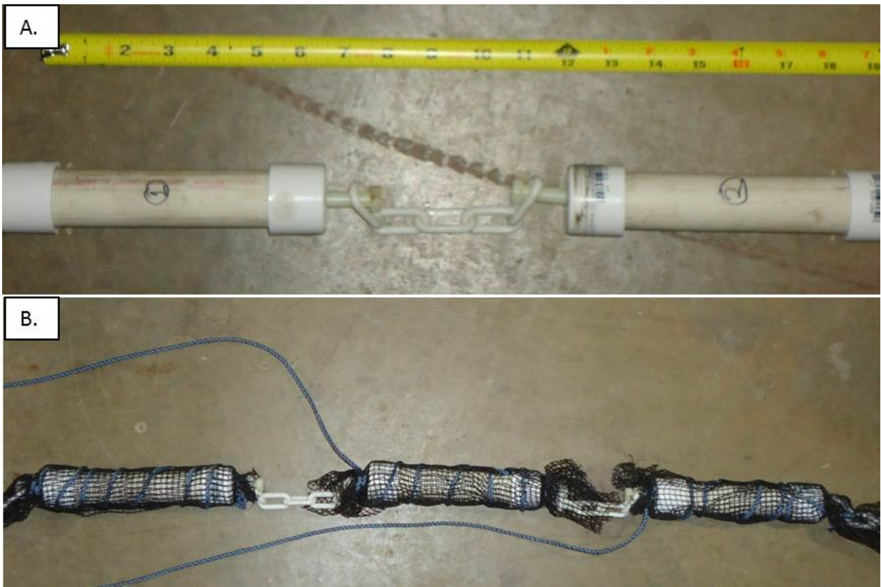
Figure 13. Leopold Chain. (A) A close-up image of the Leopold chain with two encased transponders and a plastic chain to minimize interference; and (B) The encased transponders were also placed in a is before the fishing net and secured with paracord were added.
