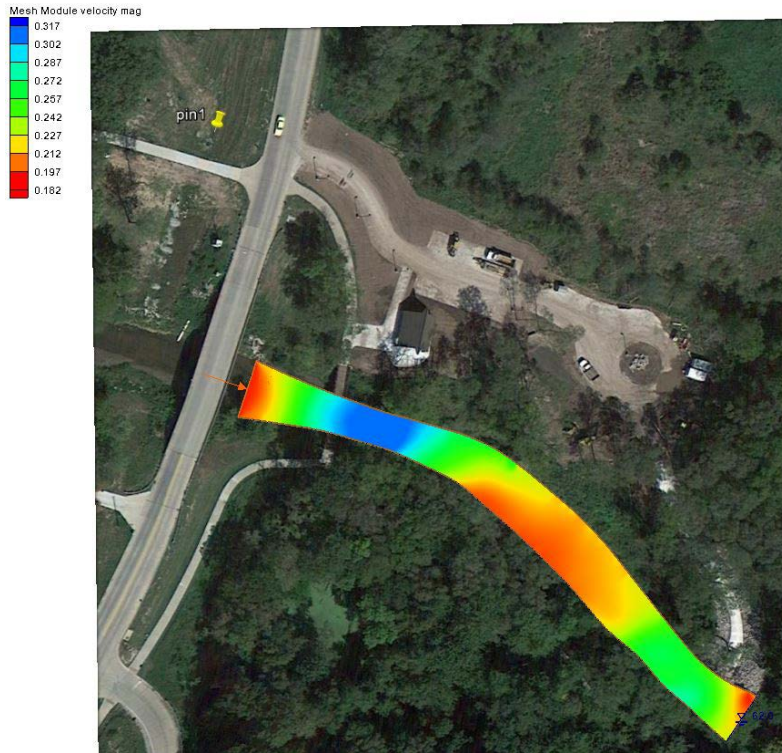
Figure 22. FESWMS simulation. The velocity flow field for Clear Creek near Camp Cardinal developed using FESWMS and the sonar-measured bathymetry data. Blue colors represent faster velocities and red colors represent slower velocities.
