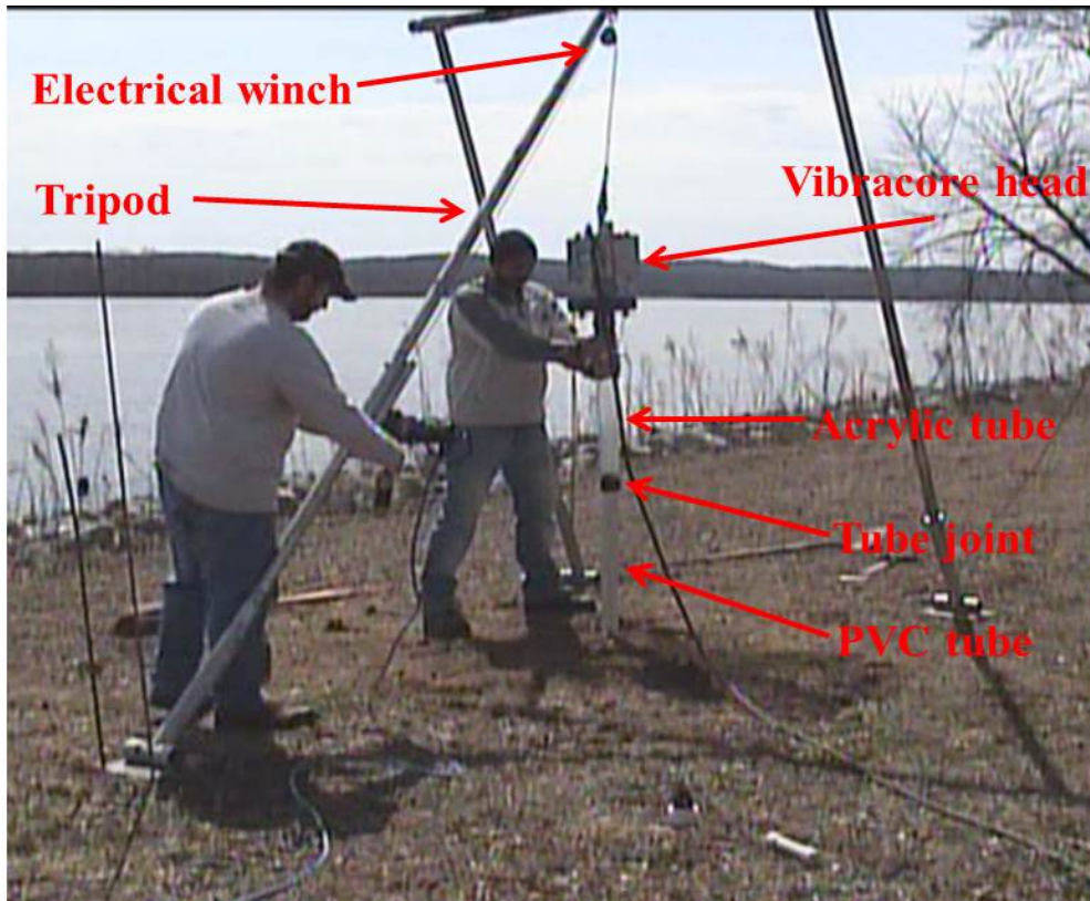
Figure 18. Vibracore drill components and field setup. The field installation process of the transponders shows the vibracore being driven into the sediment.
