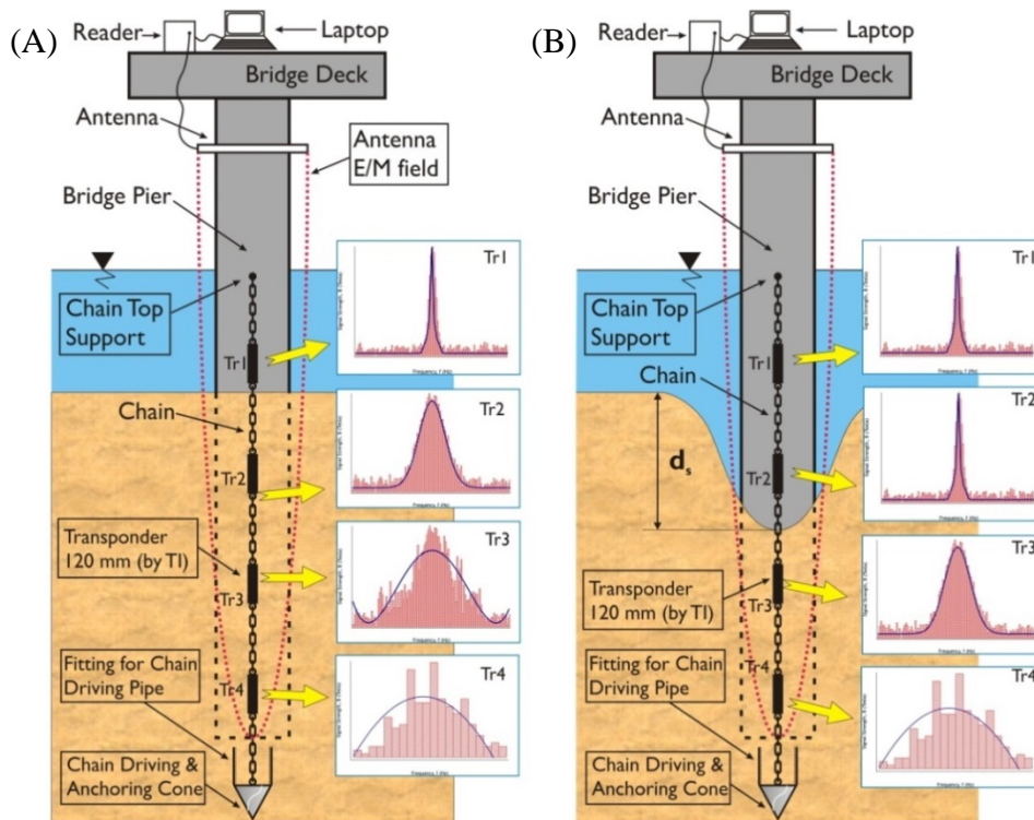
Figure 10. Detection of the scour depth using the “signal strength” approach. (A) No scour. (B) Scour
