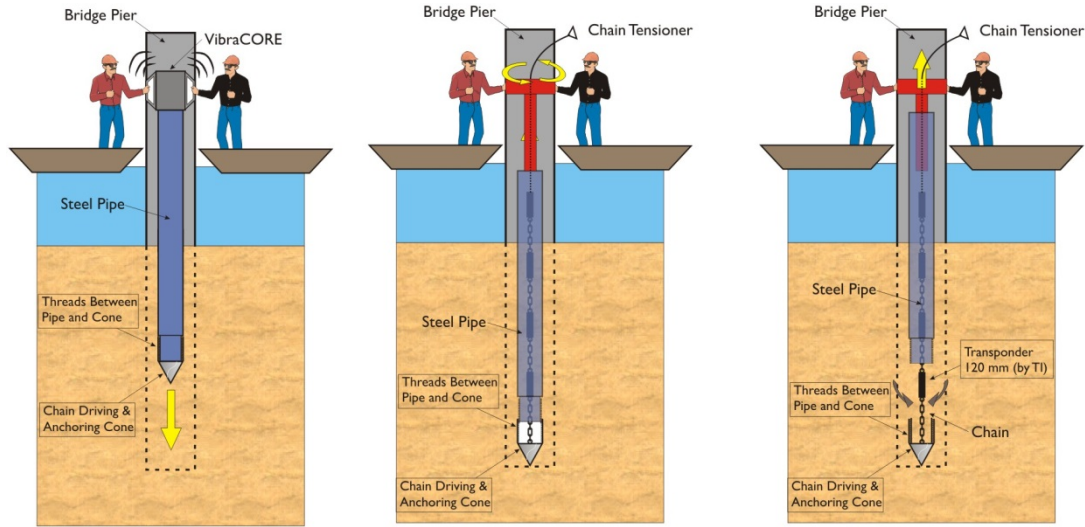
Figure 8. The pile/chain driving mechanism with vibracoring. Transponders are mounted to the chain at predetermined distance.
