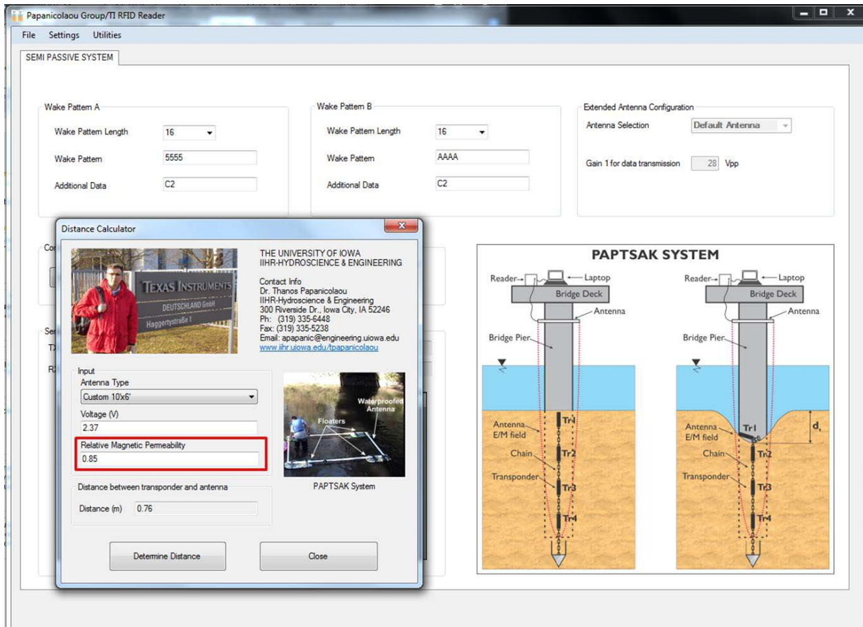
Figure 21. Screen shot of the PAPTSAK RFID software “Distance Calculator”. The user can insert the relative magnetic permeability of the medium or mixture of mediums in between the excitation and the transponder miniature antennas, as well as to select the excitation antenna type from the drop down menu.
