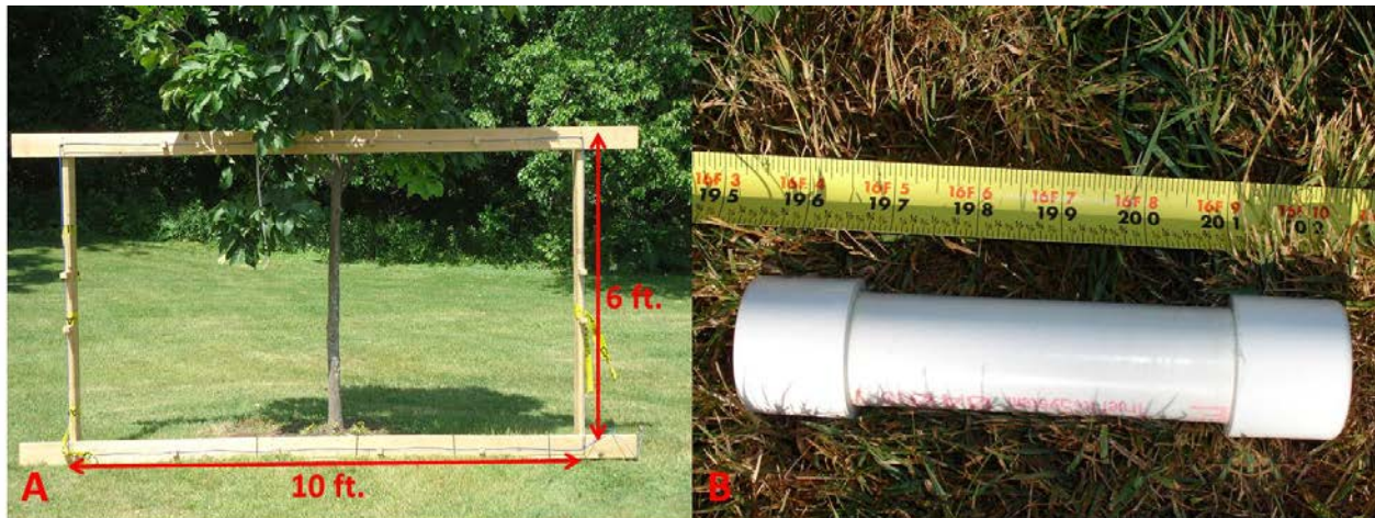
Figure 6. (a) Custom-made excitation antenna and (b) PVC-encased transponder.
