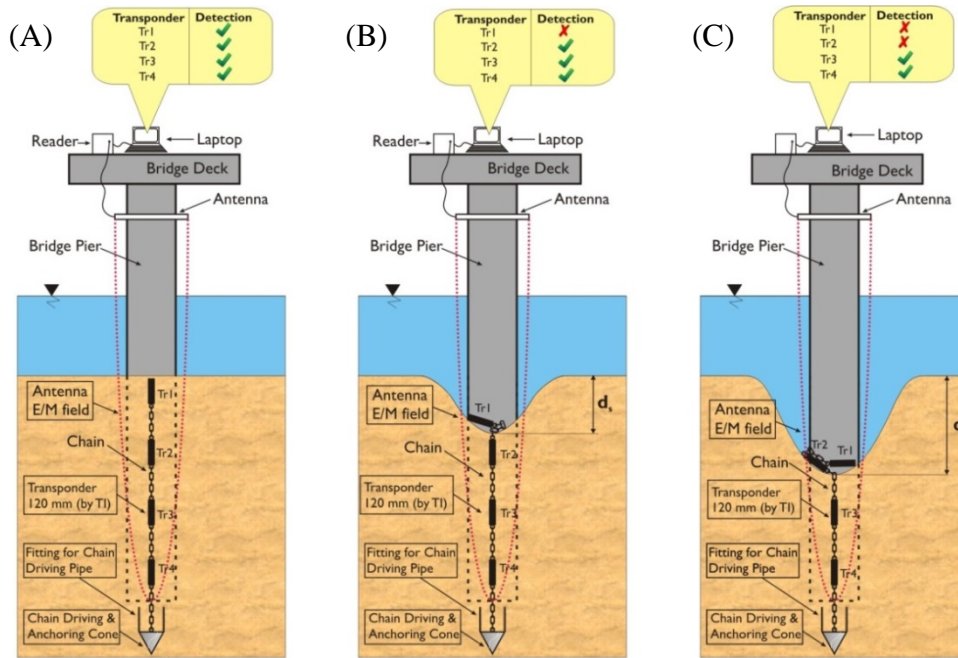
Figure 9. Detection of the scour depth using the “folding chain” approach. (A) No scour. (B) Scour exposes transponder Tr1. (C) Scour increases and exposes transponders Tr1 and Tra2
