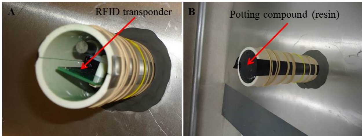
Figure 12. Encapsulating the transponder. (A) The transponder was carefully placed into a mold and potting compound was added to encapsulate the transponder circuitry; and (B) The transponder is fully covered, or encapsulated, into the potting compound.
