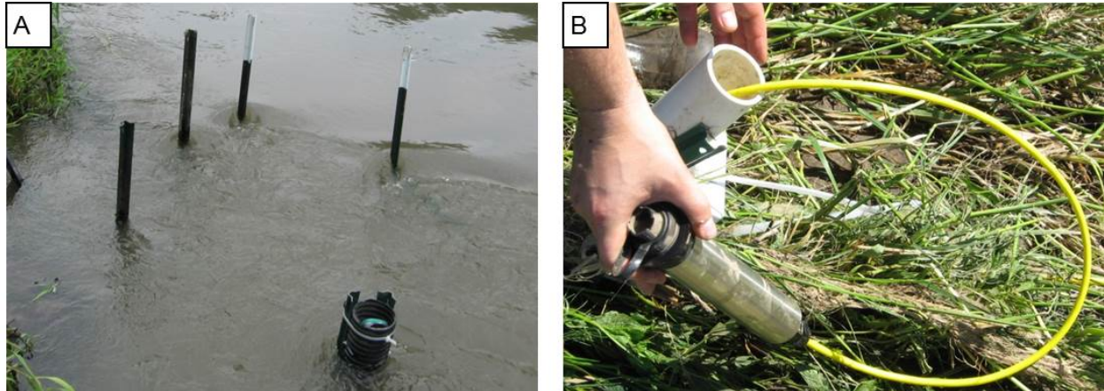
Figure 14. Pressure Transducer. (A) The pressure transducer was installed in stilling well in Clear Creek near Camp Cardinal, IA site; and (B) The datalogger of the pressure transducer was secured on the bank.
