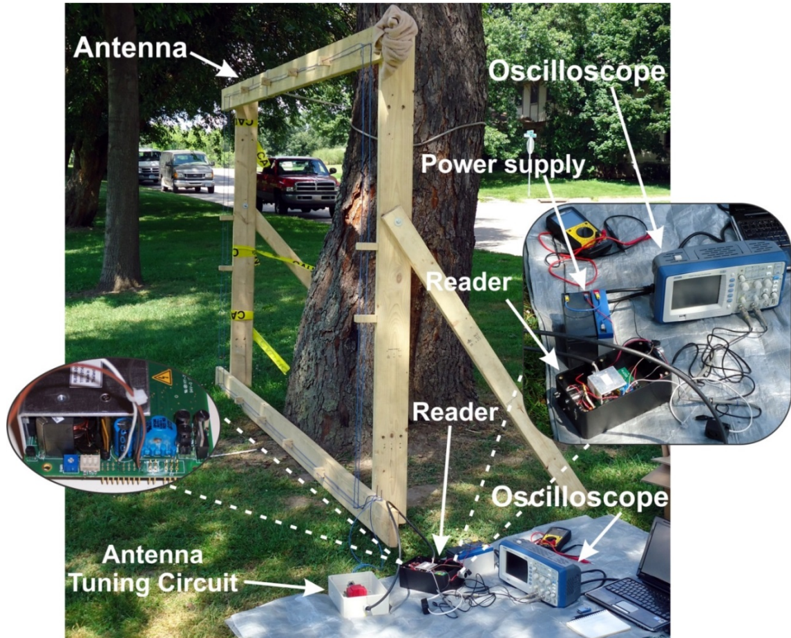
Figure 3. Setup of the Low Frequency, passive RFID system used in this study with the custom antenna.
