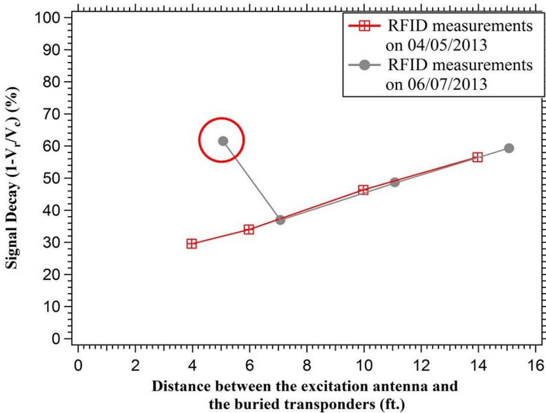
Figure 20. Processed RF signal strength decay curves corresponding to the two measurement dates during the period of 04/05/2013 and 06/07/2013.
