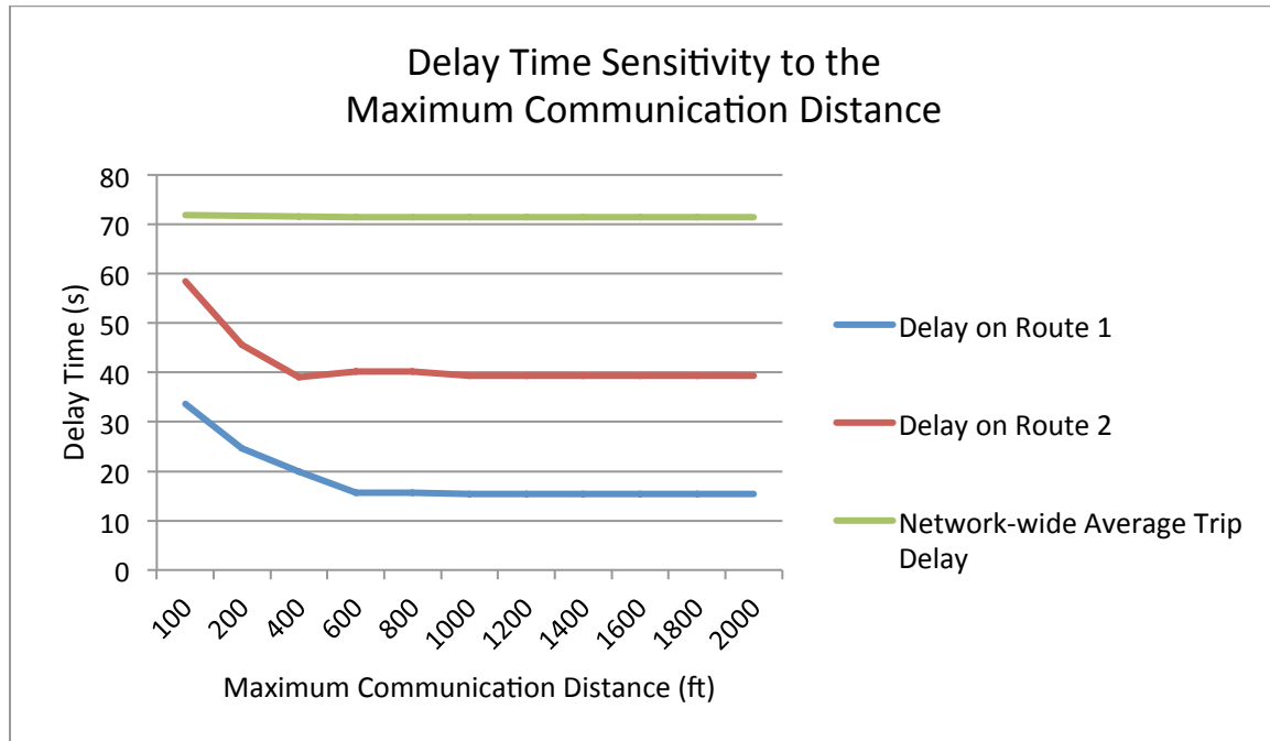
Figure 16. Bus Travel Time under Different Maximum Communication Distances
