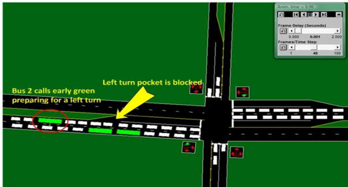
Figure 19. TSP Strategy Update from Early Green to Early Green
