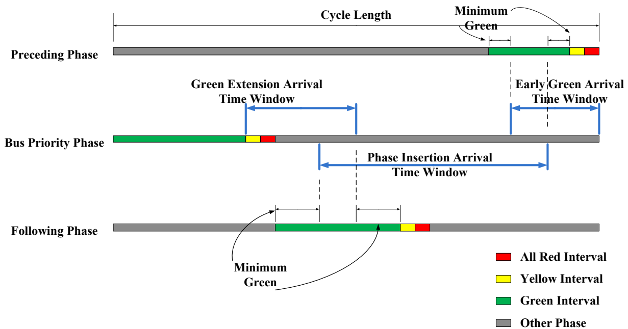
Figure 3. Time Window for Transit Signal Priority Request
