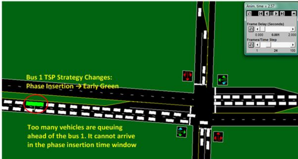
Figure 17. TSP Strategy Update from Phase Insertion to Early Green
