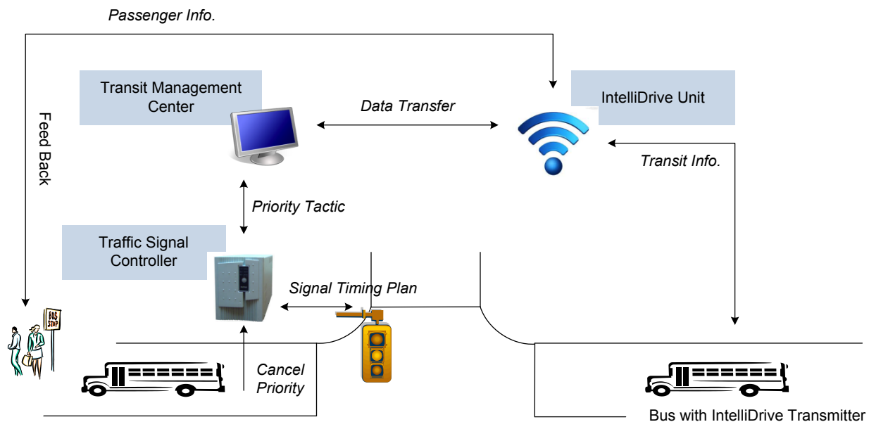
Figure 2. Coordination of TSP and IntelliDrive
