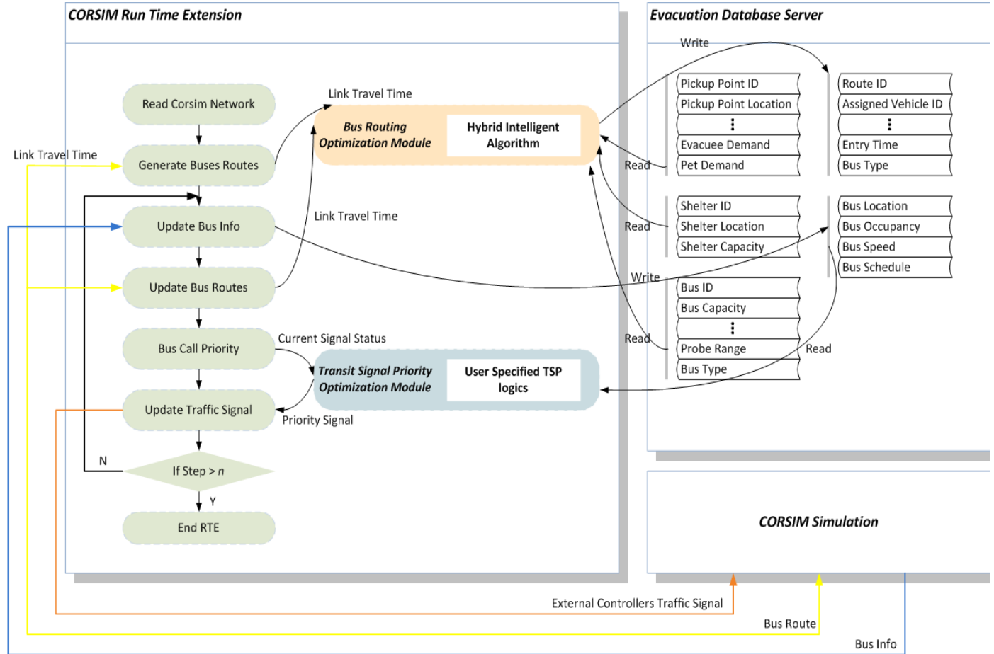
Figure 7. Flowchart of TSP System Implementation
