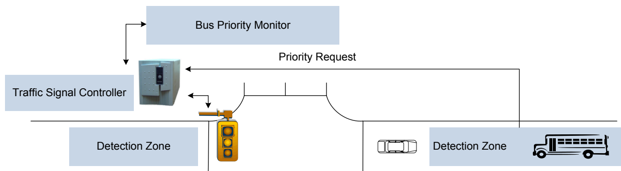
Figure 1. Transit Priority at Traffic Signalized Intersections
