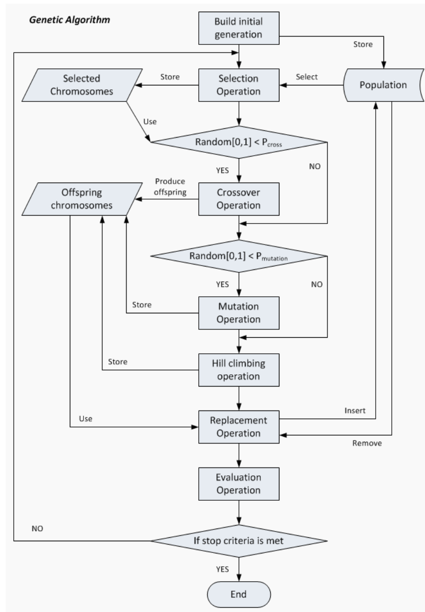
Figure 4. Flowchart of the Proposed HIA
