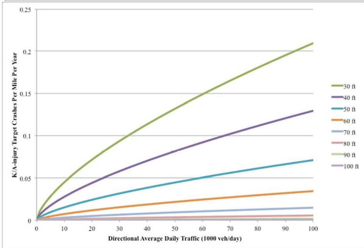
Figure 24. Predicted Number of Target Crashes by Severity Level (PDO/C and K/A) Based upon Directional Average Daily Traffic and Median Width
