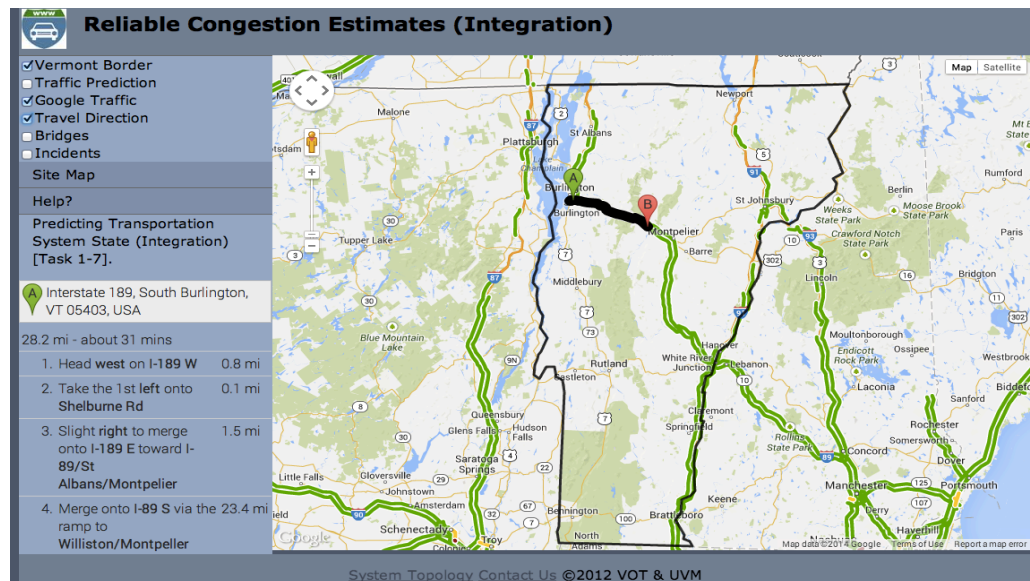
Figure 4.13: Route Planning
