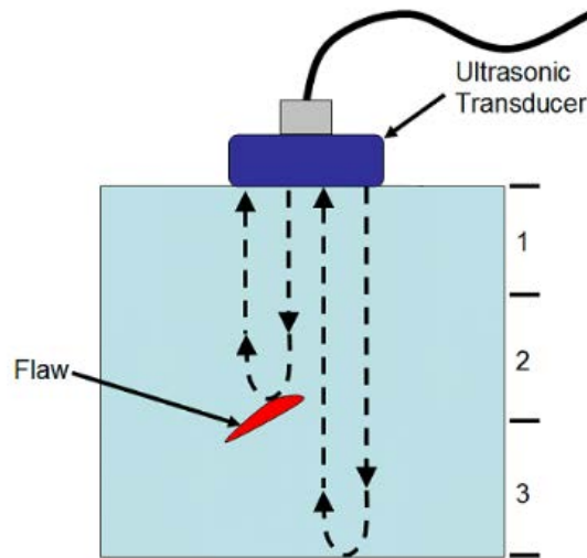
Figure 7. Pulse-Echo Technique
