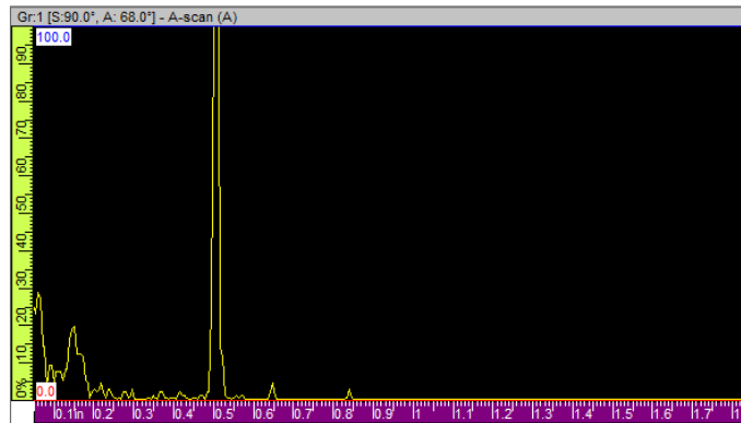
Figure 10. A-Scan Representation of a Half-Inch Flaw
