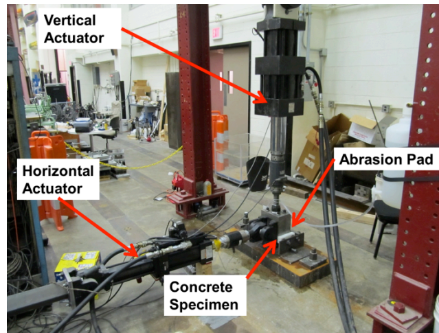
Figure 2.1. Large-Scale Abrasion Test Setup.
