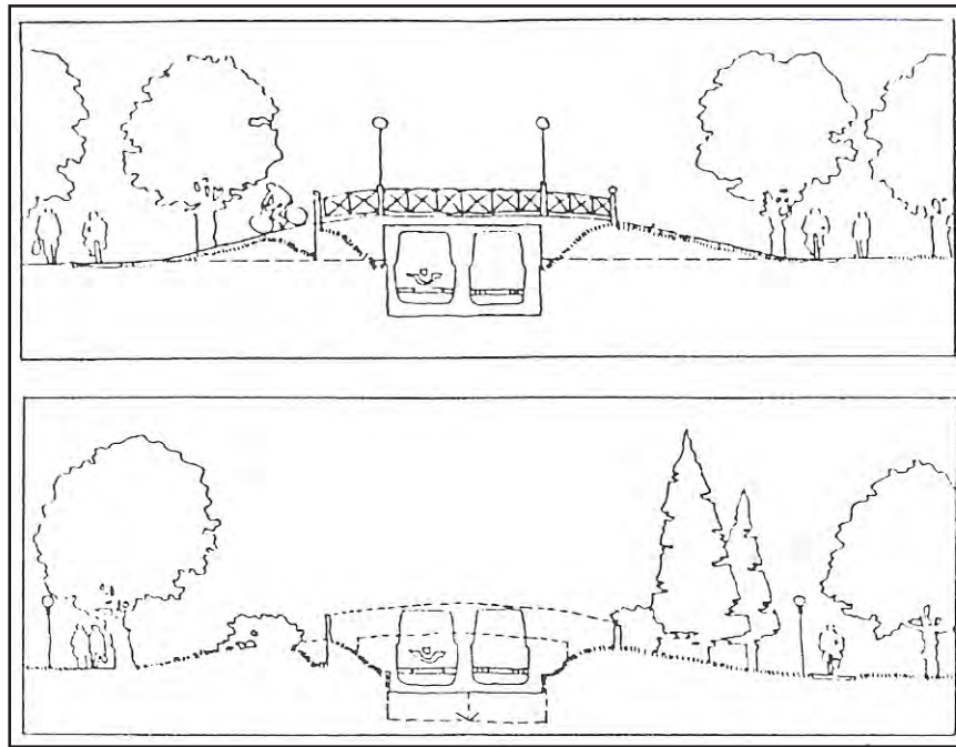
Figure 14. Near-grade Guideway Placement
