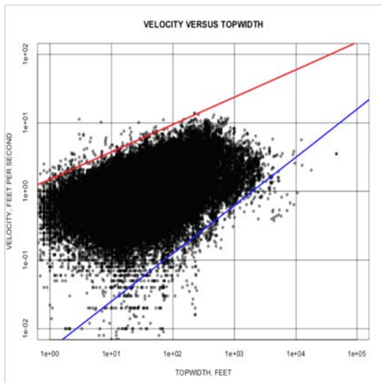
Figure 1. Velocity-Topwidth Relation for Texas.
