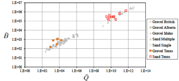
Figure 2. Dimensionless Discharge and Topwidth for Texas Streams.
