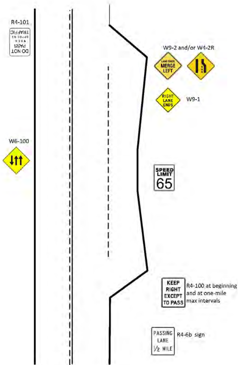
Figure 8. Schematic view of Scenario 6 – Passive speed reduction with lane narrowing (geometry not to scale).
