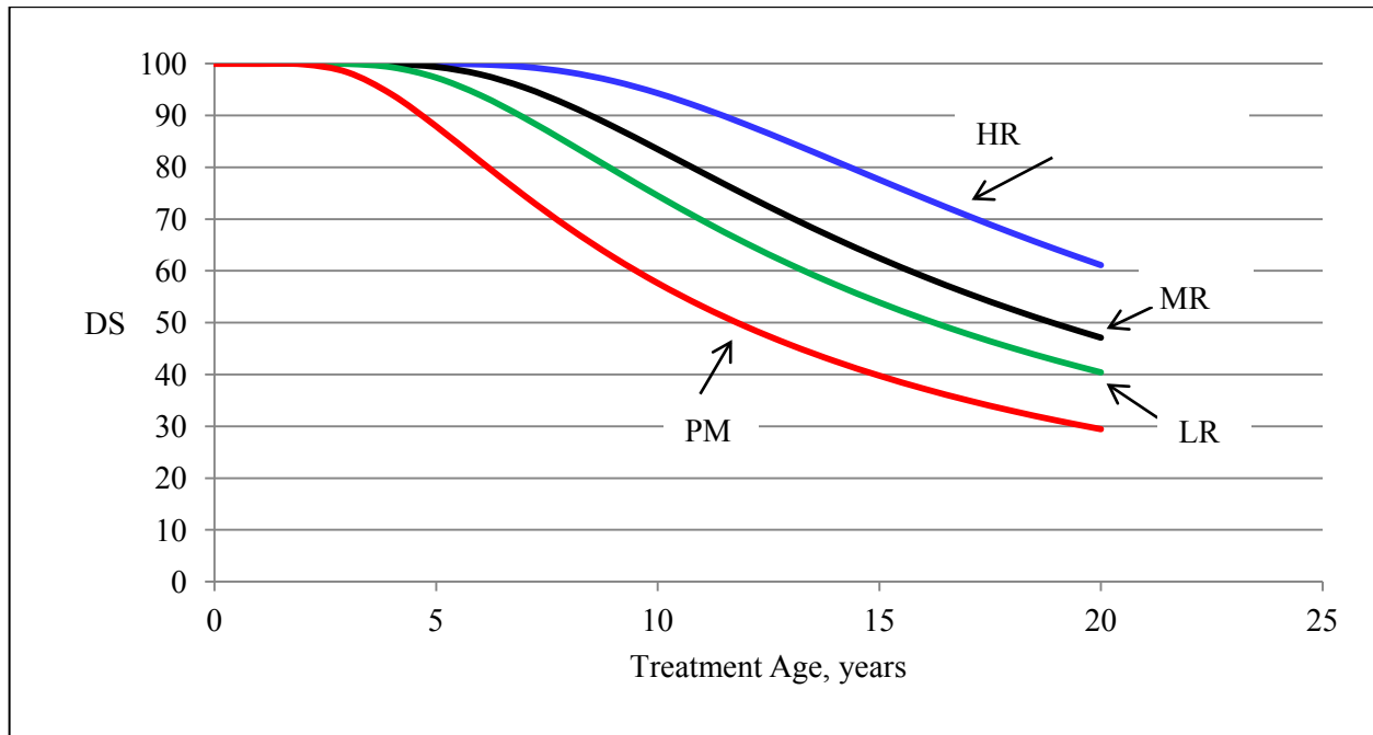
Figure 39. Example DS Prediction Models (Pavement A, Zone 2, and Medium Traffic Loading).
