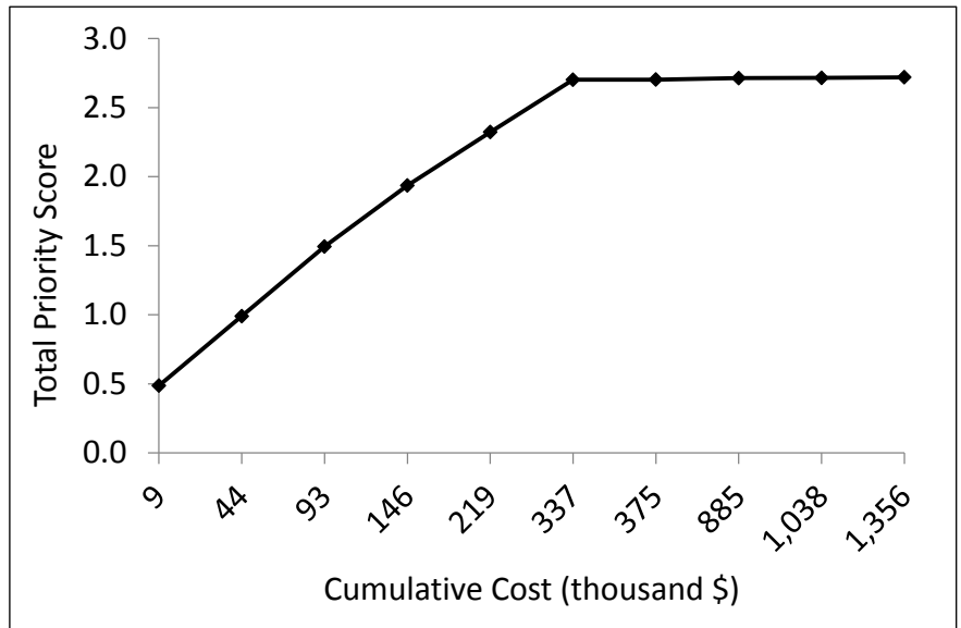
Figure 48. Maximization of the Total Priority Score Using the IBC Algorithm.
