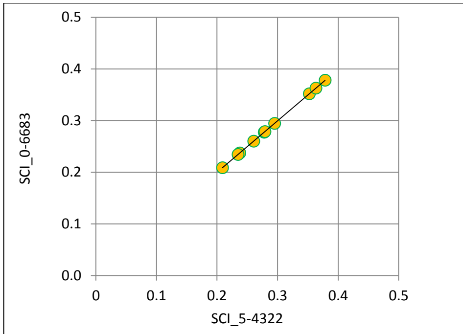
Figure B2. SCI values Computed Using Original Procedure (Developed under Project 5-4322) and Replicated Procedure (Replicated under This Study).
