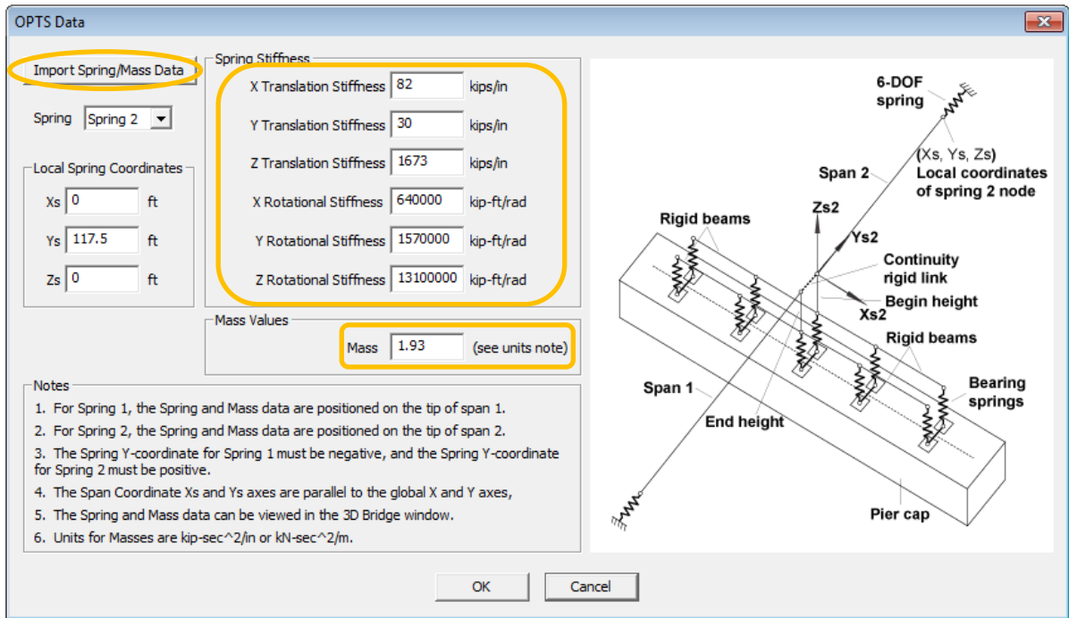
Figure 3.209 Iteration 2 OPTS spring stiffnesses and mass
