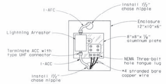
ARRESTOR ENCLOSURE DETAIL NO SCALE
