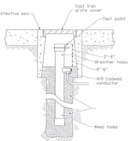
GROUND ROD DETAIL NO SCALE
