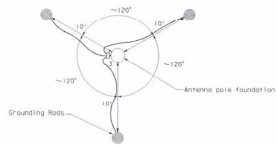
LAYOUT FOR GROUNDING RODS NO SCALE
