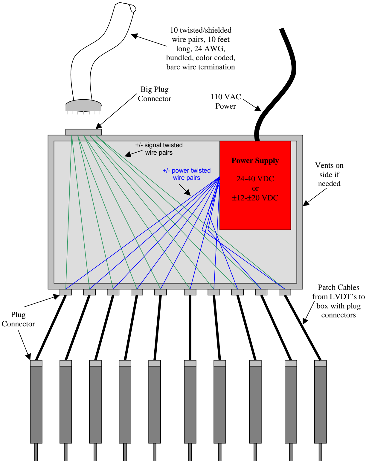
Figure C-17: LVDT Breakout Box Schematic
