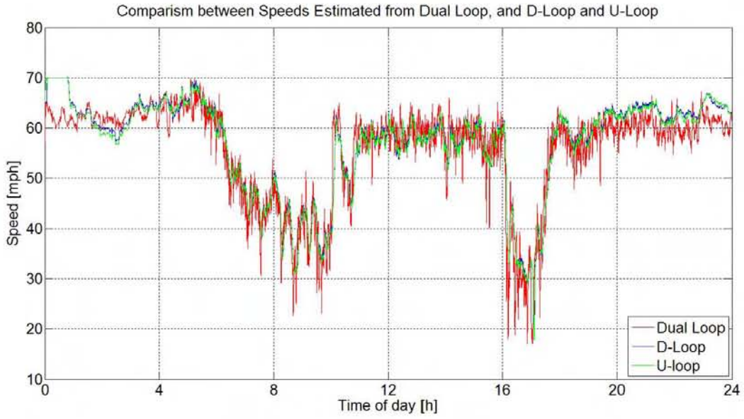
Figure B. 34 BHL WB, Station 2, Lane 4, Speed estimation comparison
