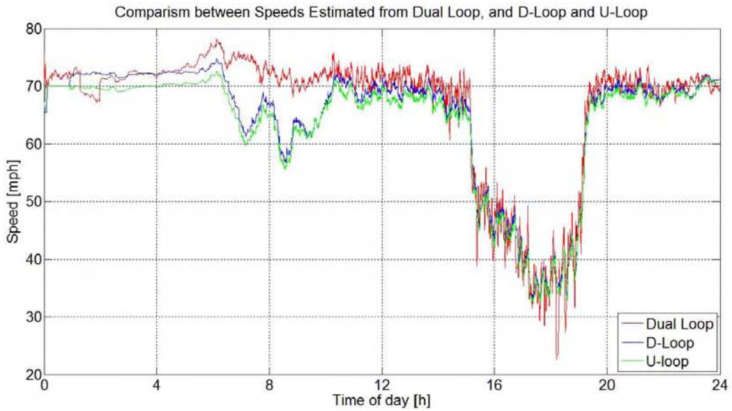
Figure B. 56 BHL EB, Station 7, Lane 1, Speed estimation comparison
