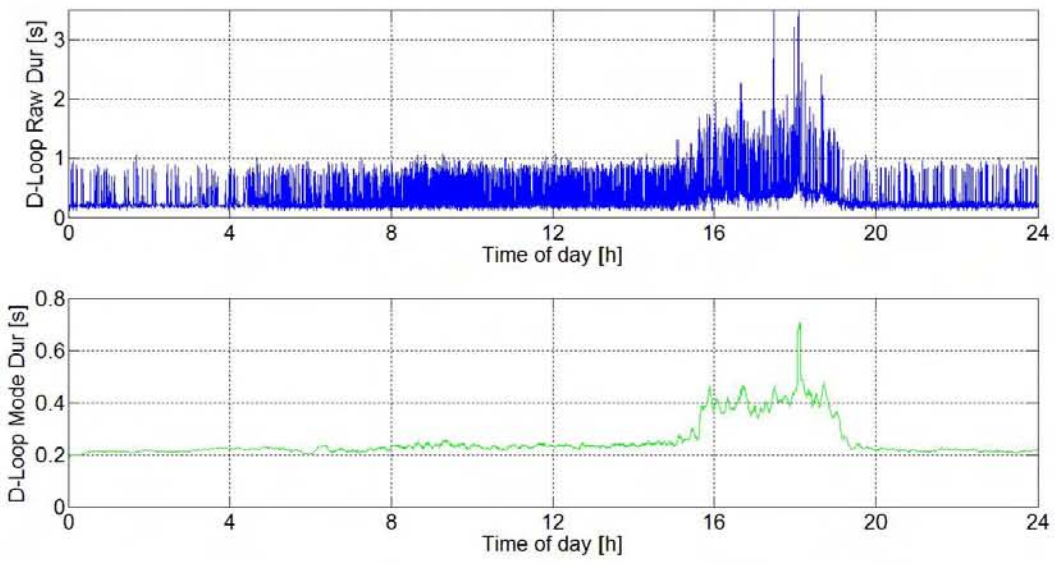
Figure B. 10 BHL EB, Station 1, Lane 3, Raw and Mode Durations: D-loop
