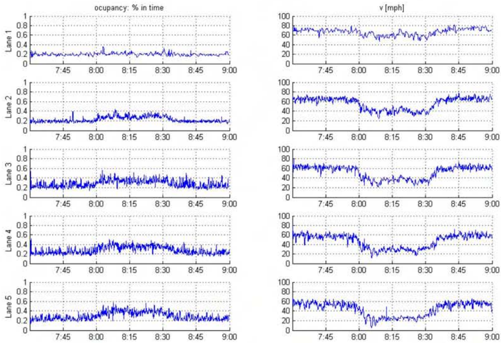
Figure 5.1. Occupancy and speed estimation at loop Station 4 and Station 6 on 07/01/2007
