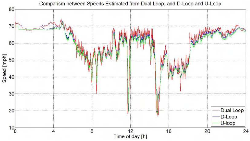
Figure 3.5. BHL data on 03/01/2011, St-7 WB Lane 1: estimated speed comparison
