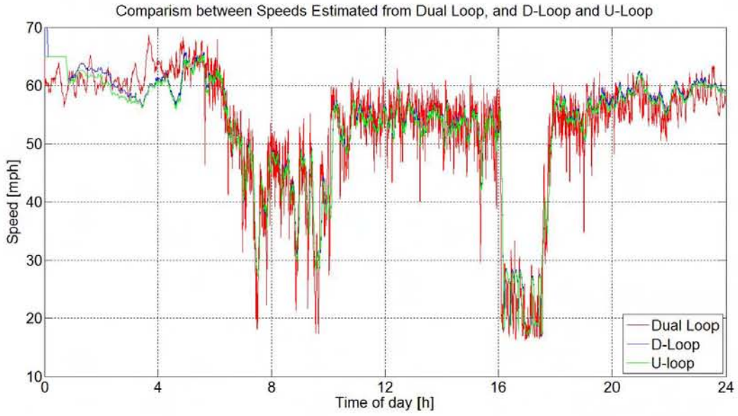
Figure B. 45 BHL WB, Station 3, Lane 5, Speed estimation comparison ***** *****
