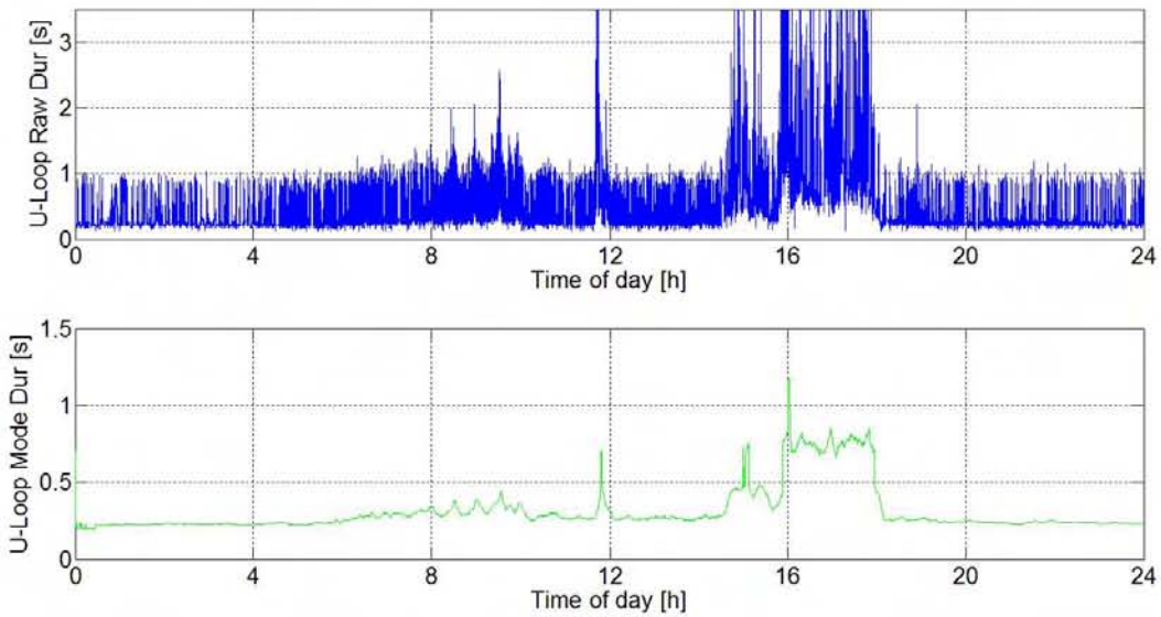
Figure 3.3. BHL data on 03/01/2011, St-7 WB Lane 3 U-loop: raw and mode durations
