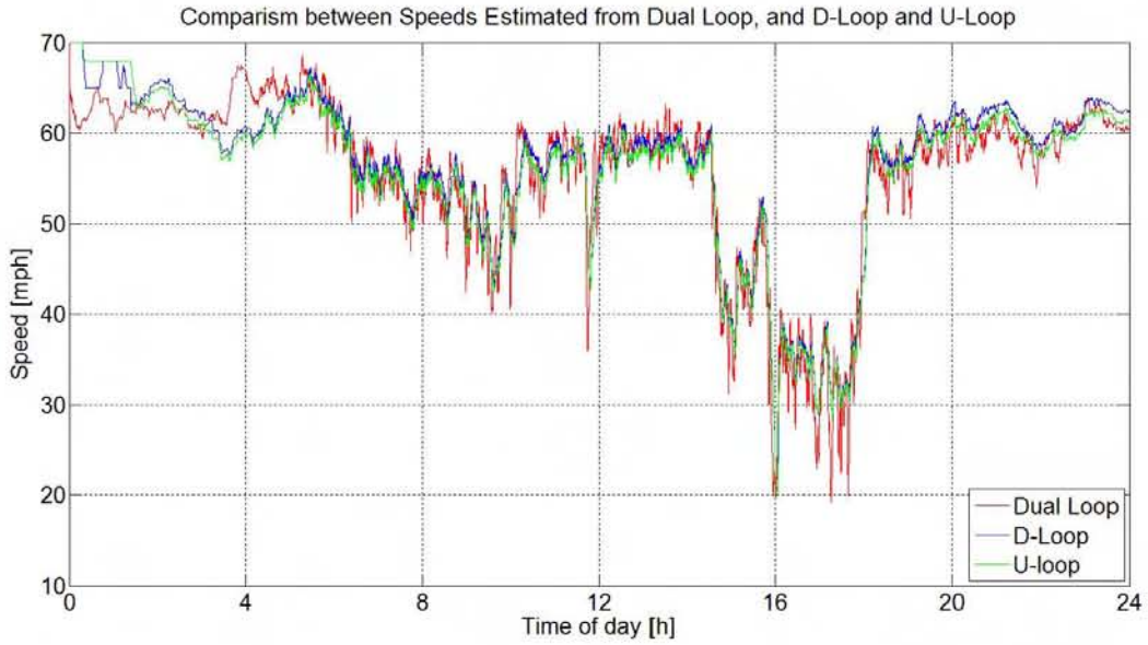
Figure B. 55 BHL WB, Station 6, Lane 5, Speed estimation comparison ***** *****
