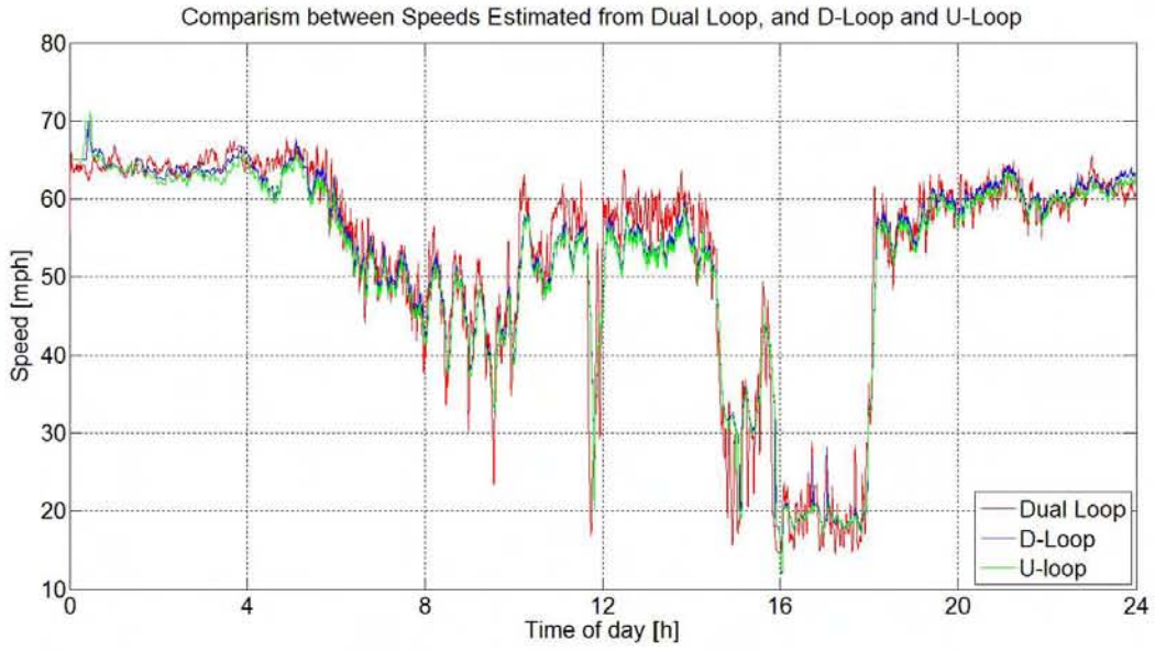
Figure B. 63 BHL WB, Station 7, Lane 3, Speed estimation comparison
