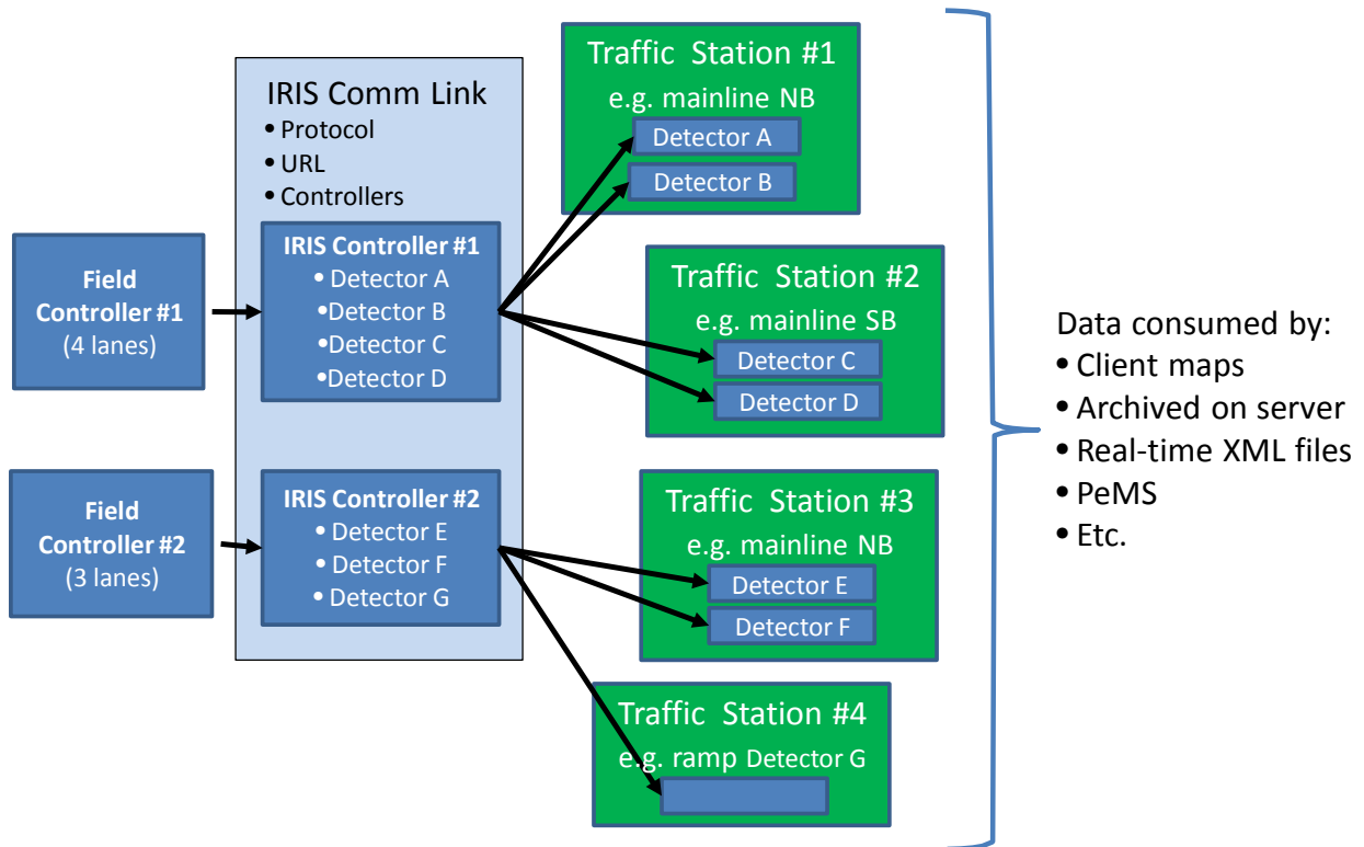
Figure 3.9: VDS configuration
