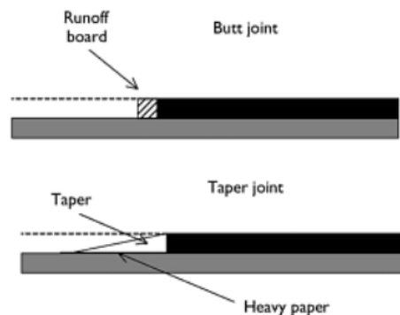
Figure 6.11 Transverse joints.
