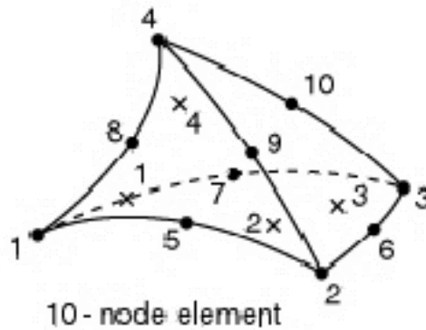
Figure 2-4 - Numbering of integration points for output
