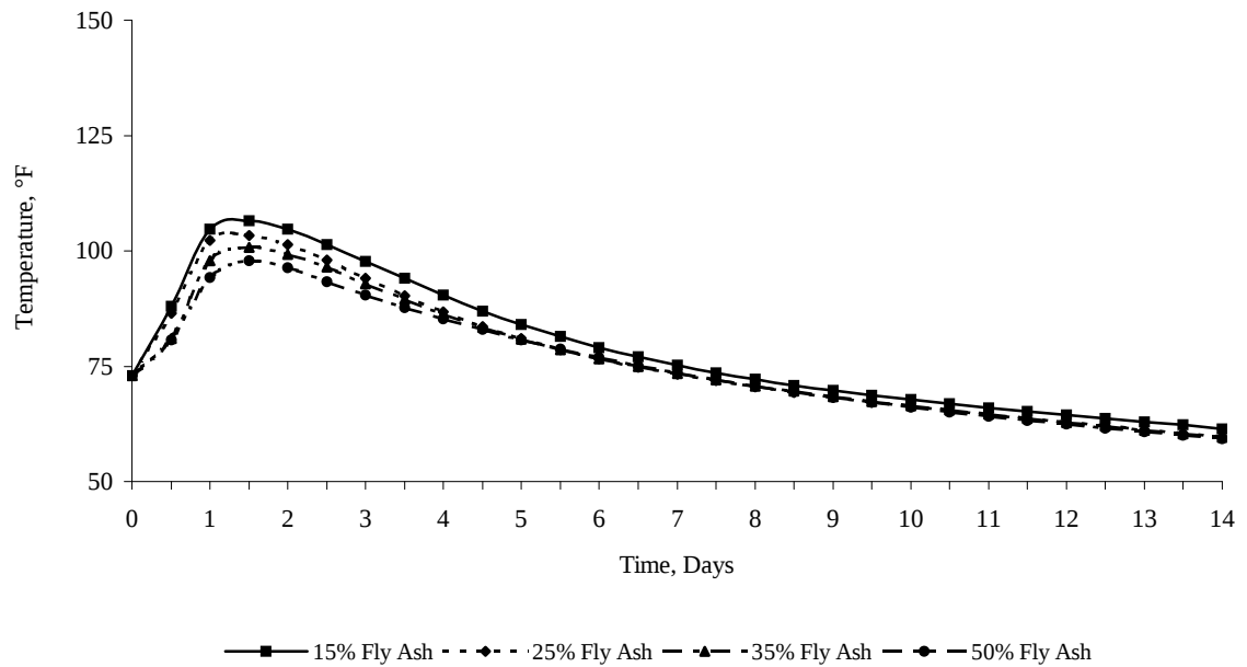
Figure 3-36 - Temperature versus Time for 6ft Pile – ABAQUS – Series 3 – (Total Cementitious Materials 506 lb/cy)
