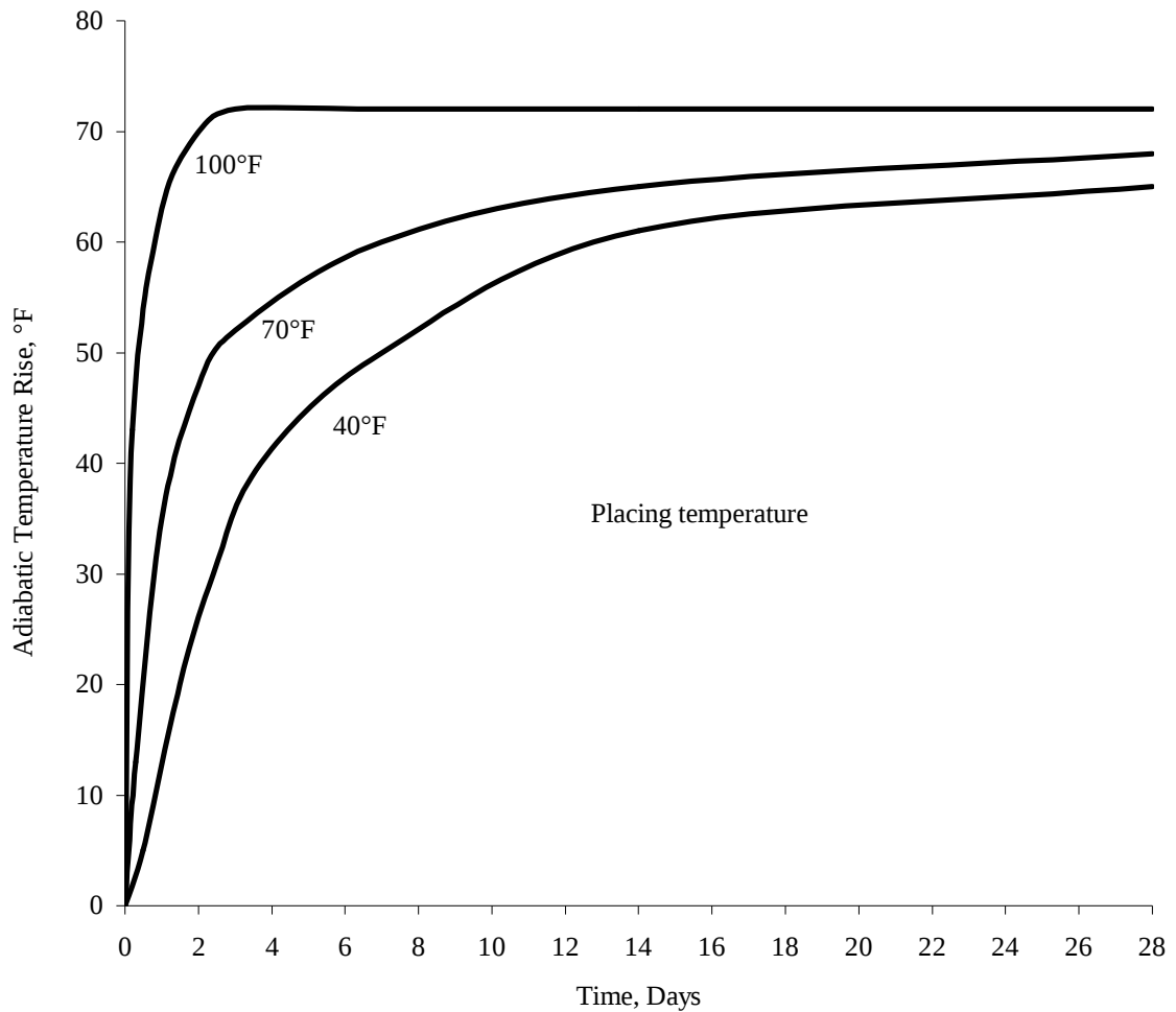
Figure 2-1 - Effect of placing temperatures of mass concrete (Type I cement 376 lb/yd 3 )
