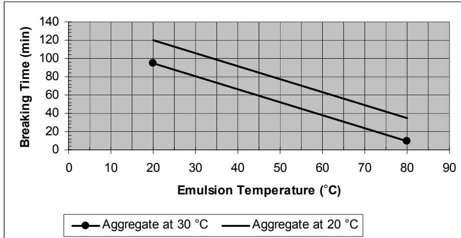
Figure 14: Effect of Temperature on Break Rate
