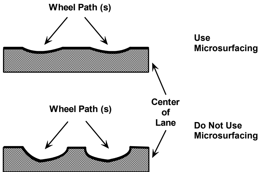
Figure 17: Suitable and Unsuitable Surfaces to Use Microsurfacing as a Rut Filler (7)
