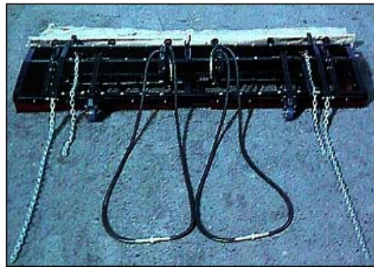
Figure 8: Slurry Seal Box with Augers (11)
