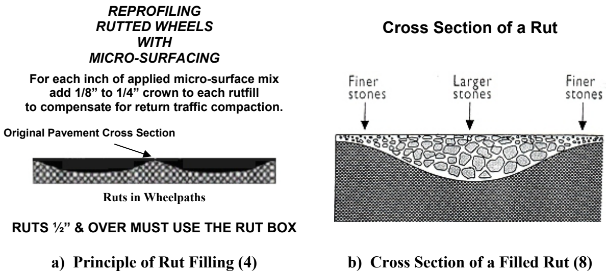
Figure 16: Rut Filling Principle and Sectional Diagram
