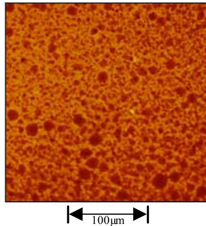
Figure 2: Micrograph of a Latex/Asphalt Cured Film (4)
