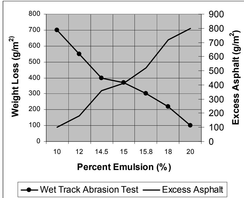
Figure 6: Determining Optimum Binder Content (8)
