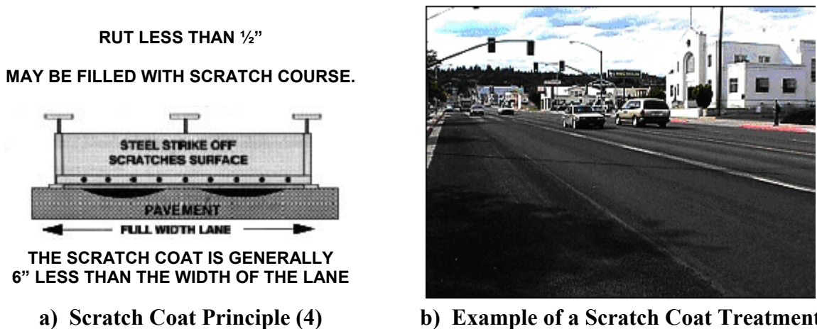
Figure 15: Scratch Coat Principles and Treatment
