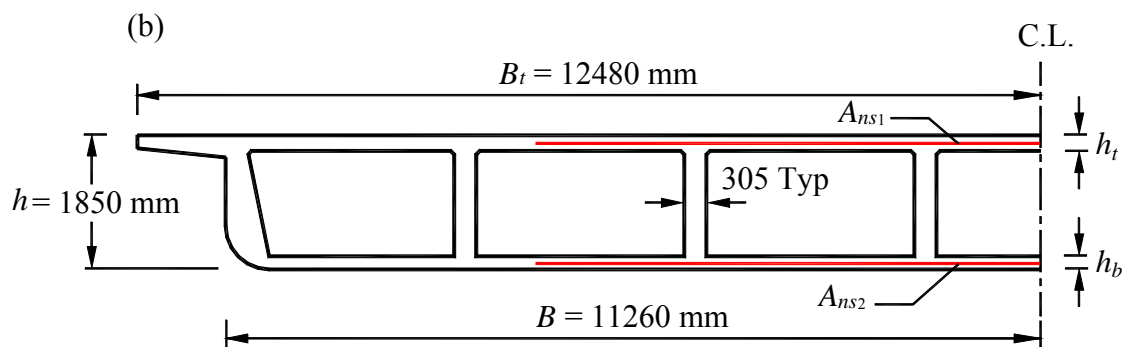
Fig. 6.1 Lake Hodges Bridge: (a) Half elevation; and (b) Half cross section.
