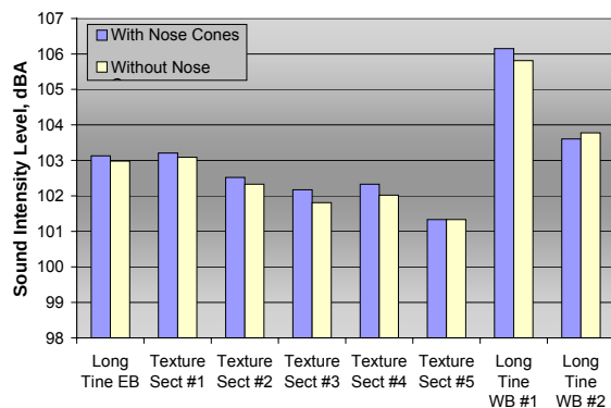
Figure 12: Comparison of overall SI levels with and without nose cones for a windscreen protected probe measured on PCC pavements on the Mojave Bypass
