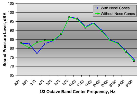
Figure 13: Comparison of 1/3 octave band SI levels with and without nose cones for a windscreen protected probe measured on PCC pavements on the Mojave Bypass
