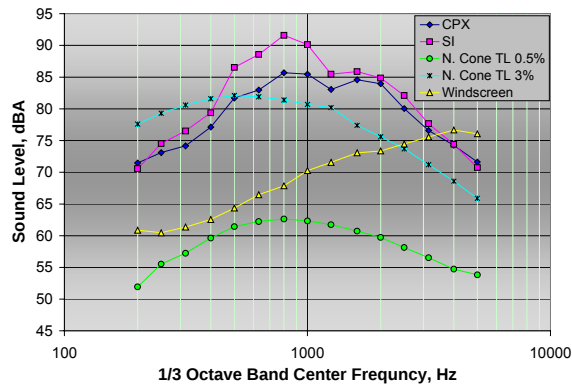
Figure 10: Increase in flow induced noise (SPL) with increase in turbulence level from 0.5% to 3% for a nose cone compared to windscreen performance and tire noise
