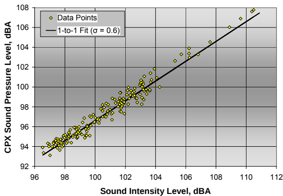
Figure 20: SI vs. CPX tire/pavement noise levels measured simultaneously on the ADOT CPX trailer using a two probe SI fixture
