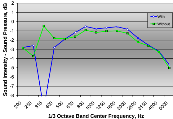
Figure 14: Comparison of 1/3 octave band differences between SI and SPL levels with and without nose cones for a windscreen protected probe measured on PCC pavements on the Mojave Bypass
