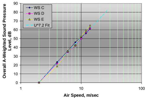
Figure 6b: Microphone windscreen performance for grazing incident flow spanning range of production variation for commercially available windscreens
