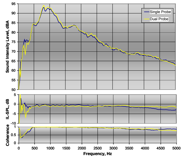
Figure 34: Comparison single and dual probe SI averages of multiple runs on grind #2 PCC for the leading edge of the tire contact patch
