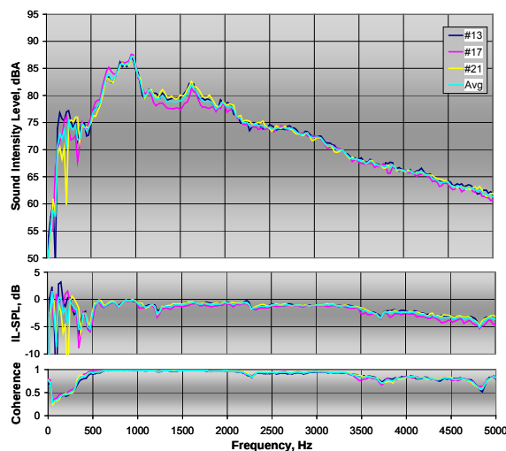
Figure 31: SI for multiple runs on ARFC for the trailing edge of the tire contact patch using the single probe fixture
