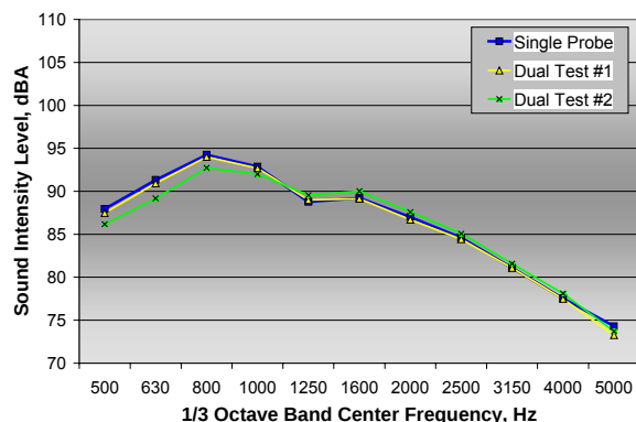
Figure 24: Comparison of 1/3 octave band SI levels measured with single and dual probe fixtures on ARFC
