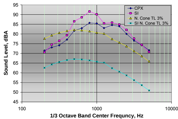
Figure 11: Comparison of the flow induced background noise for SPL and IL using nose cones with a 3% turbulence level relative CPX & SI tire/pavement noise
