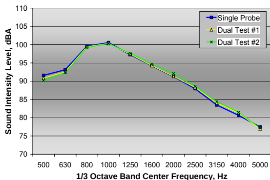
Figure 27: Comparison of 1/3 octave band SI levels measured with single and dual probe fixtures on Whisper grind PCC section #2
