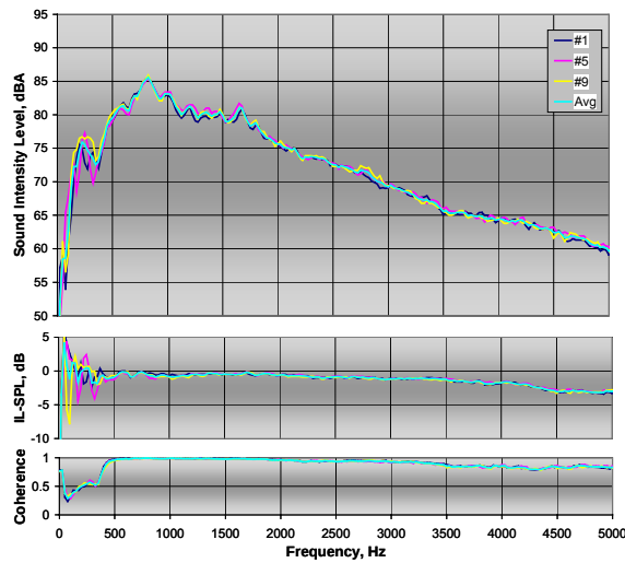
Figure 28: SI for multiple runs on ARFC for the leading edge of the tire contact patch using the single probe fixture
