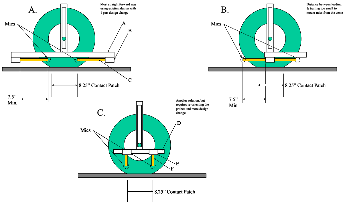
Figure 17: Alternative configurations conceptualized for a two probe tire/pavement noise SI measurement method
