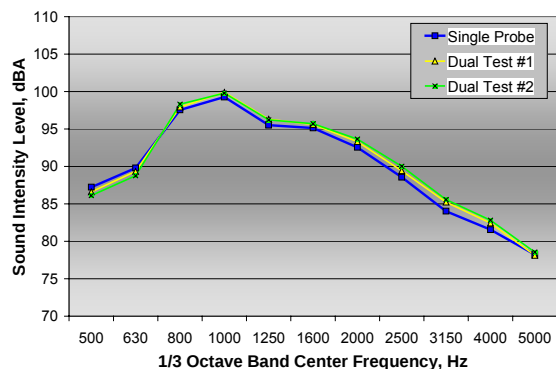
Figure 26: Comparison of 1/3 octave band SI levels measured with single and dual probe fixtures on Whisper grind PCC
