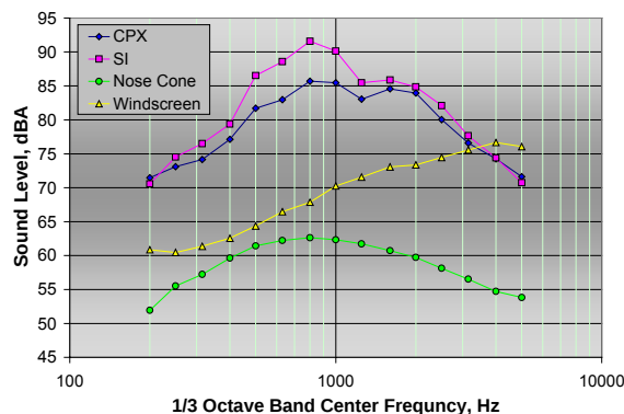
Figure 9: Comparison of flow induced noise (SPL) for a nose cone and a windscreen protected microphone relative to CPX & SI tire noise
