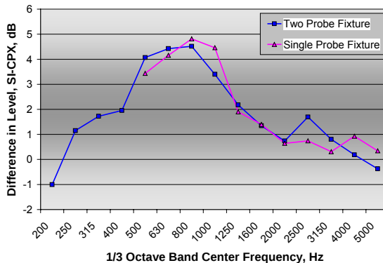
Figure 22: Comparison of averages of differences in 1/3 octave band levels between SI and CPX measurements made with the ADOT CPX trailer using single and dual probe fixtures
