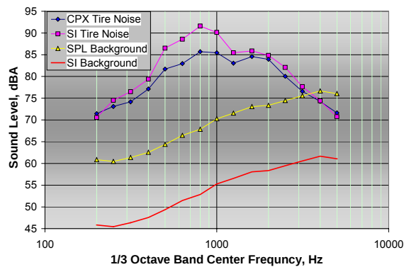
Figure 8: Comparison of flow induced background noise in SI and SPL measurements relative to tire noise and wind flow induced at 60 mph for windscreen protected microphones
