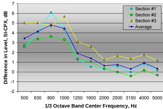
Figure 16: Difference in 1/3 octave band levels between SI and CPX measurements made with the ADOT CPX trailer on 3 AC pavements for the same test tire
