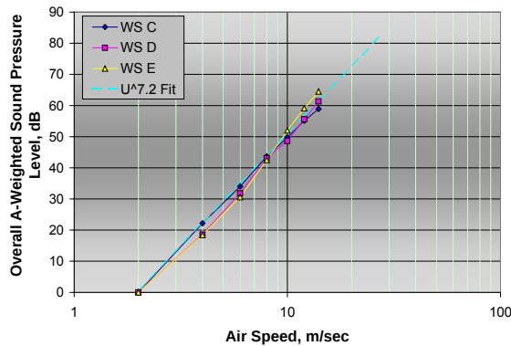
Figure 6a: Microphone windscreen performance for normally incident flow spanning range of production variation for commercially available windscreens
