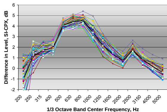
Figure 21: Difference in 1/3 octave band levels between SI and CPX measurements made simultaneously on the ADOT CPX trailer using the two probe fixture on different pavements
