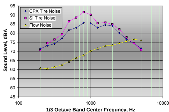
Figure 7: Wind flow induced noise (SPL) for microphone windscreen (#E) for grazing flow at 60 mph compared to CPX and SI tire noise for a quieter AZ ARFC pavement
