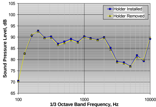
Figure 19: Comparison of CPX sound pressure levels measured with and without the two probe SI fixture installed on the CPX trailer in the lab for a loudspeaker noise source
