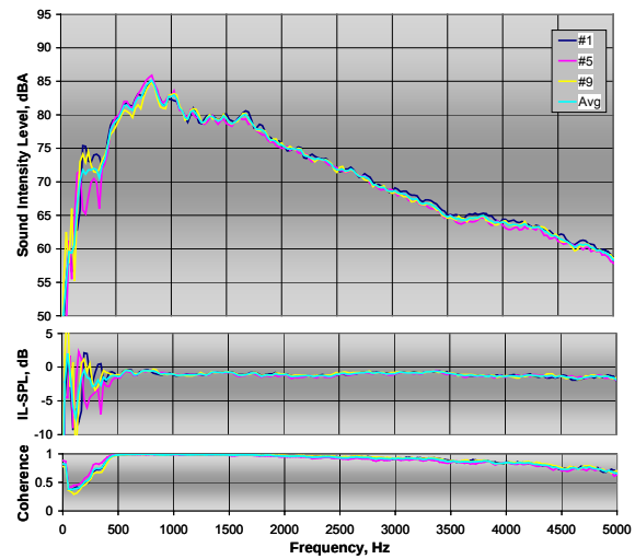
Figure 29: SI for multiple runs on ARFC for the leading edge of the tire contact patch using the dual probe fixture
