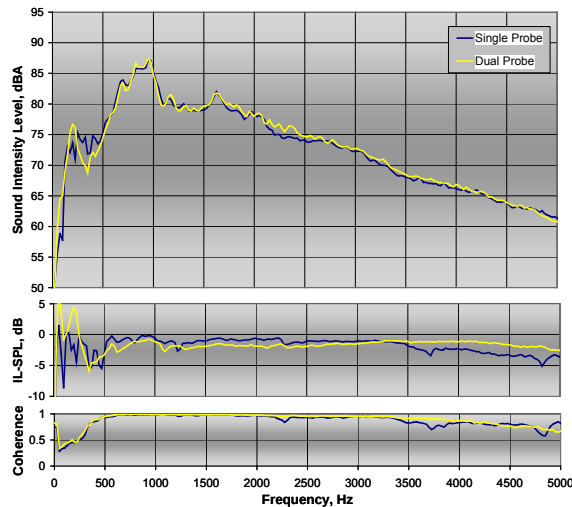
Figure 33: Comparison single and dual probe SI averages of multiple runs on ARFC for the Trailing edge of the tire contact patch
