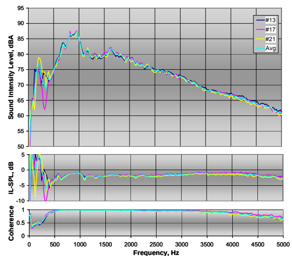
Figure 32: SI for multiple runs on ARFC for the trailing edge of the tire contact patch using the dual probe fixture
