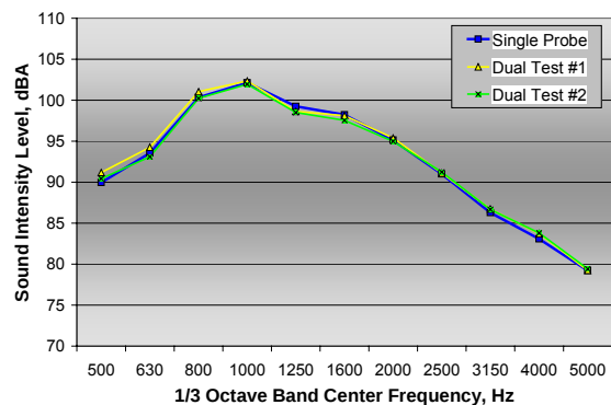
Figure 25: Comparison of 1/3 octave band SI levels measured with single and dual probe fixtures on longitudinally tined PCC
