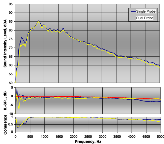
Figure 30: Comparison single and dual probe SI averages of multiple runs on ARFC for the leading edge of the tire contact patch
