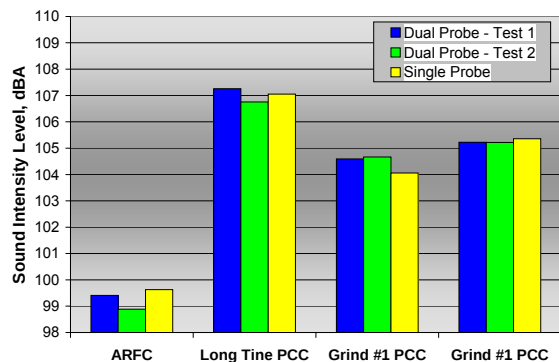
Figure 23: Comparison of overall A-weighted SI levels measured with single and dual probe fixtures on 4 pavements
