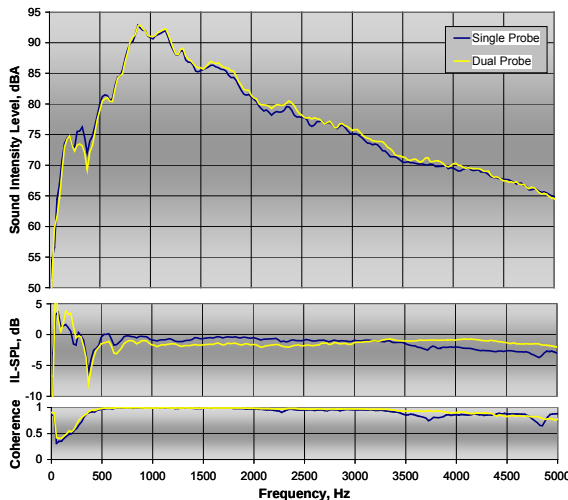
Figure 35: Comparison single and dual probe SI averages of multiple runs on grind #2 PCC for the trailing edge of the tire contact patch
