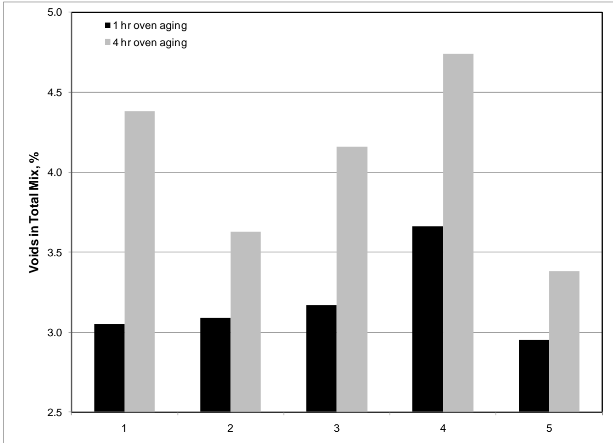
Figure 3: Influence of Oven Aging Time on Air Void Content
