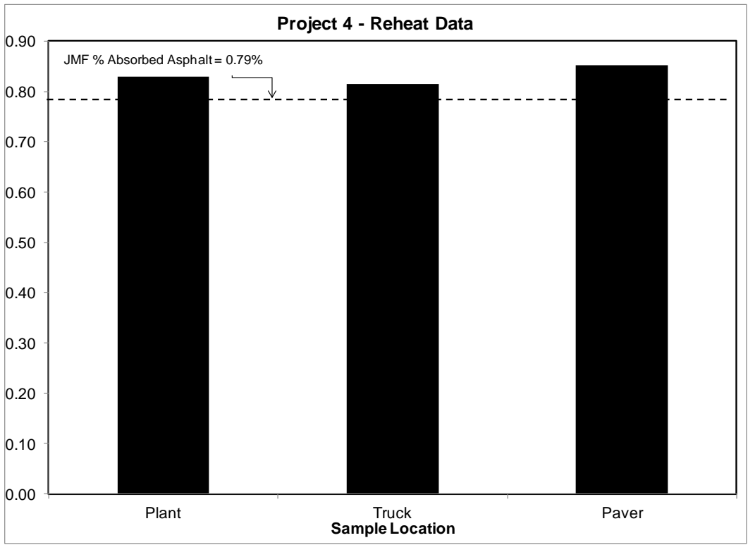
Figure 23: Average Percent Absorbed Asphalt at Each Sample Location - Project 4
