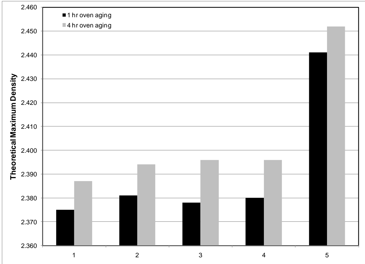
Figure 1: Effect of Aging Time on Theoretical Maximum Density
