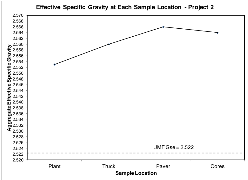
Figure 17: Effective Specific Gravity at Each Sample Location - Project 2
