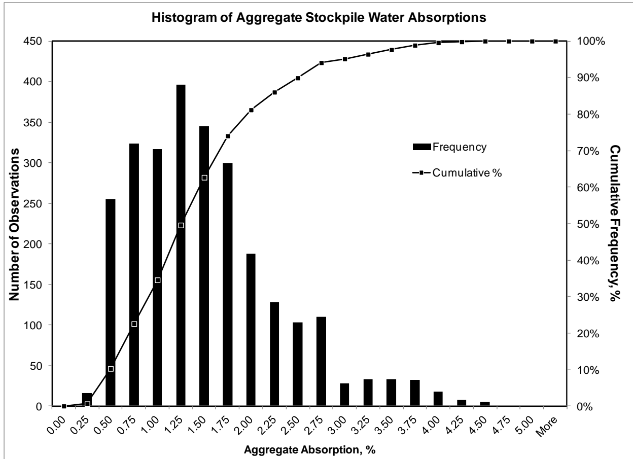
Figure 6: Histogram of Water Absorptions Encountered
