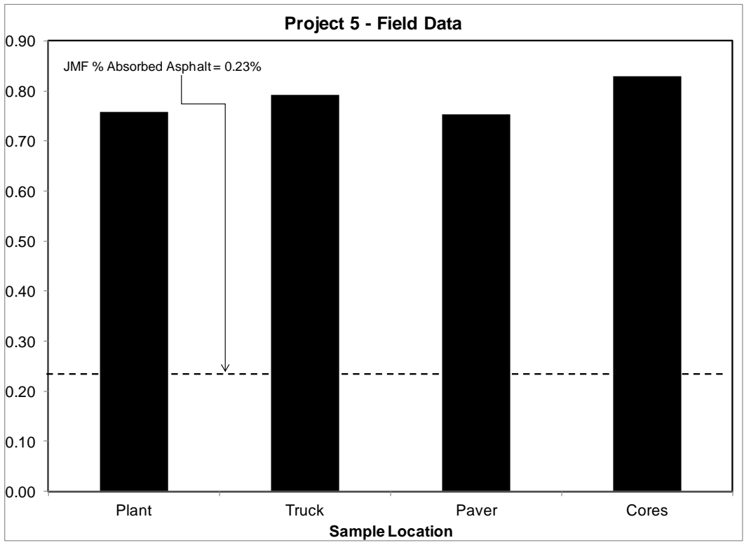
Figure 14: Average Percent Absorbed Asphalt at Each Sample Location - Project 5
