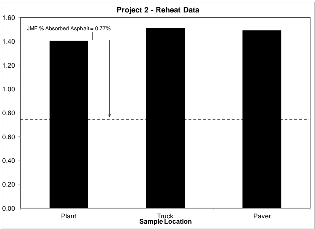
Figure 21: Average Percent Absorbed Asphalt at Each Sample Location - Project 2
