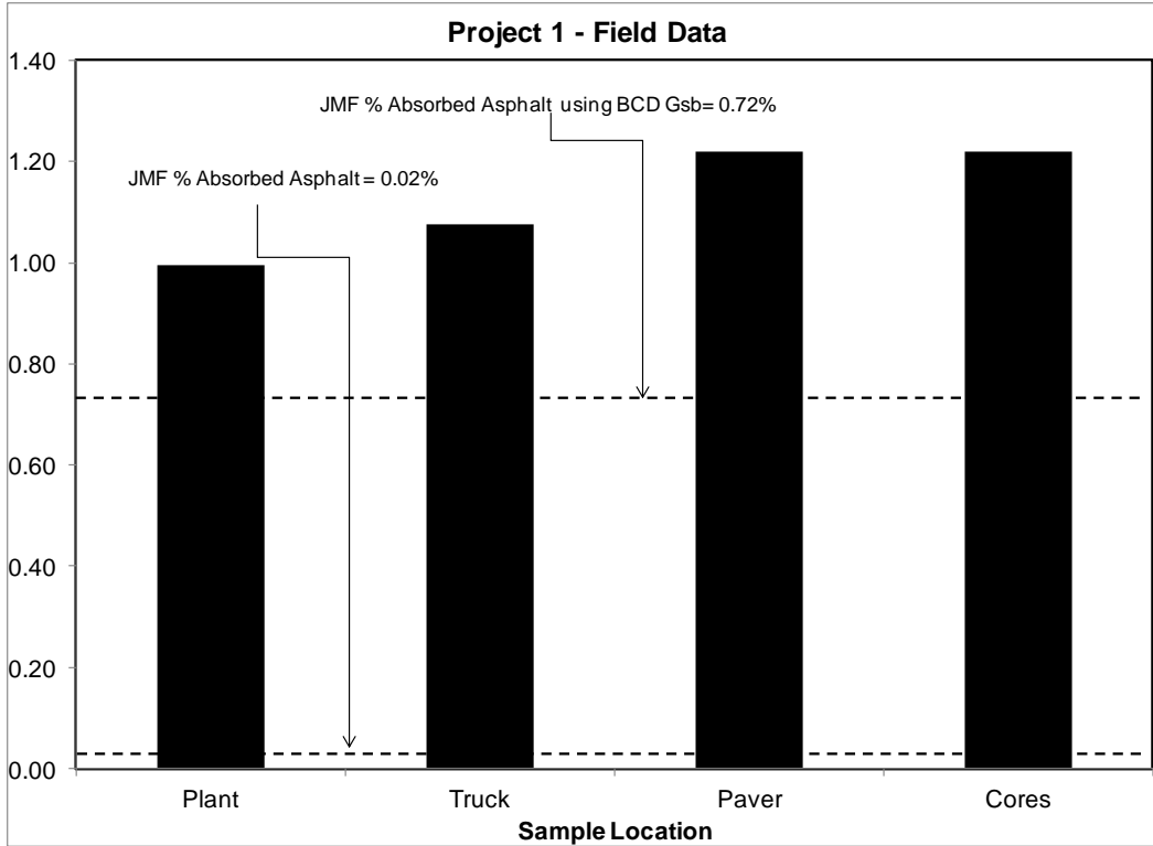
Figure 10: Average Percent Absorbed Asphalt at Each Sample Location – Project 1
