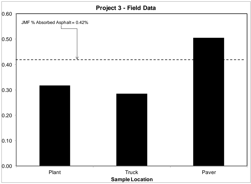
Figure 12: Average Percent Absorbed Asphalt at Each Sample Location - Project 3
