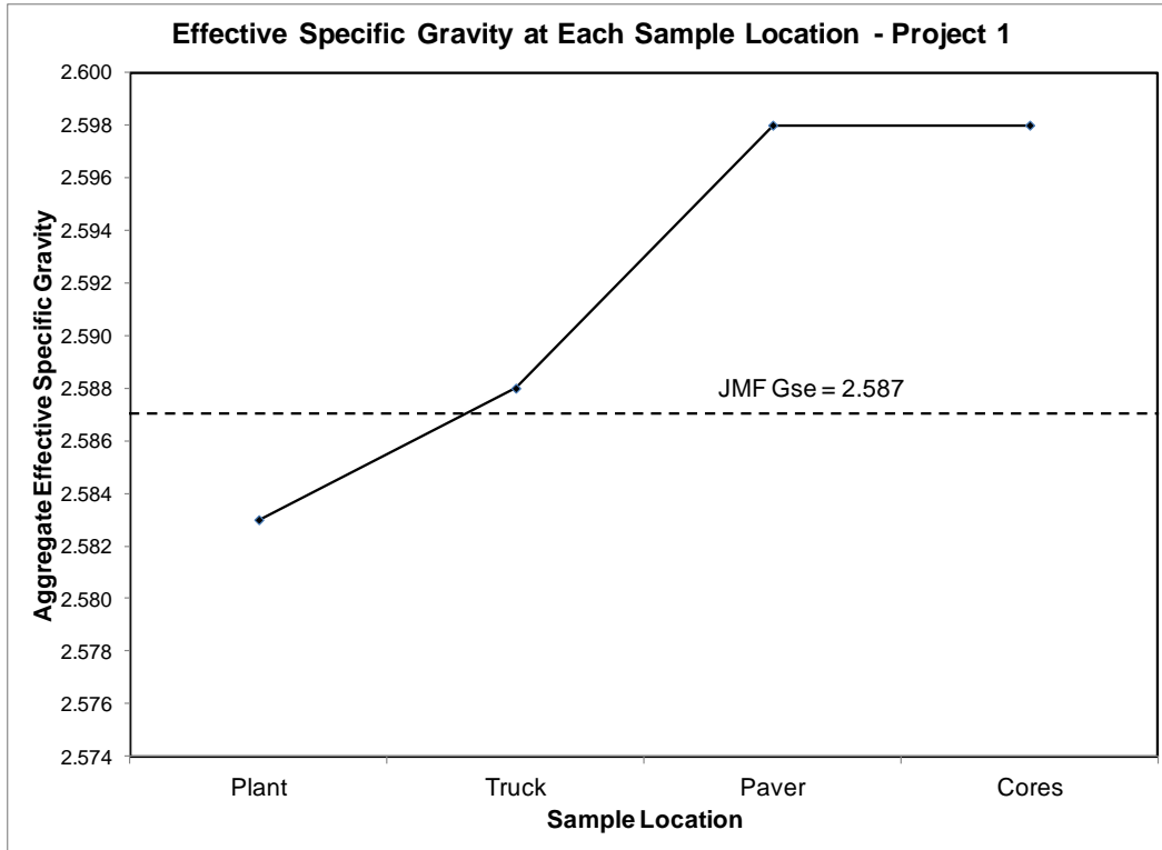
Figure 16: Effective Specific Gravity at Each Sample Location - Project 1
