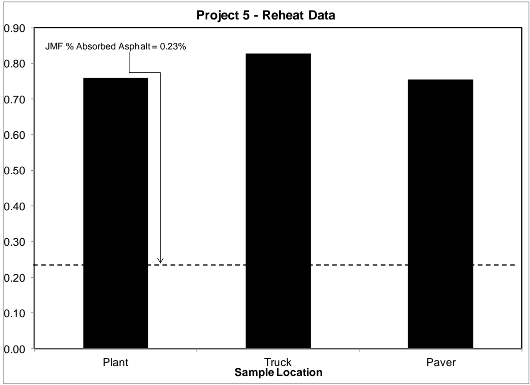
Figure 24: Average Percent Absorbed Asphalt at Each Sample Location - Project 5
