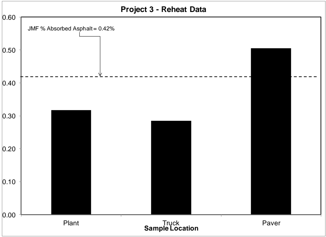
Figure 22: Average Percent Absorbed Asphalt at Each Sample Location - Project 3
