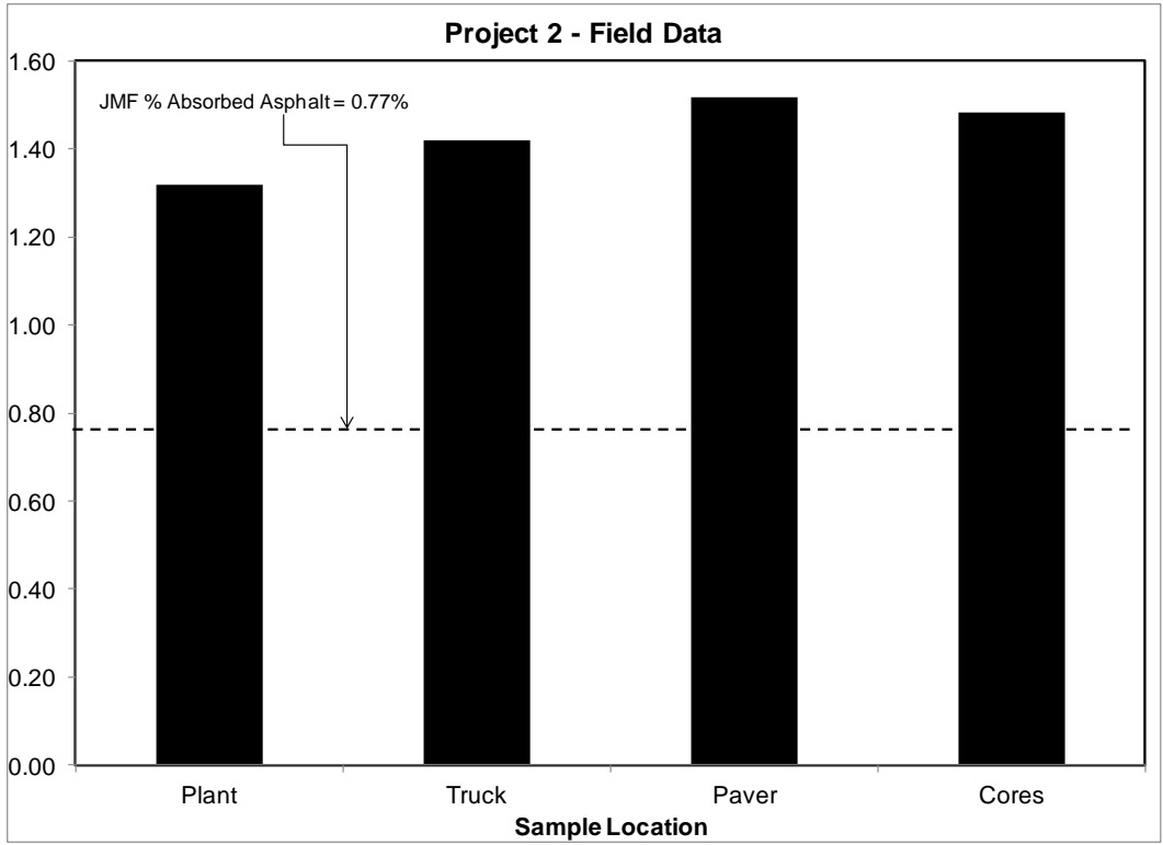
Figure 11: Average Percent Absorbed Asphalt at Each Sample Location - Project 2
