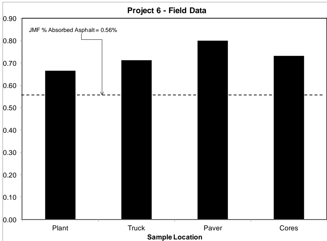
Figure 15: Average Percent Absorbed Asphalt at Each Sample Location - Project 6
