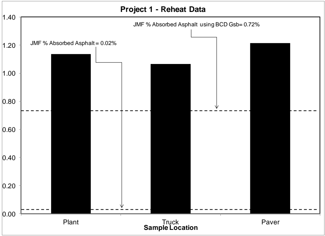
Figure 20: Average Percent Absorbed Asphalt at Each Sample Location - Project 1
