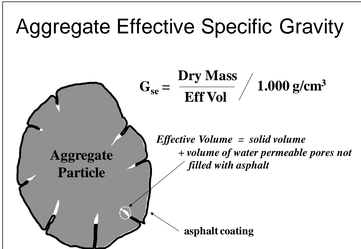
Figure 9: Definition of Aggregate Effective Specific Gravity
