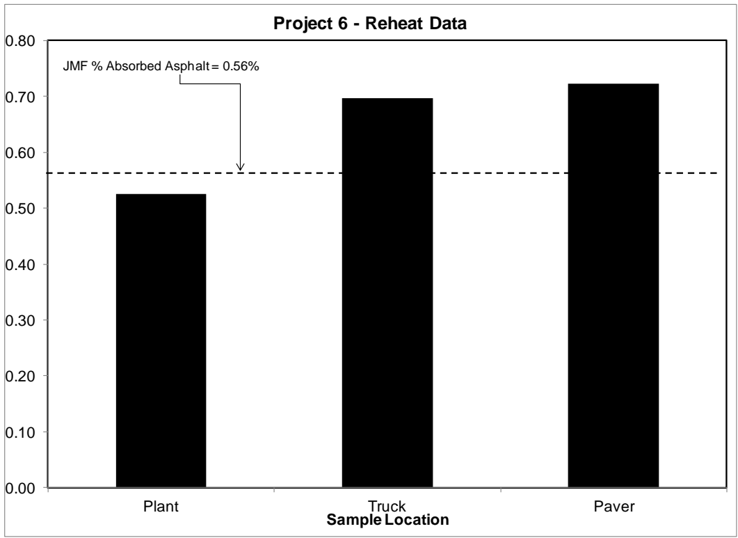
Figure 25: Average Percent Absorbed Asphalt at Each Sample Location - Project 6
