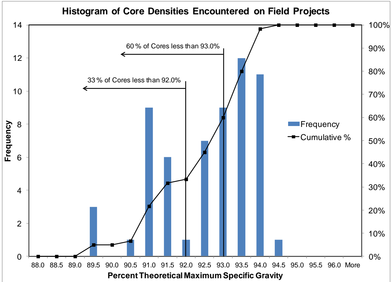
Figure 19: Histogram Showing Range of In-Place Densities Encountered
