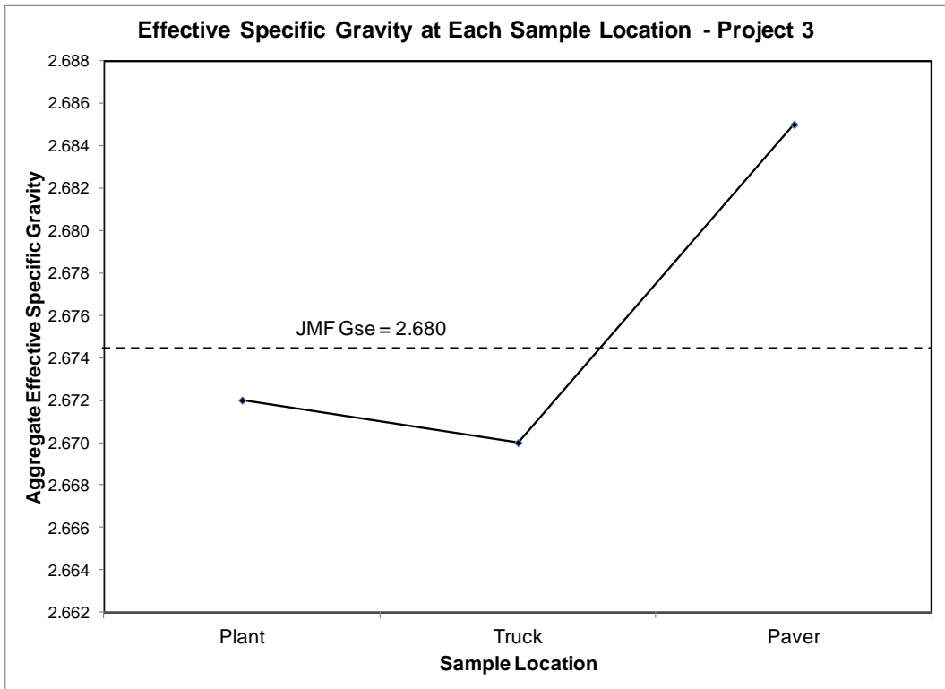
Figure 18: Effective Specific Gravity at Each Sample Location - Project 3
