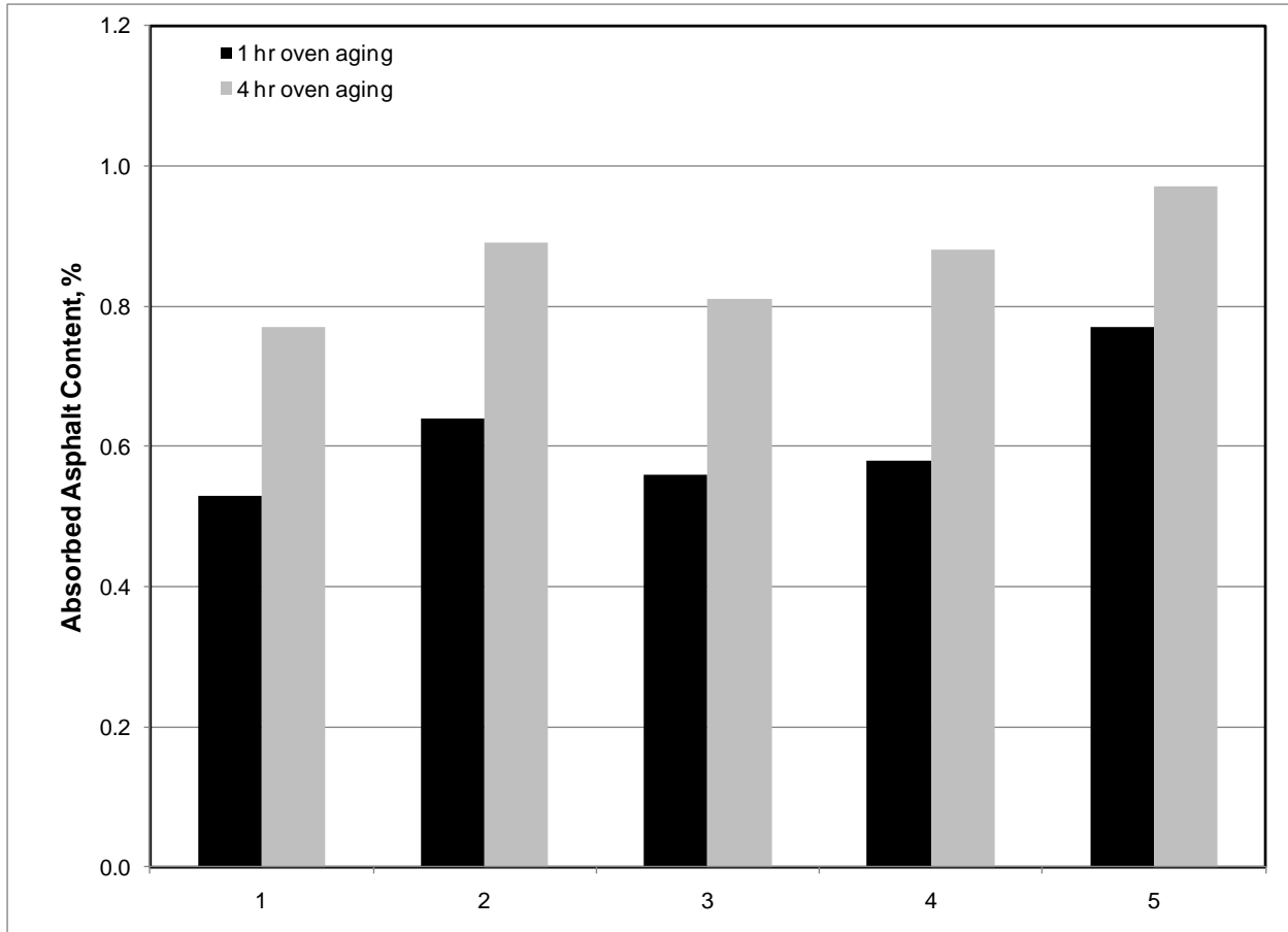
Figure 2: Influence of Aging Time on Absorbed Asphalt Content
