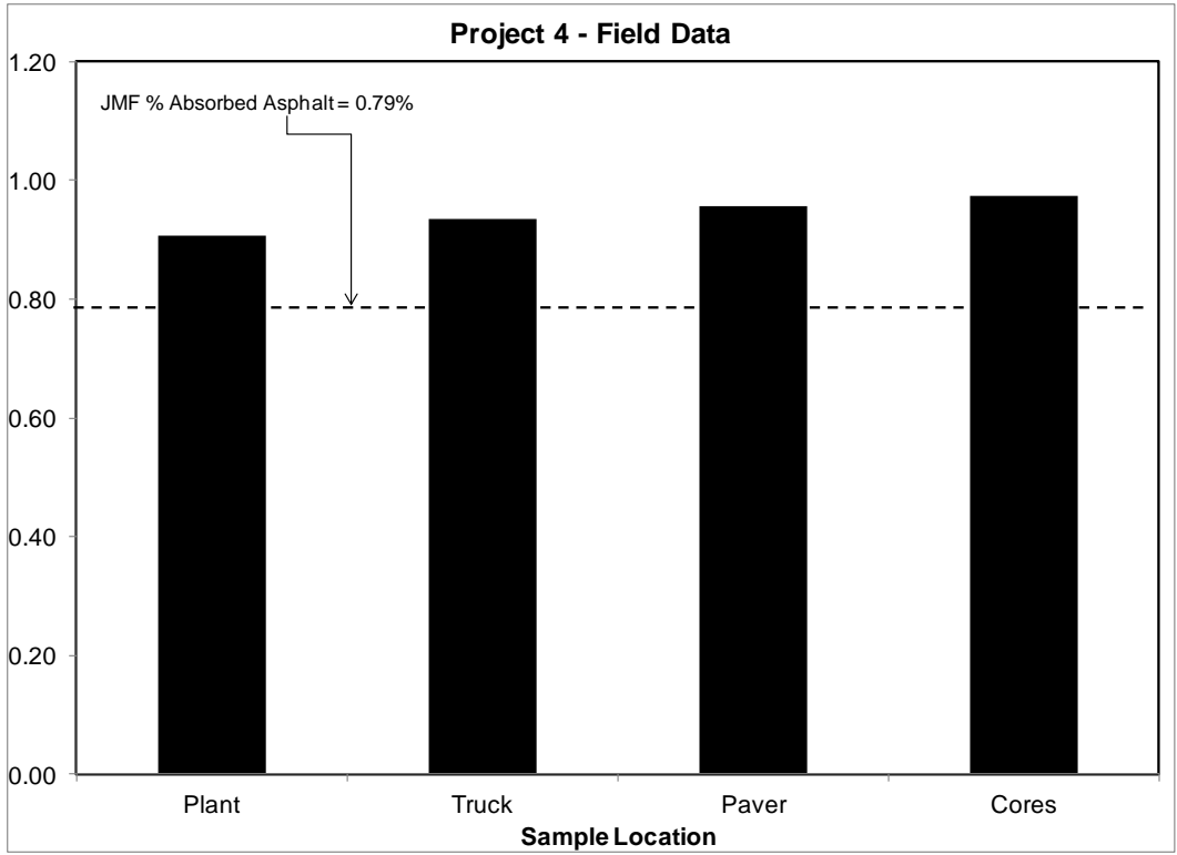
Figure 13: Average Percent Absorbed Asphalt at Each Sample Location - Project 4
