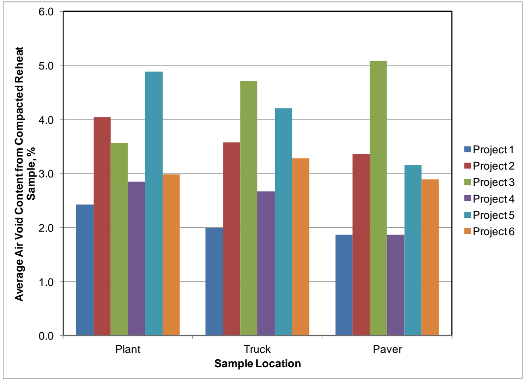
Figure 26: Average Air Void Content by Sample Location - Reheat Samples
