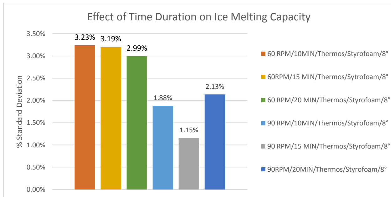
Figure 17: Time Duration - Standard Deviation
