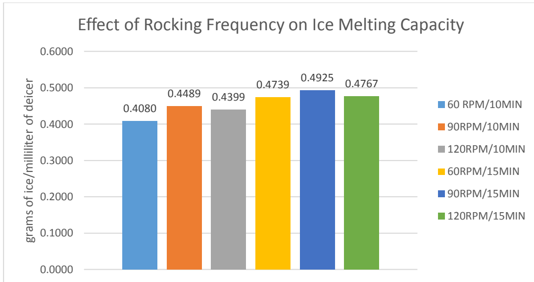
Figure 12: Rocking Frequency - Ice Melting Capacity
