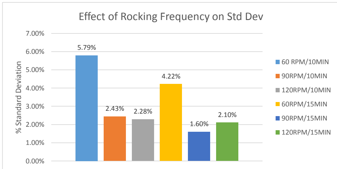
Figure 13: Rocking Frequency - Standard Deviation
