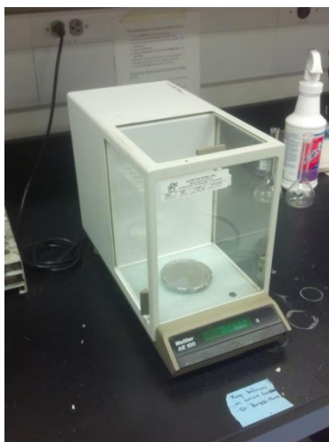
Figure 6: Digital Mass Balance (in confined space)
