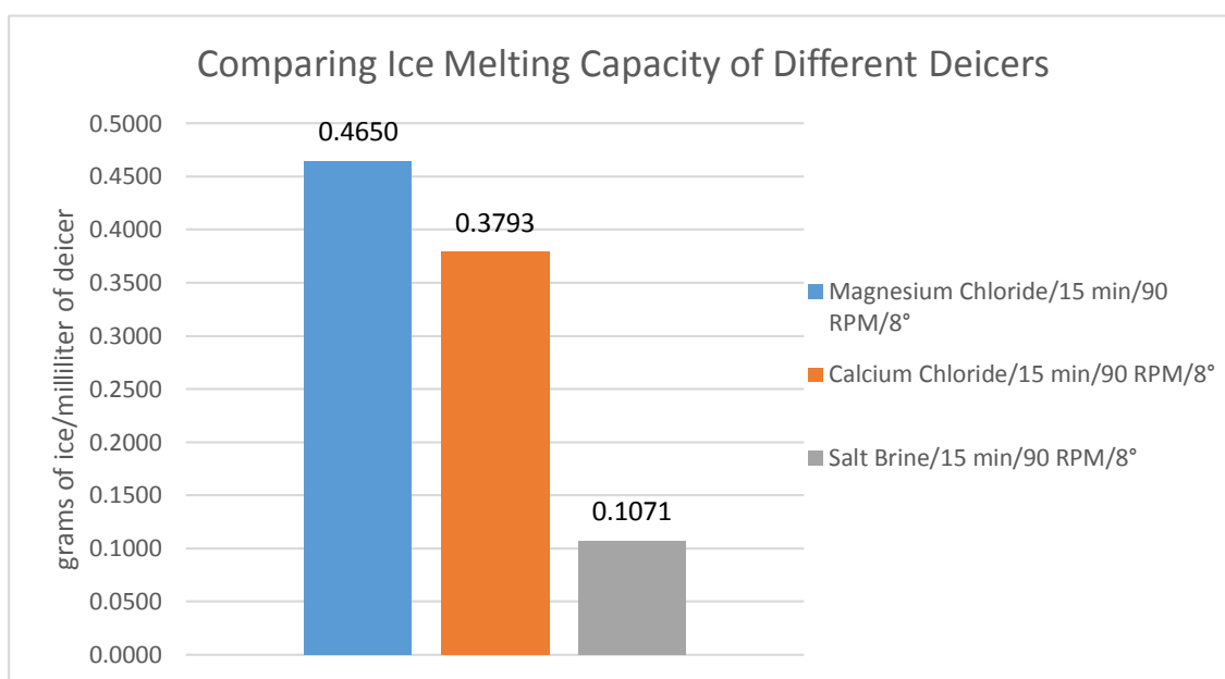
Figure 24: Different Deicer Chemicals - Ice Melting Capacity
