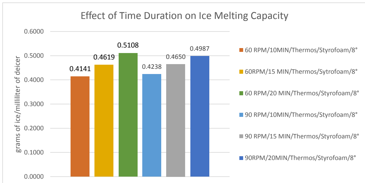
Figure 16: Time Duration - Ice Melting Capacity
