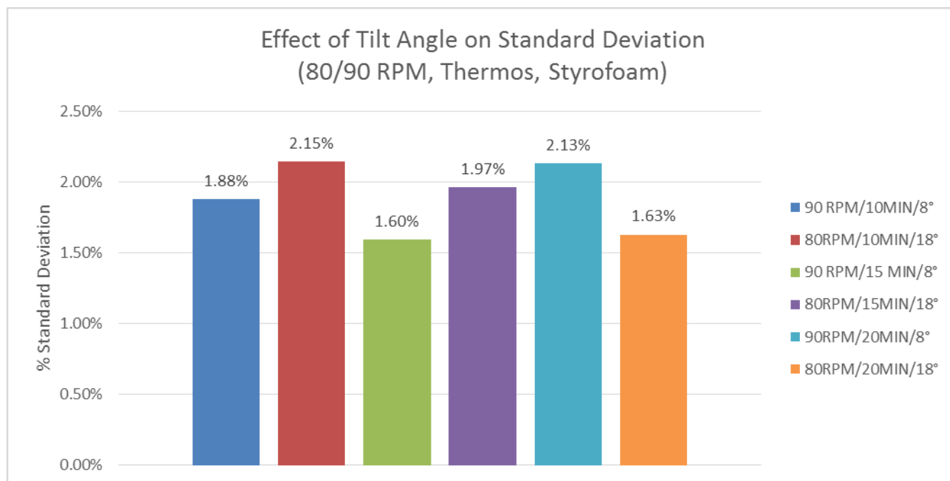
Figure 21: Tilt Angle at 90RPM - Standard Deviation
