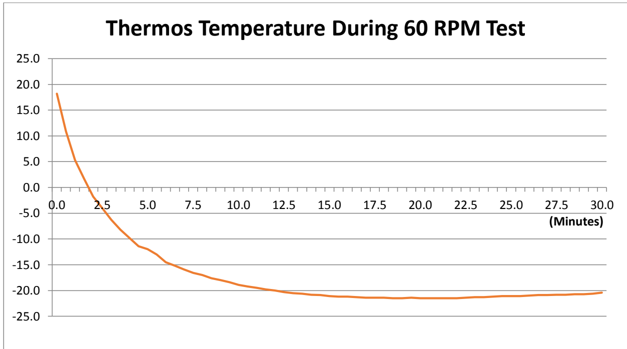
Figure 14: Thermos Temperature during a 60 RPM Test
