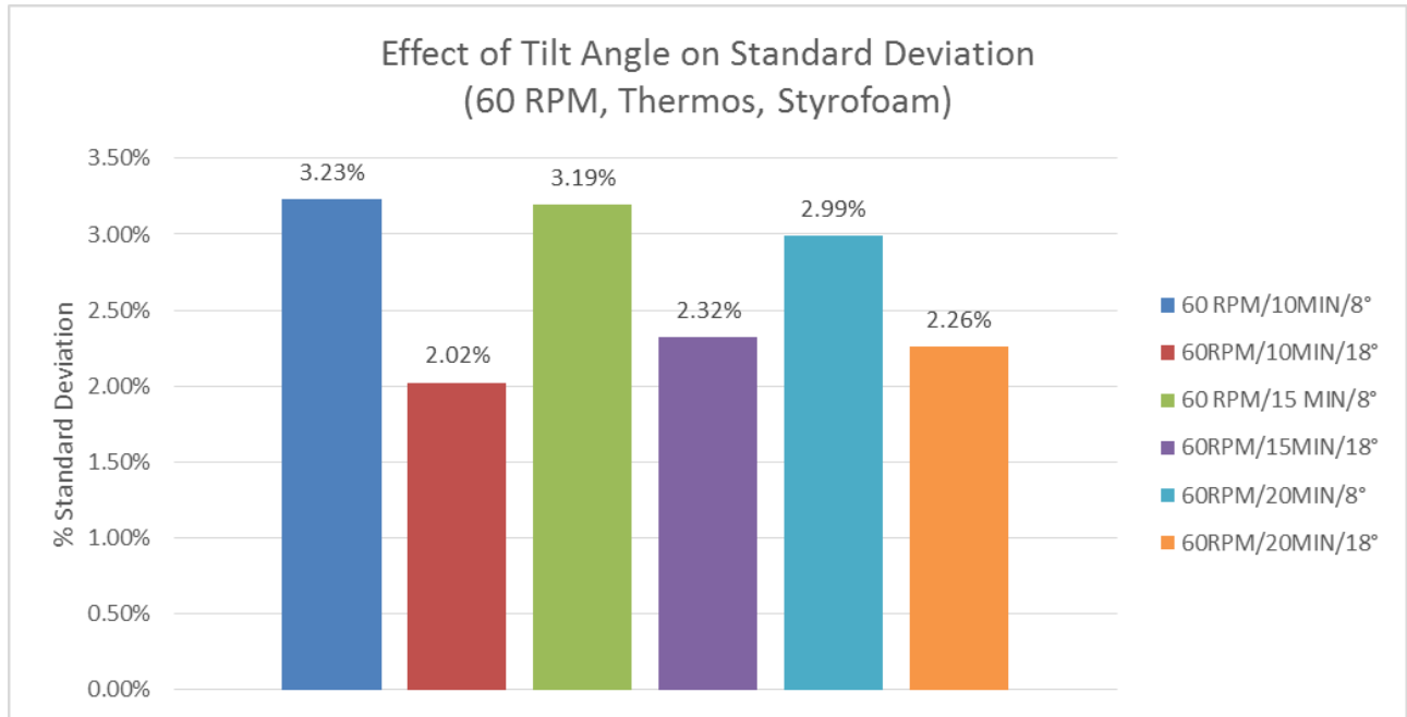
Figure 19: Tilt Angle at 60 RPM - Standard Deviation
