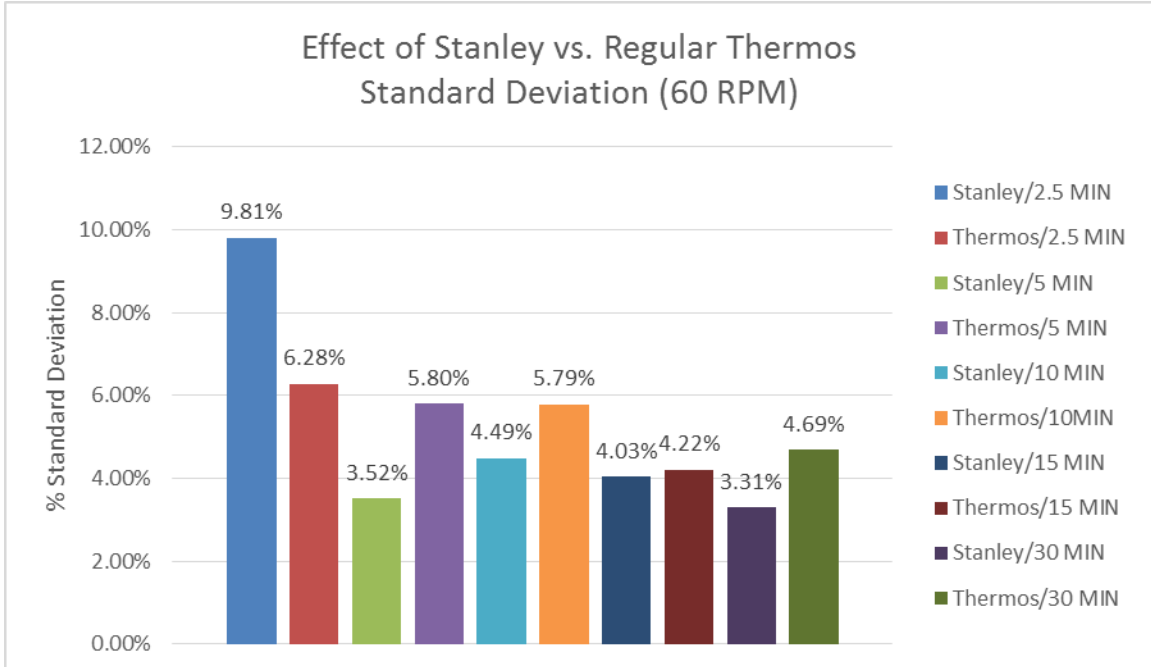
Figure 11: Stanley vs. Thermos - Standard Deviation
