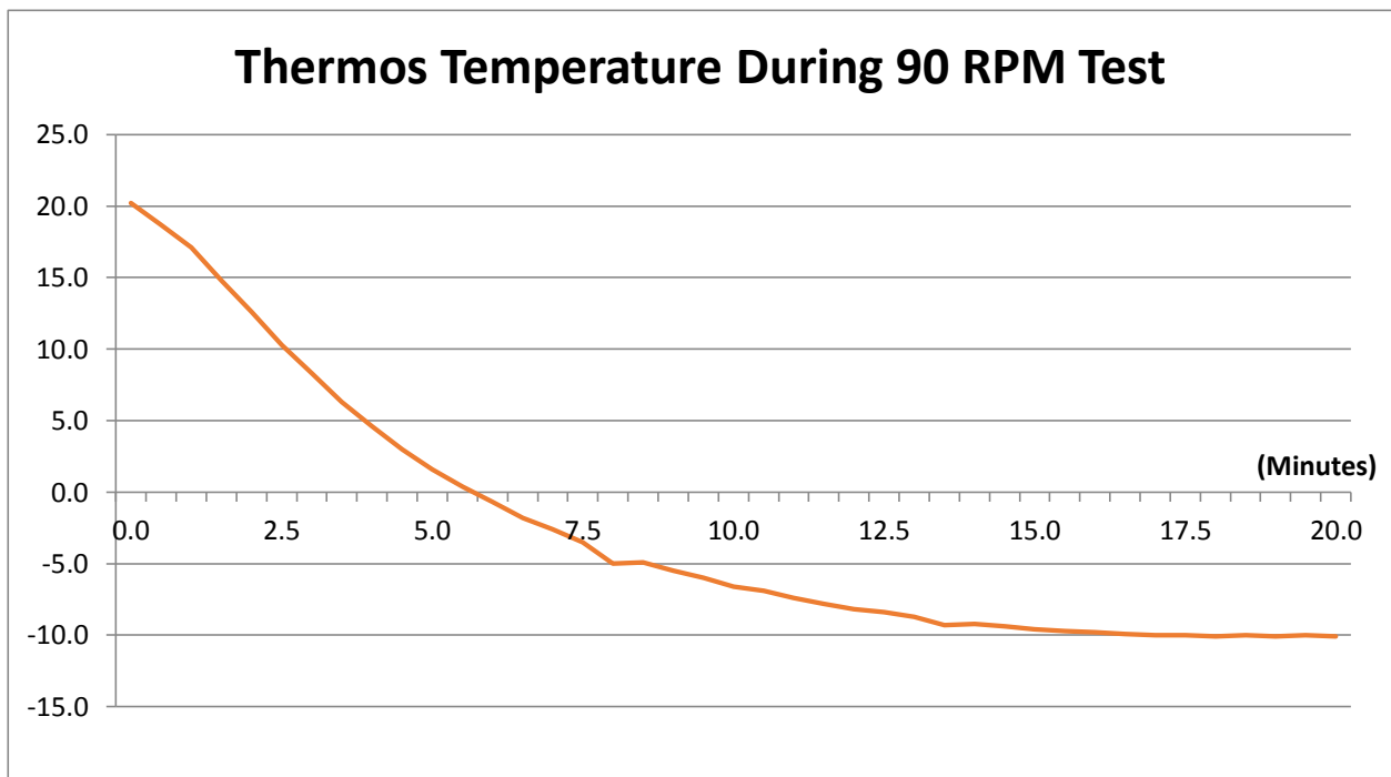
Figure 15: Thermos Temperature during a 90 RPM Test
