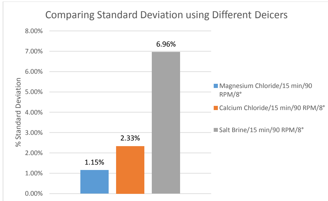
Figure 25: Different Deicer Chemicals - Standard Deviation
