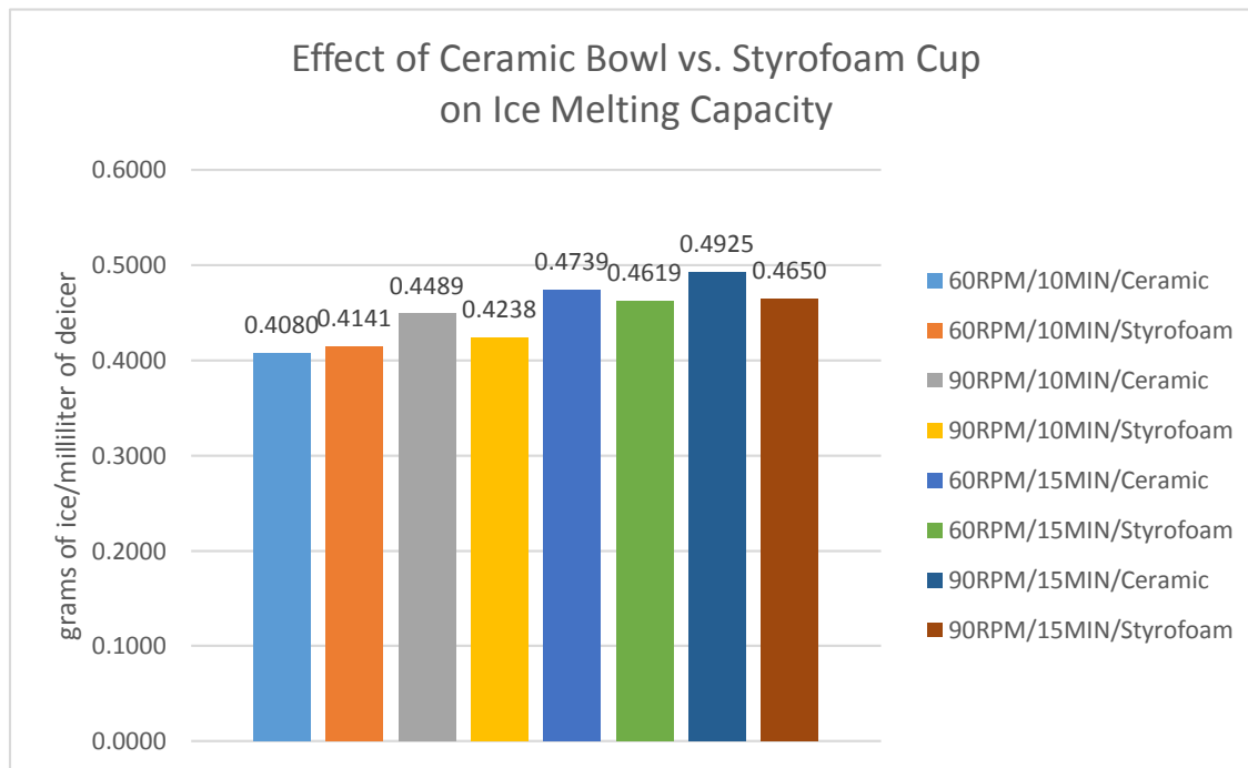
Figure 22: Ceramic Bowl vs. Styrofoam Cup - Ice Melting Capacity
