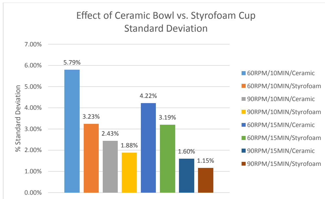
Figure 23: Ceramic Bowl vs. Styrofoam Cup - Standard Deviation
