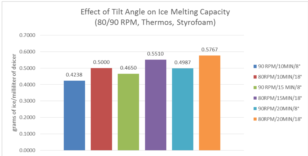
Figure 20: Tilt Angle at 90 RPM - Ice Melting Capacity
