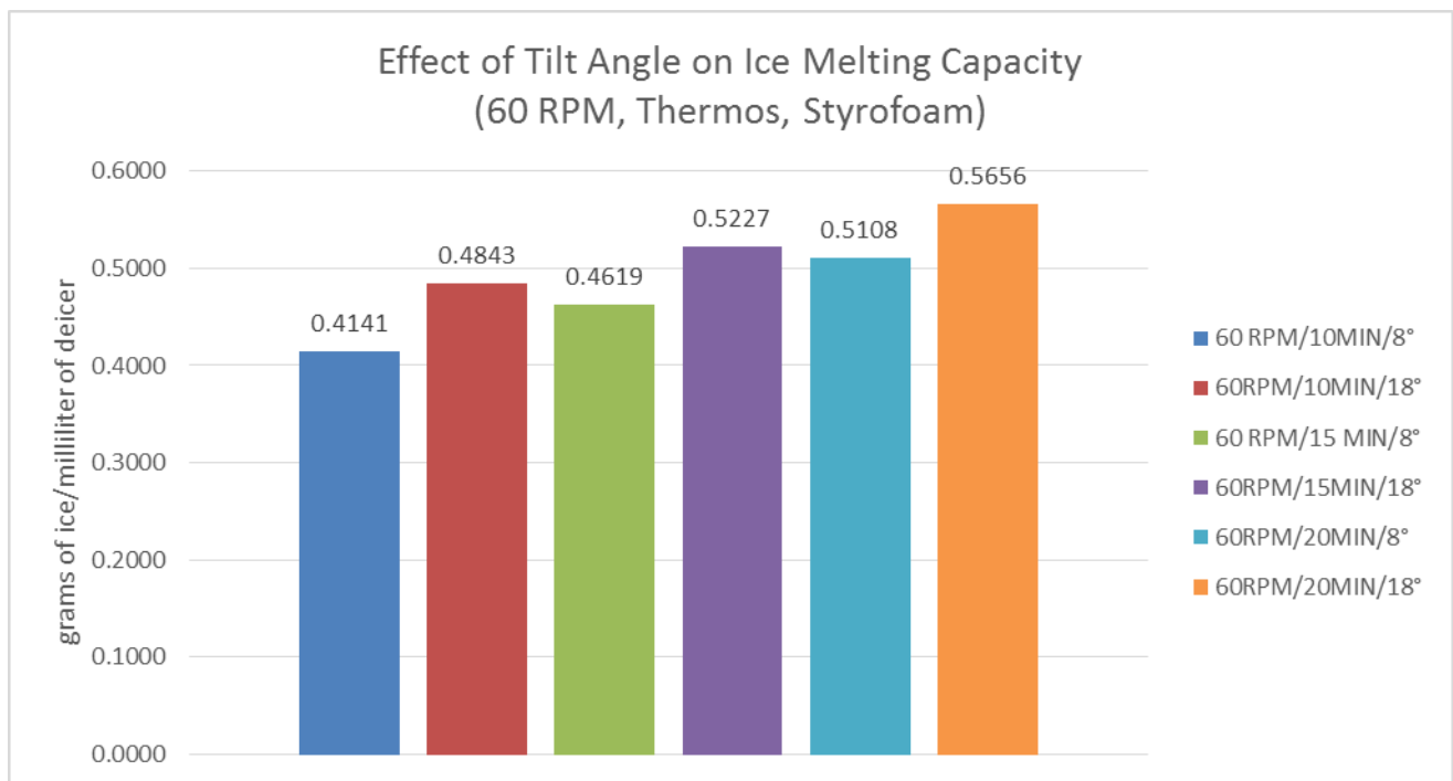
Figure 18: Tilt Angle at 60 RPM - Ice Melting Capacity
