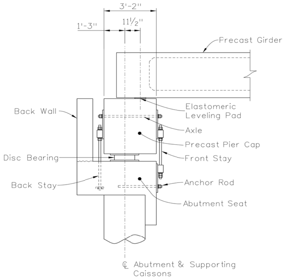
Figure 6 - Typical Abutment Section
