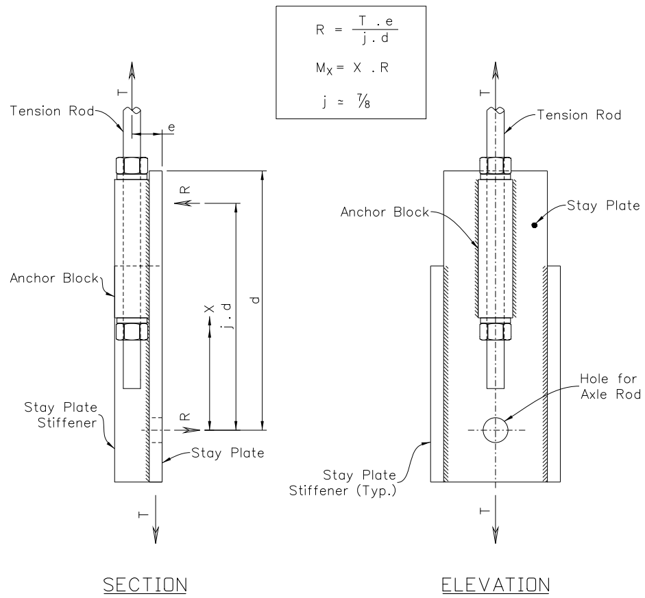
Figure 8 - Stay Plate Stiffeners
