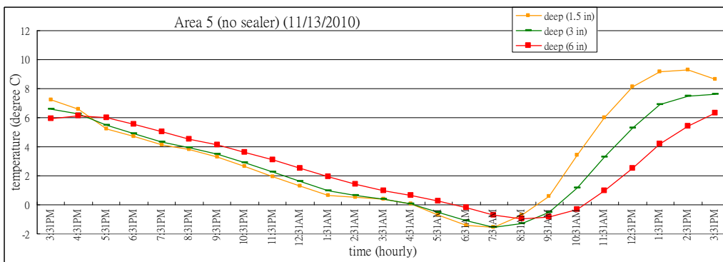
Fig 5.10 Comparison of temperature variations at different depths over 24 hrs. (no sealer)
