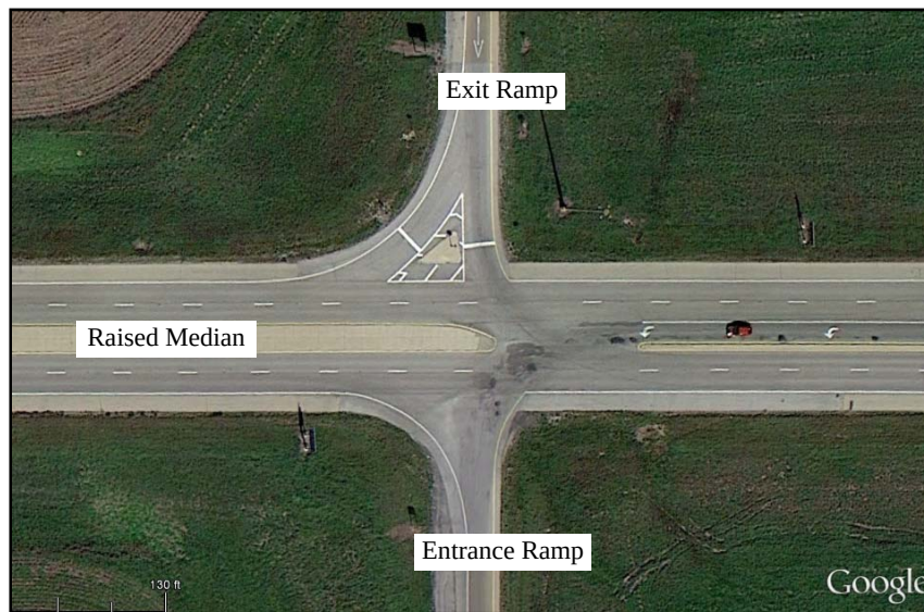
Figure 3-10. A non-traversable raised median at the ramp-crossroad intersection of a diamond interchange (Image: Google Earth).
