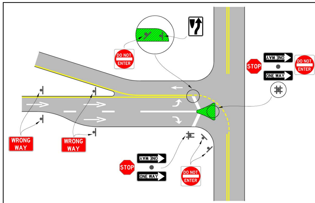
Figure 2-19. Example of signing and pavement markings at an exit ramp of parclo interchange (with island).
