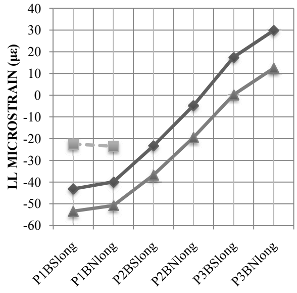
STRAIN TRANSDUCER b. 2008; Path 2
