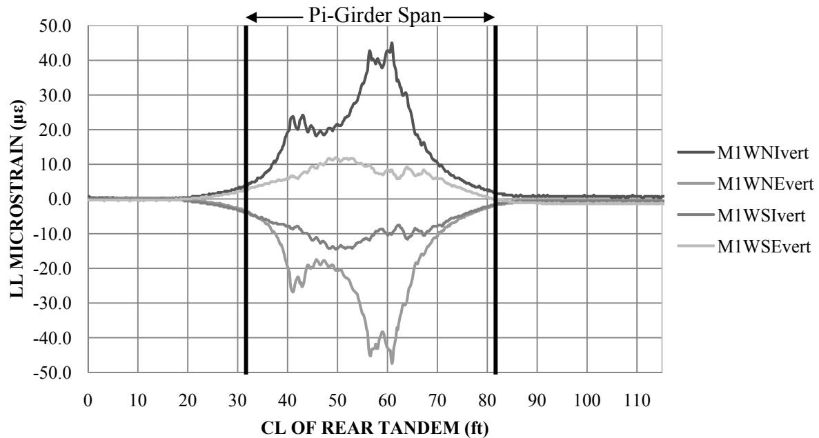
Figure 5.16-Representative Sample of LL Vertical Web Strain along Path 3
