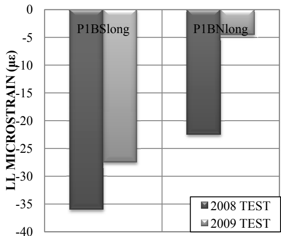
STRAIN TRANSDUCER a. 2008 & 2009; Path 1
