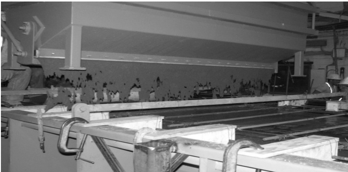
Figure 3.1 Placement of UHPC Material into Forms
