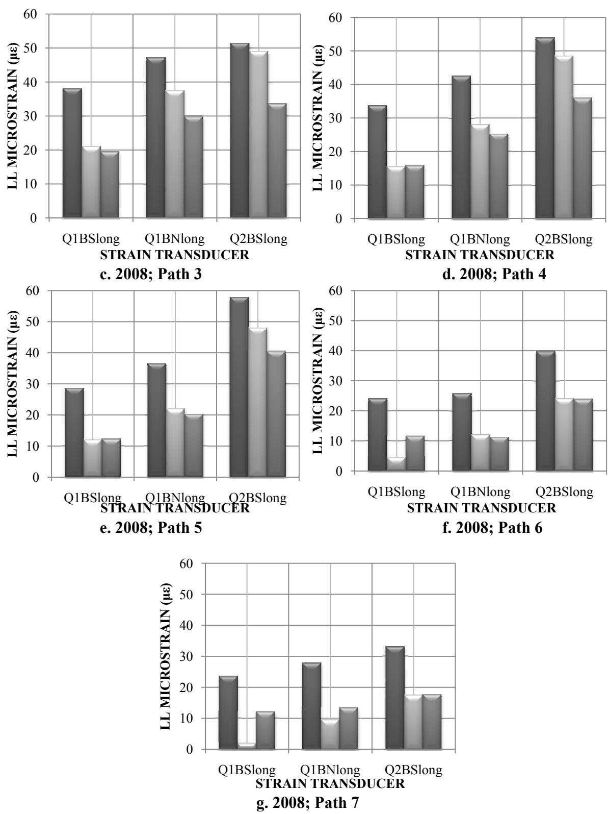
Figure 5.13-FEM LL Longitudinal Bulb Strain at Quarterspan Paths 1-7
